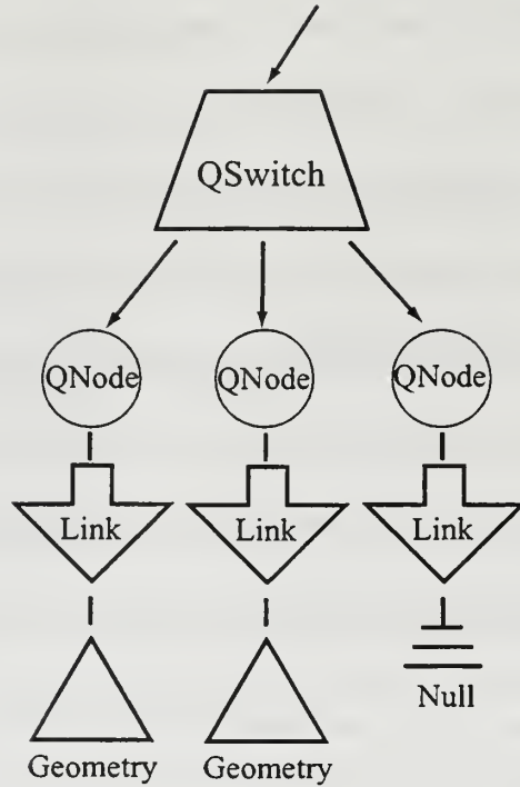
Figure 13. A legal QSwitch node has only QNode children, which each contain a single Link child.
