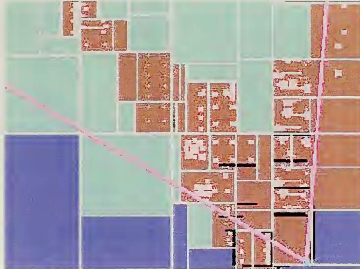
Figure 4. Dynamic visibility with the largest-occluder algorithm [Coorg and Teller, 1996].
