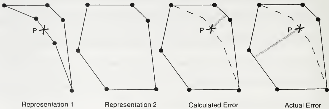
Figure 9. Error calculation using surface distances.
