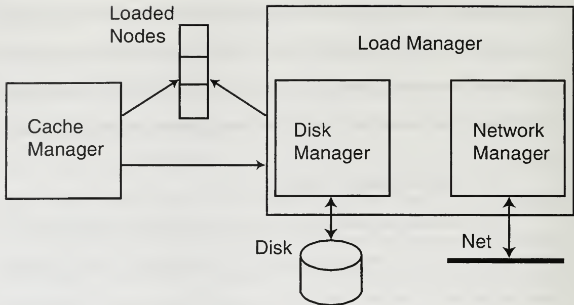
Figure 22. Cache management components.
