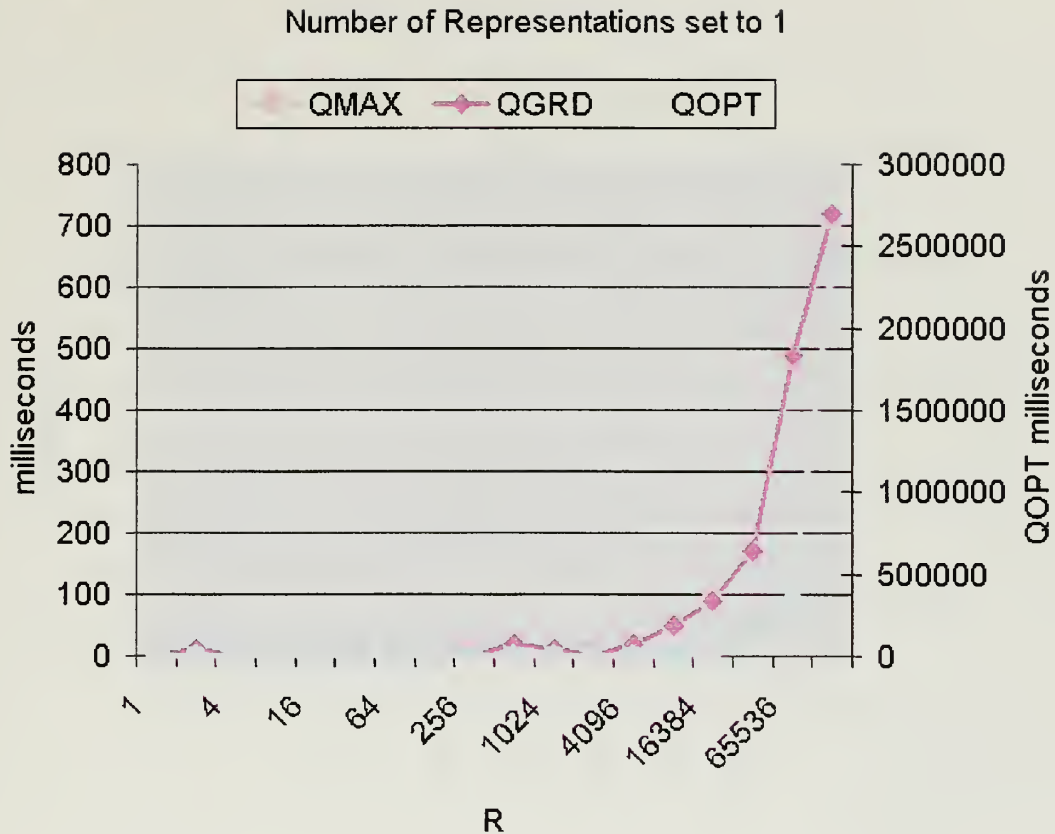
Figure 38. Running times compared with N=2^i and R=1 .
