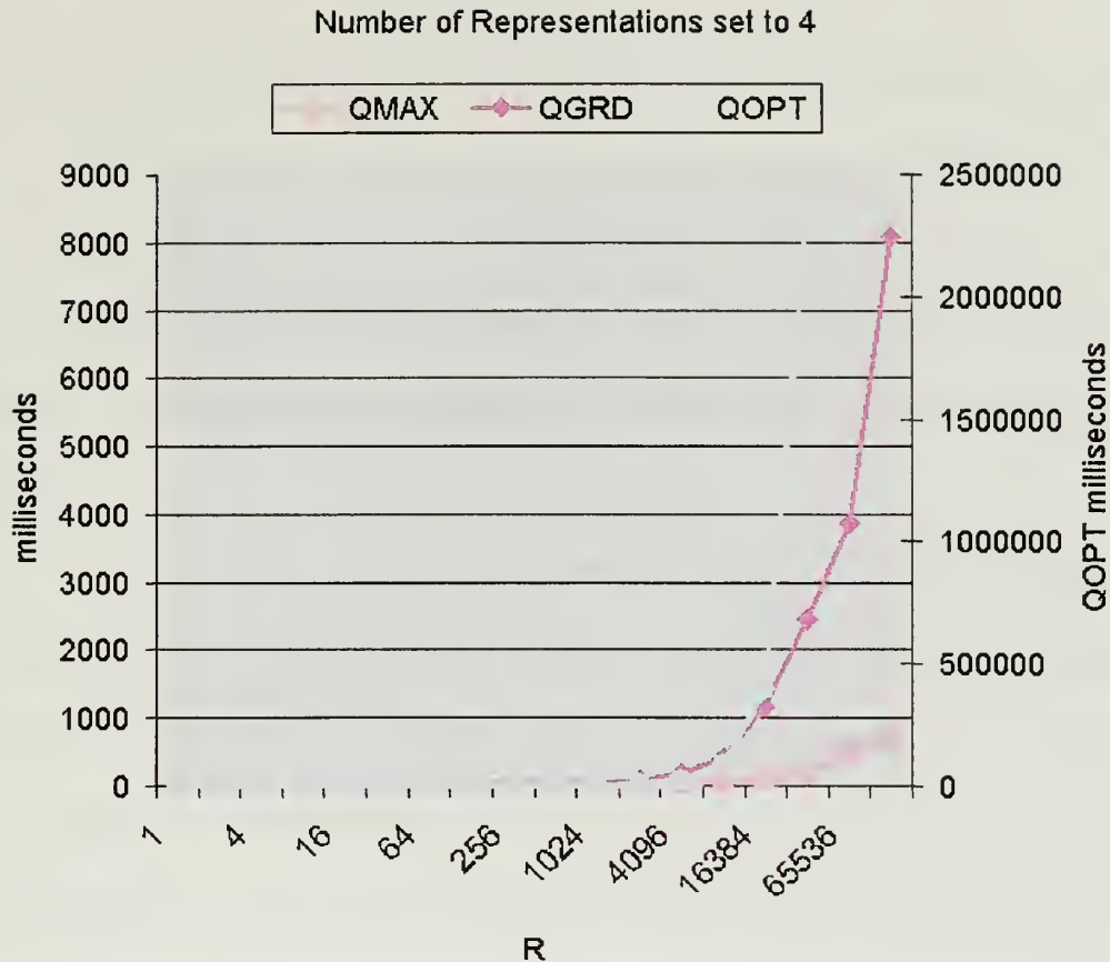
Figure 39. Running times compared with N=2^i and R=4 .
