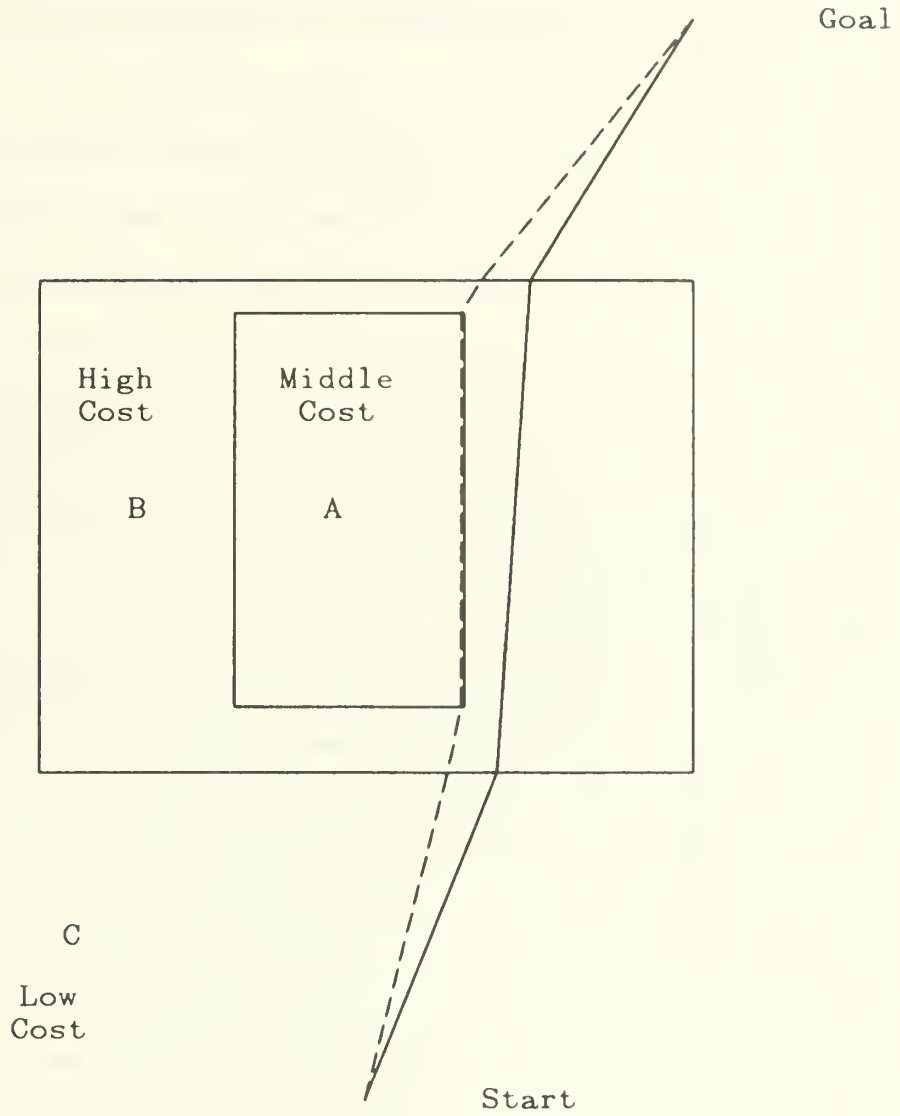
Figure 2 Locality Aspect of Snell's Law
