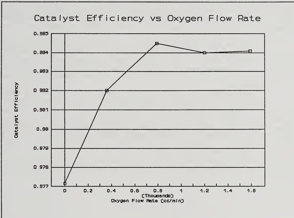
Figure 5-1: Supplemental Oxygen Effect on Catalyst Efficiency.
