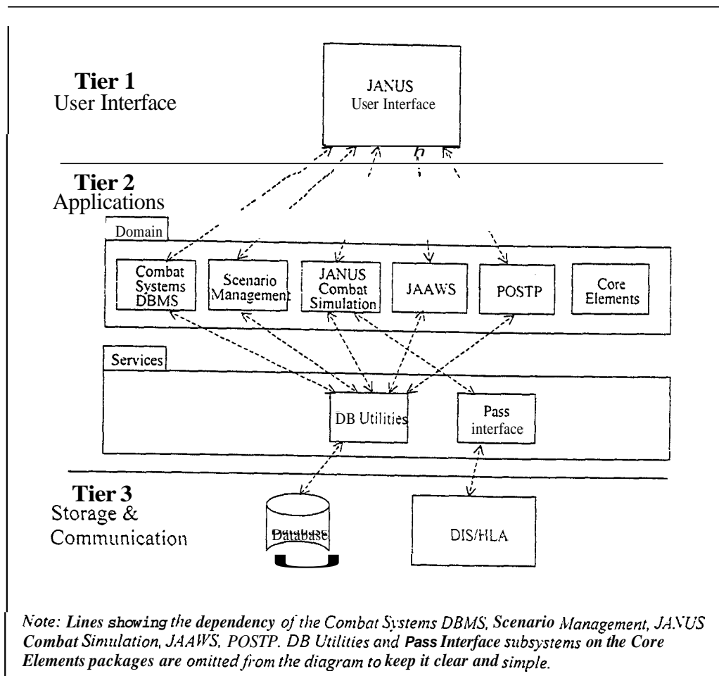
Figure 3. The proposed 3-tier object-oriented architecture.
