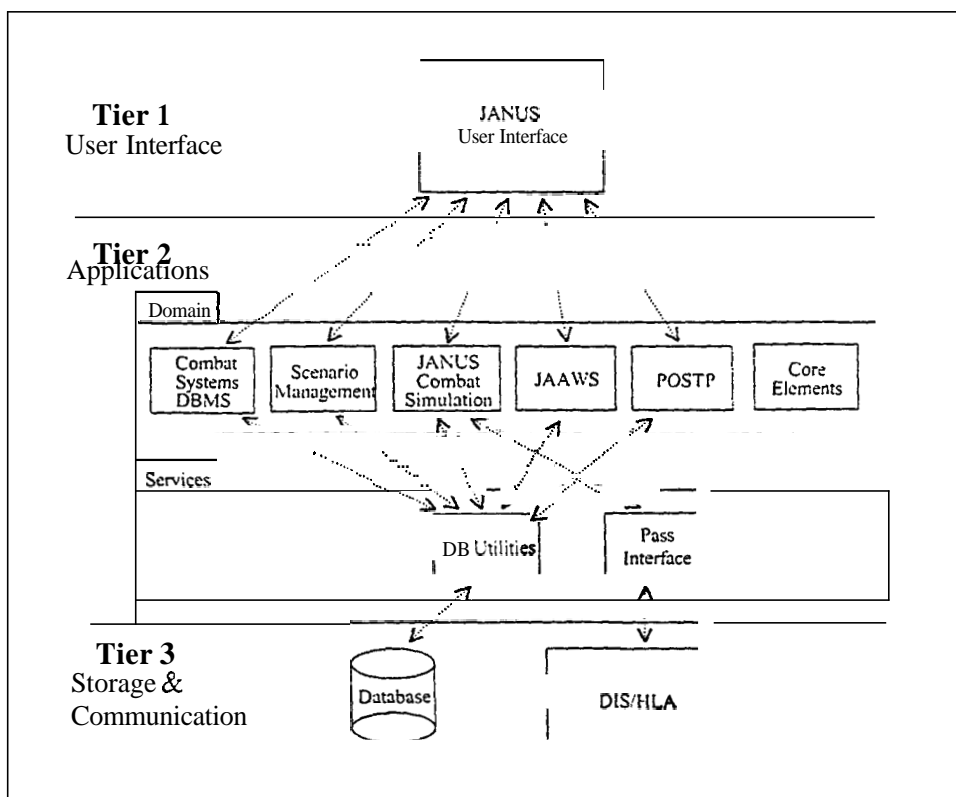
Figure 3. The proposed 3-tier object-oriented architecture
