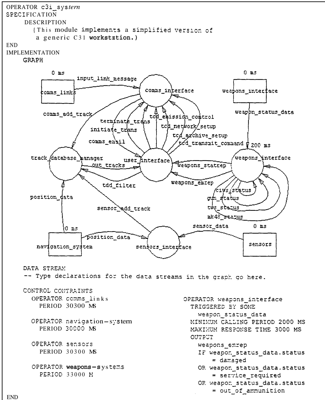
Figure 7. Top-level specification of the c3i_system
