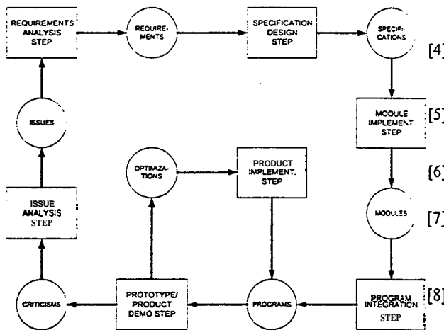
Figure 5: The evolutionary prototyping software process
