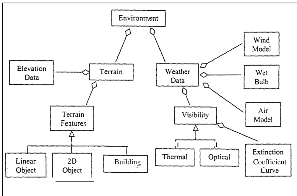
Figure 5. The Environment Object Class
