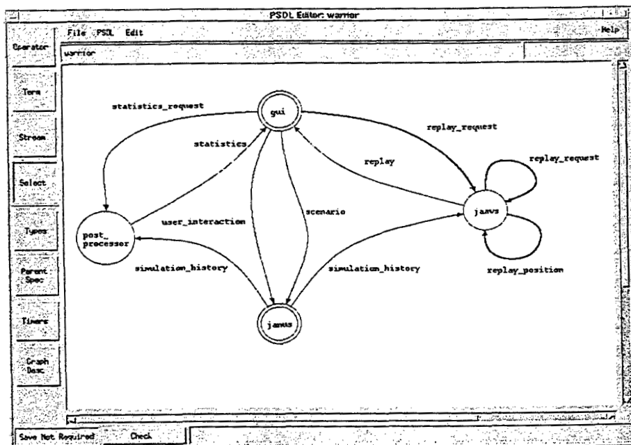
Figure 8. Top-level decomposition of the executable prototype.
