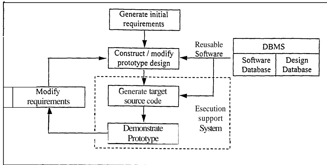
Figure 2. Iterative prototyping process in CAPS
