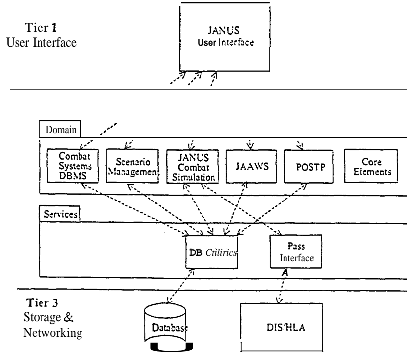
Figure 3. The proposed 3-tier object-oriented architecture.
