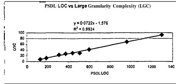
Figure 3: Correlation between PSDL and LGC
