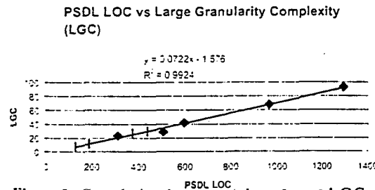
Figure 3: Correlation between Ada code and LGC
