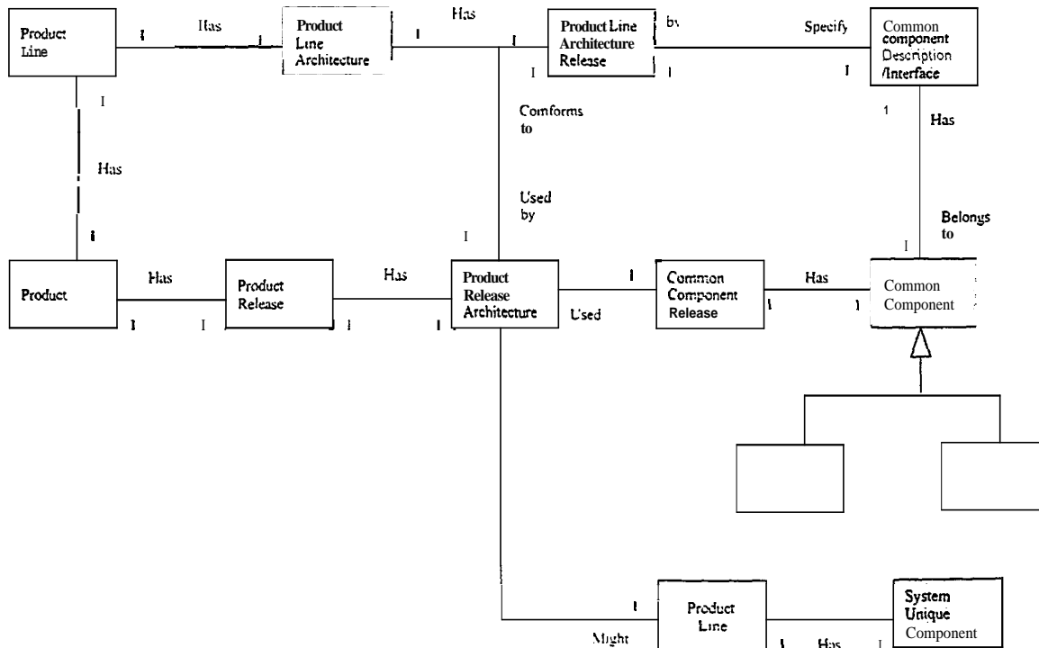
Figure I Product Line Views Model
