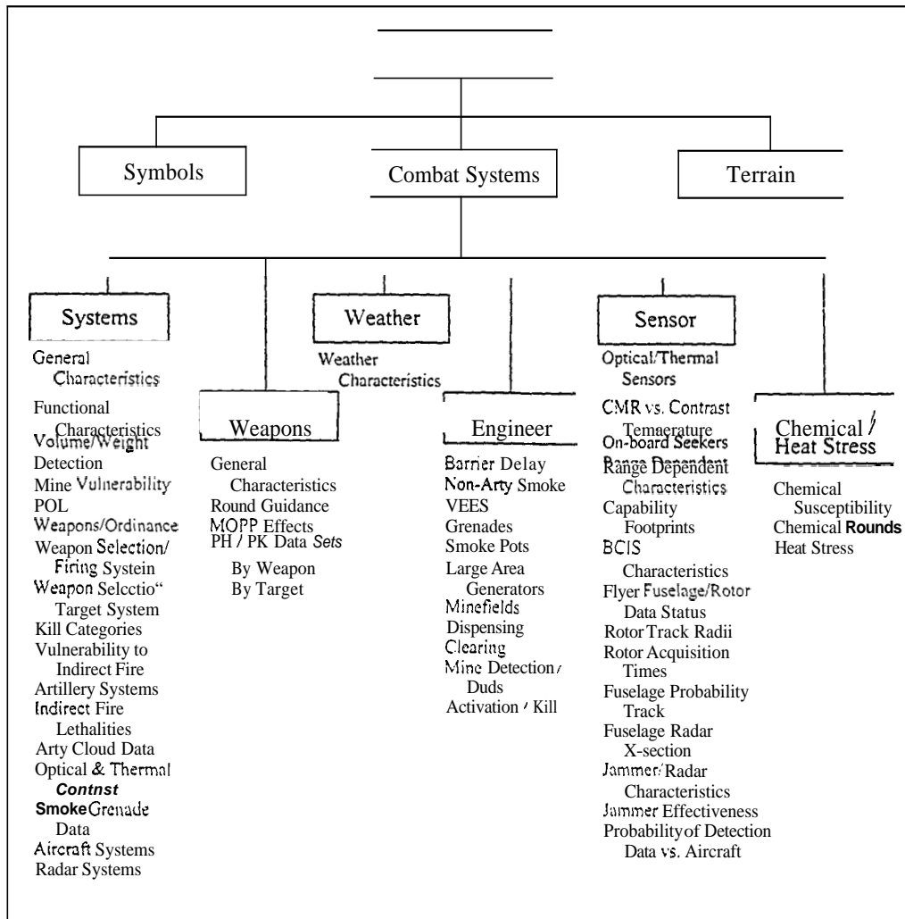
Figure 2. The top-level structure of the Janus Database
