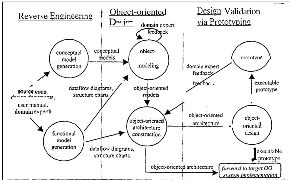
Figure 1. The object-oriented re-architecting process
