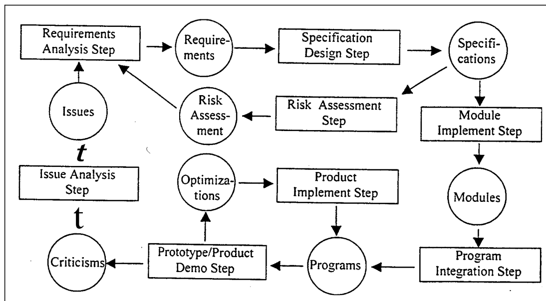
Figure 4. The improved evolutionary prototyping software process.
