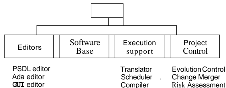
Figure 1. The CAPS rapid prototyping environment
