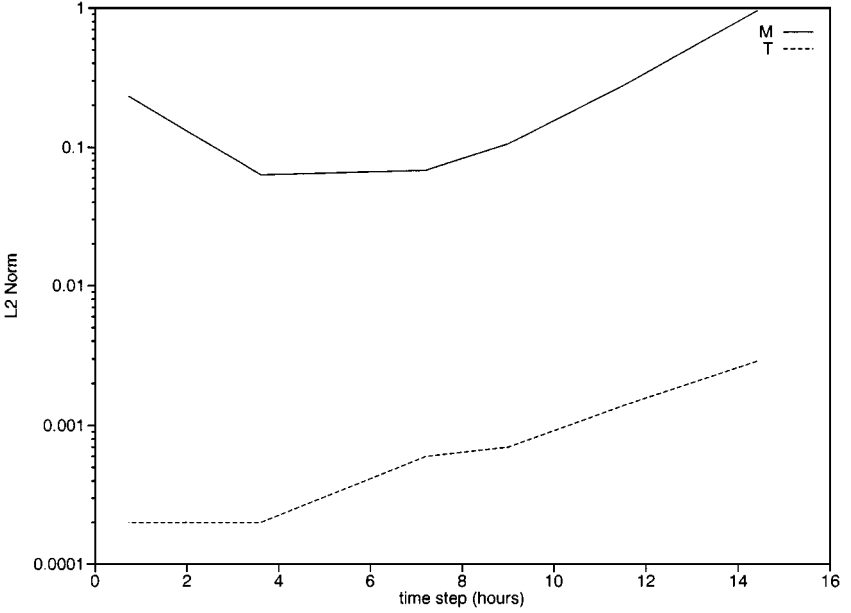
FIG. 5. Case 1. Time-step study of the mass (M) and trajectory (T) errors for the grid p = 16 .
