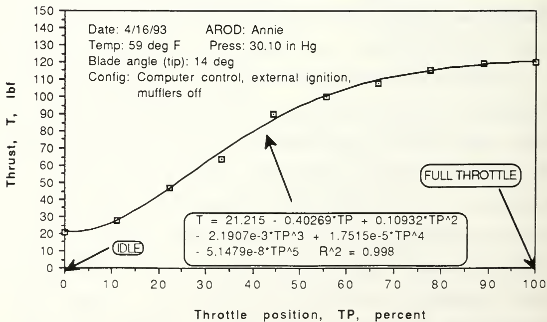
Figure IV.3: AROD Engine Modelling--Thrust Versus Throttle Position
