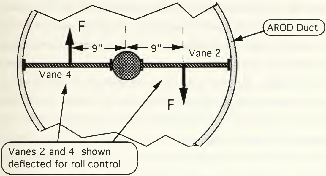
Figure IV.8: AROD Roll Control Functional Model
