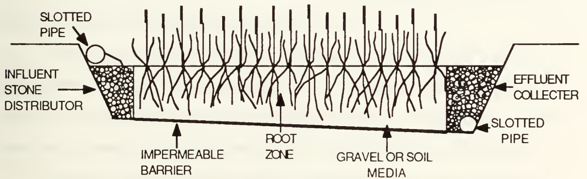
Figure II-2. Typical cross section SFCW (After EPA 1988).
