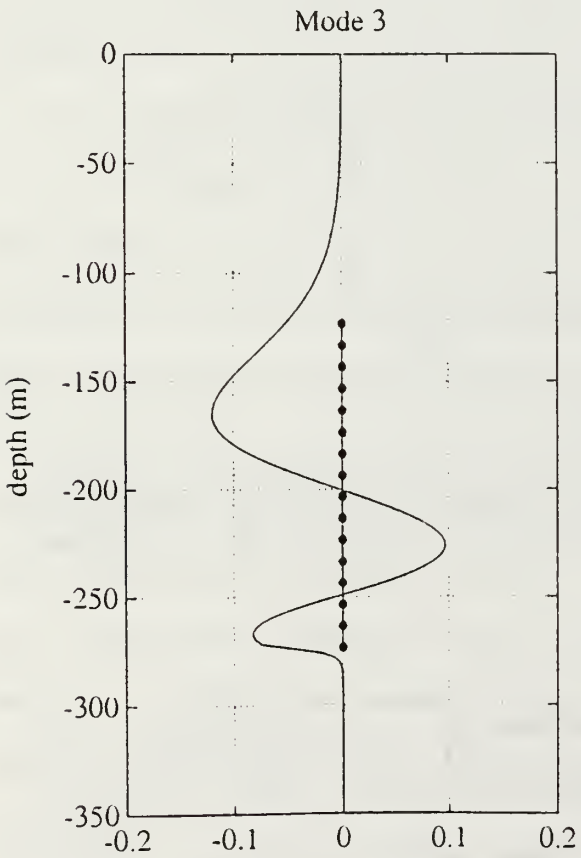
Figure 8 Normal modes 1 through 4.
