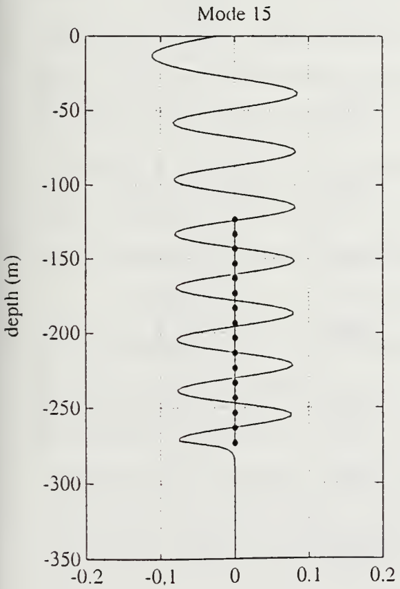
Figure 11 Normal modes 13 through 16.
