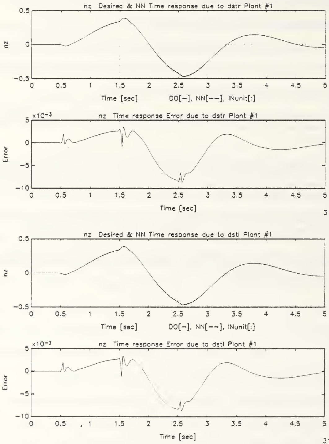
Figure 8.4: Normal Acceleration Response of the Undamaged Aircraft Due to Dipole Command in the Stabilators
