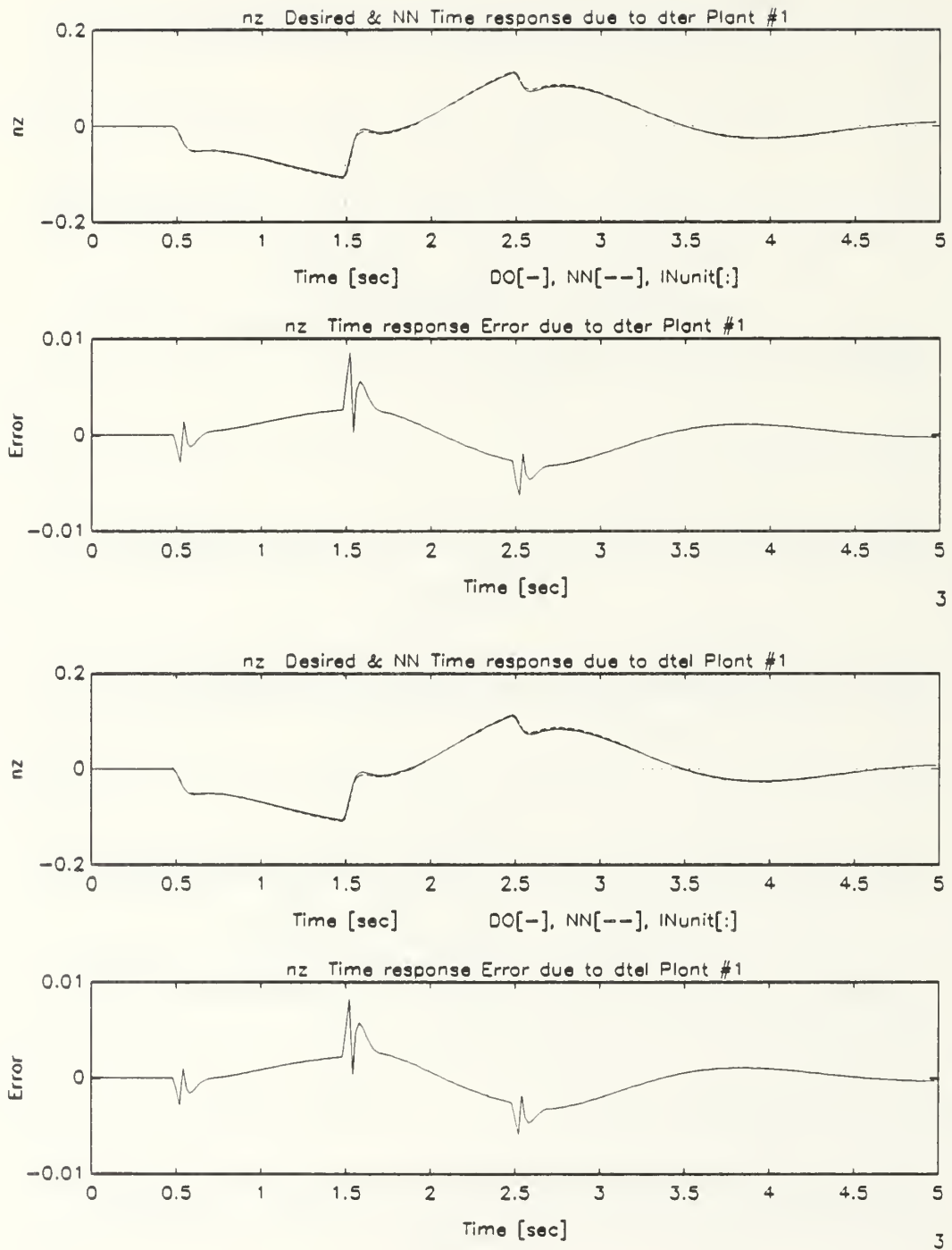
Figure B.29: Normal Acceleration Response of Undamaged Aircraft Due to Trailing Edge Flaps Dipole Command, Multiple-Plant, Single Network Emulation
