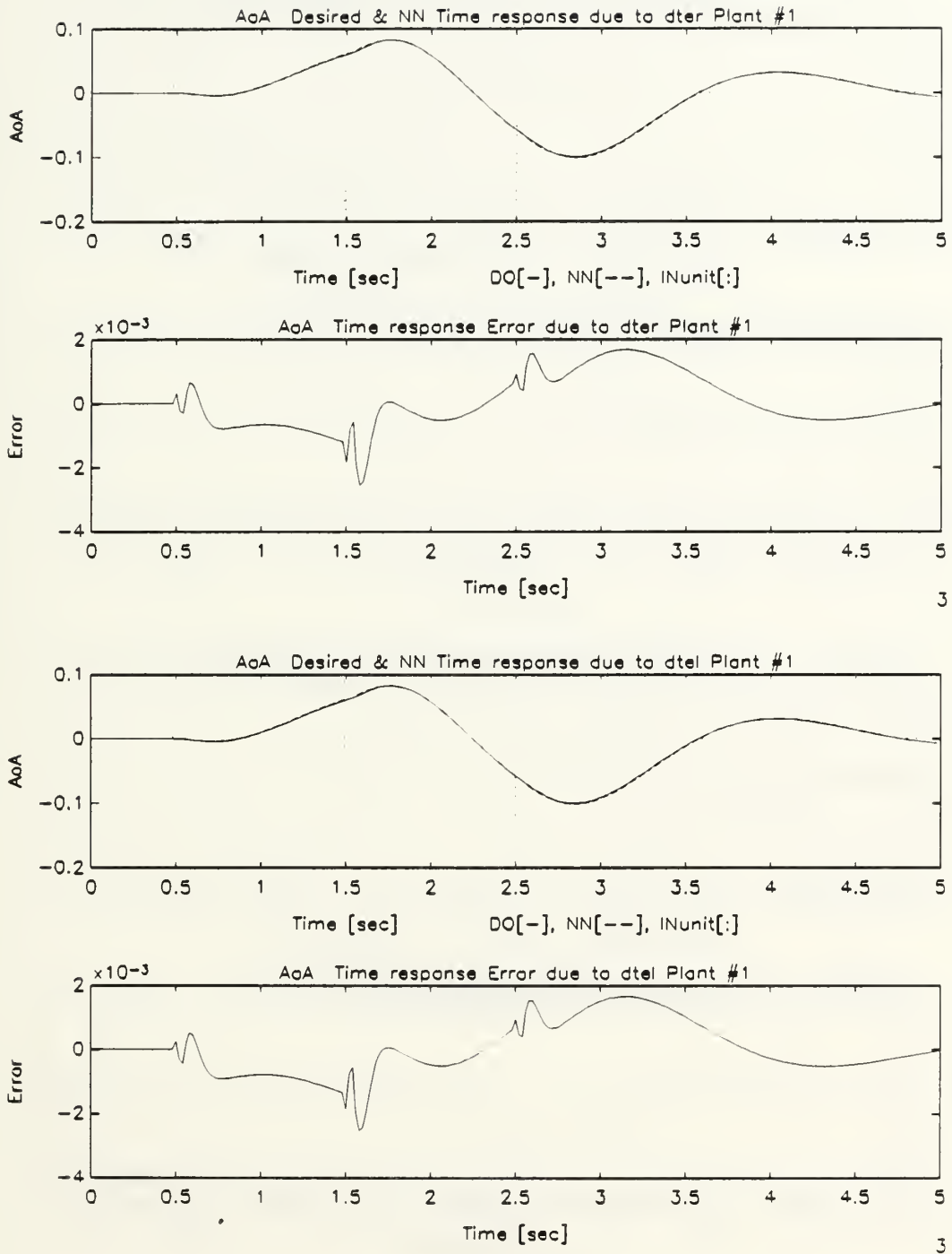
Figure B.32: Angle of Attack Response of Undamaged Aircraft Due to Trailing Edge Flaps Dipole Command, Multiple-Plant, Single Network Emulation
