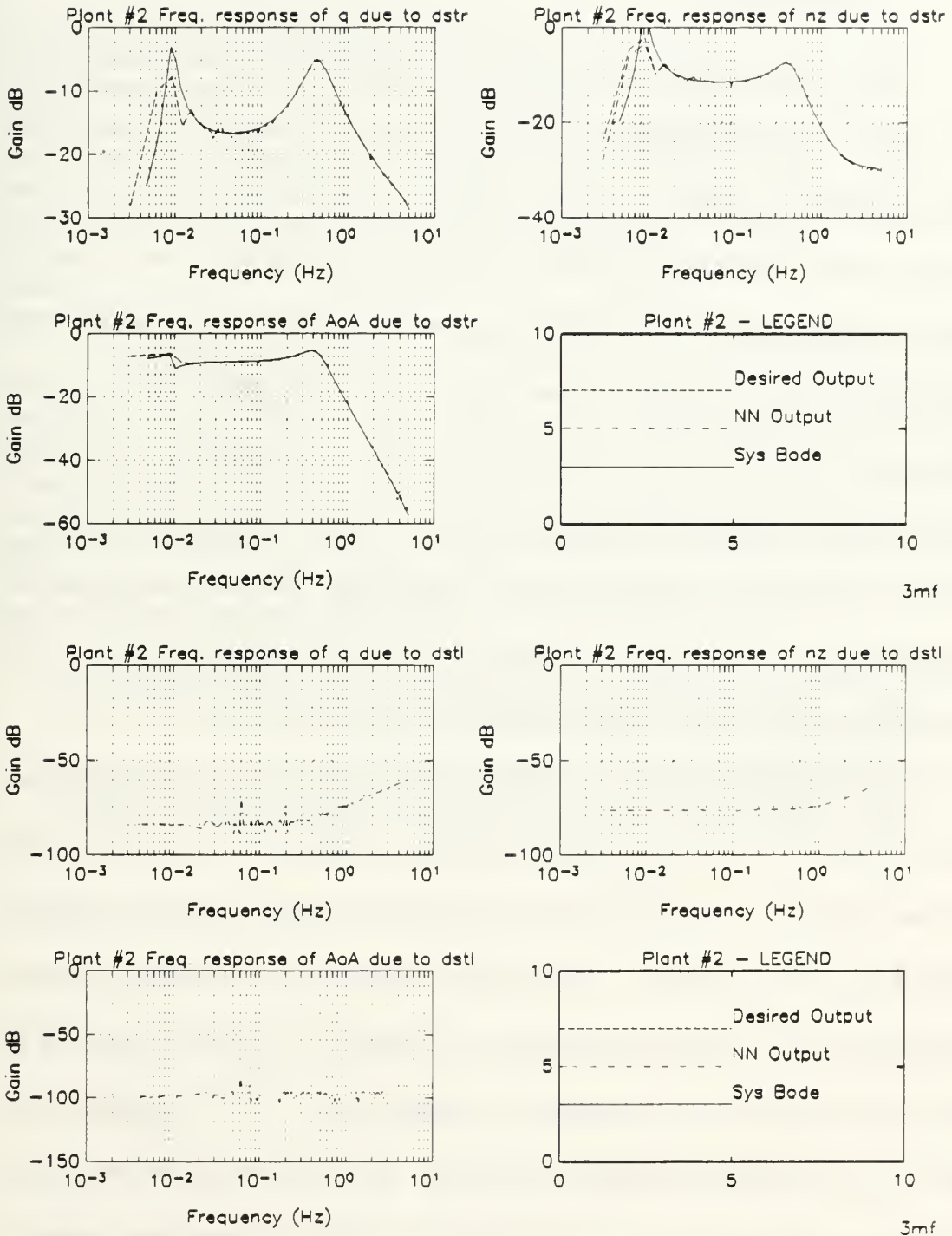
Figure 8.15: Spectral Response of Damaged Aircraft Due to Stabilators in a Minimally Realized Multiple-Plant Single Network Emulator
