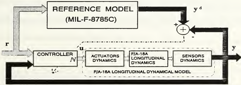
Figure 7.2: Model-Reference Control Architecture for the F/A-18A
