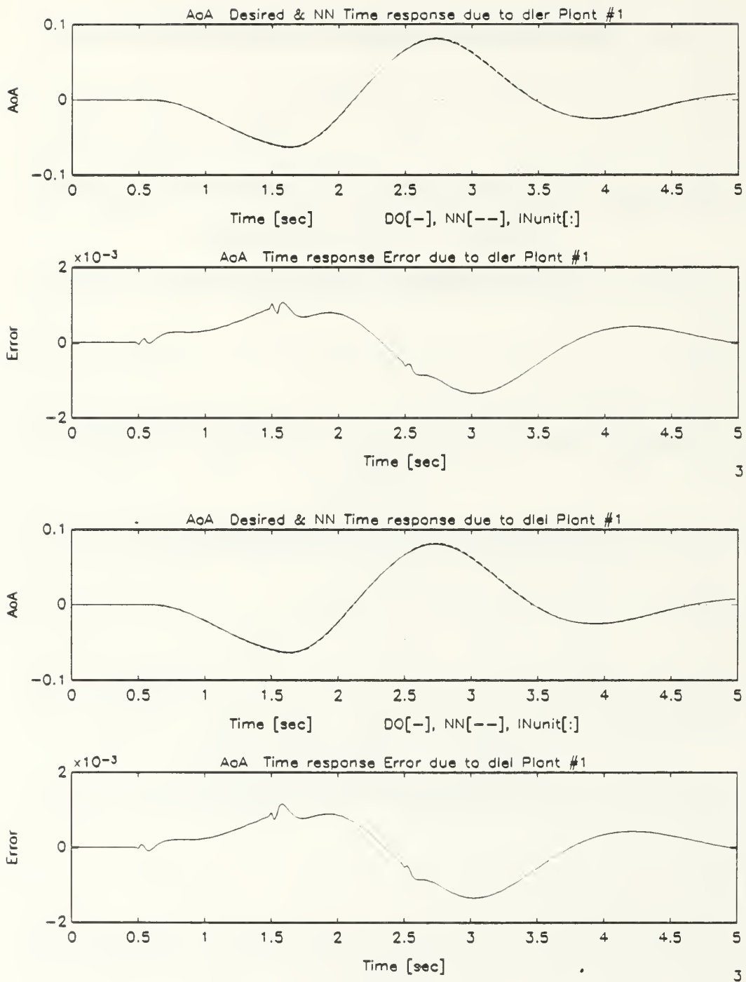
Figure B.31: Angle of Attack Response of Undamaged Aircraft Due to Leading Edge Flaps Dipole Command, Multiple-Plant, Single Network Emulation
