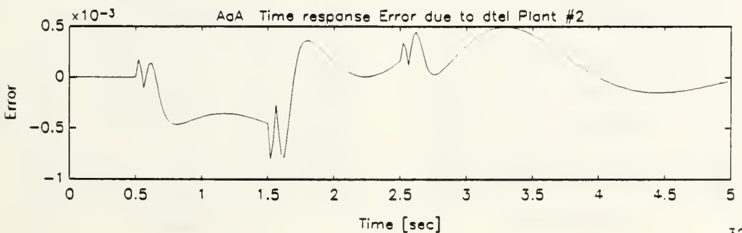
Figure B.20: Angle of Attack Response of Damaged Aircraft Due to Trailing Edge Flaps Dipole Command, Single Plant, Single Network Emulation
