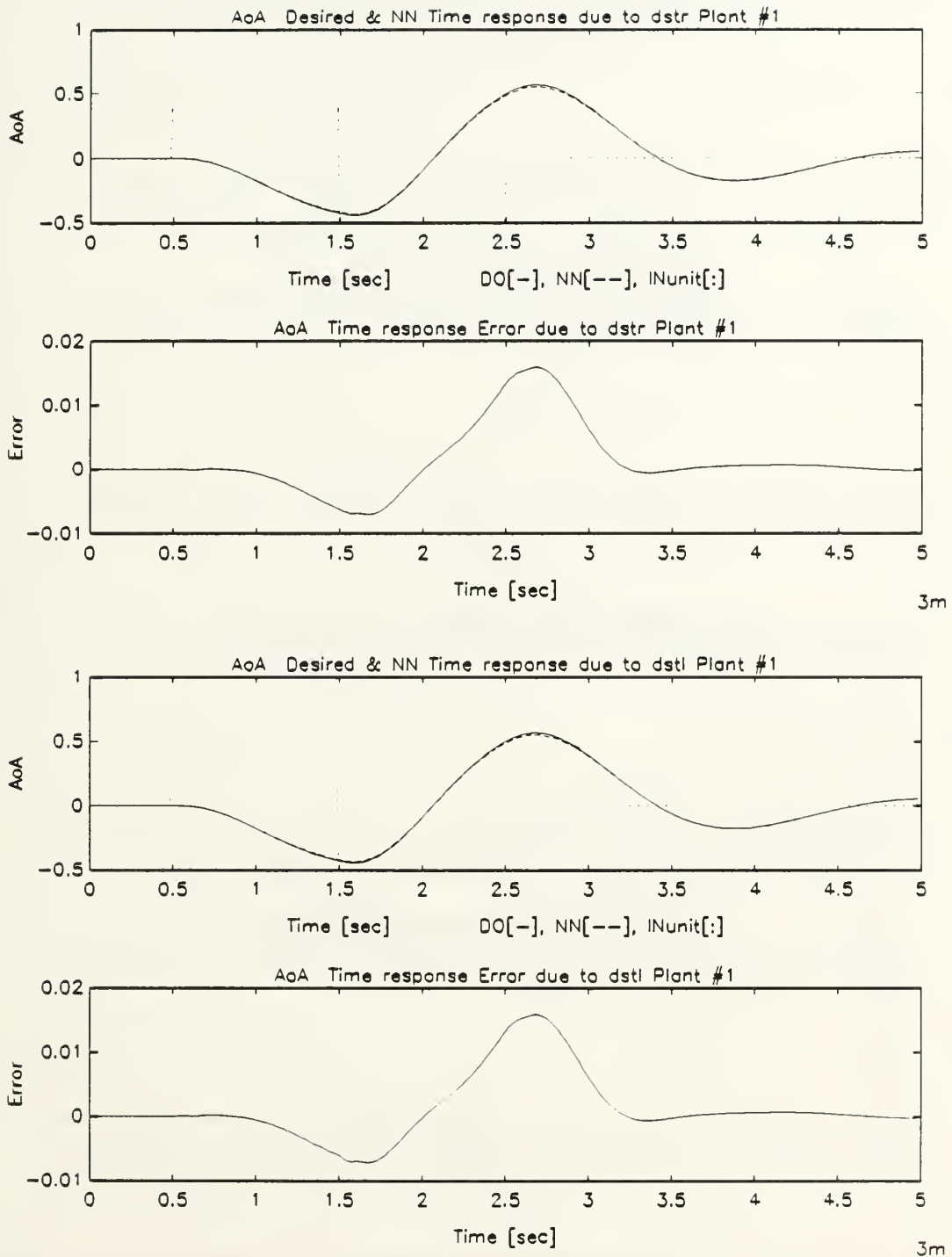
Figure B.52: Angle of Attack Response of Undamaged Aircraft Due to Stabilators Dipole Command, Multiple-Plant, Minimized Network Emulation
