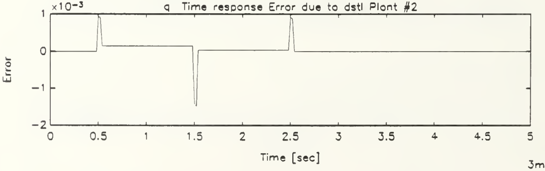
Figure B.55: Pitch Rate Response of Damaged Aircraft Due to Stabilizers Dipole Command, Multiple-Plant, Minimized Network Emulation
