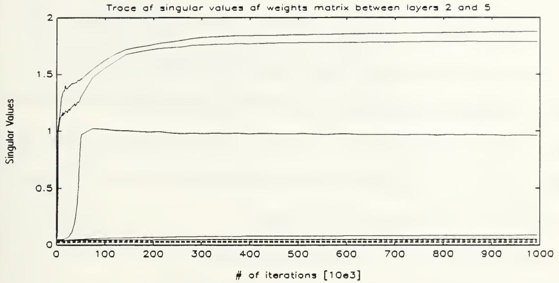
Figure C.5: Singular Values Plot of Weight Matrix from OutReg to outh1 , Before Minimization
