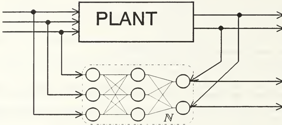
Figure 4.1: A Neural Network Emulation of Dynamical System
