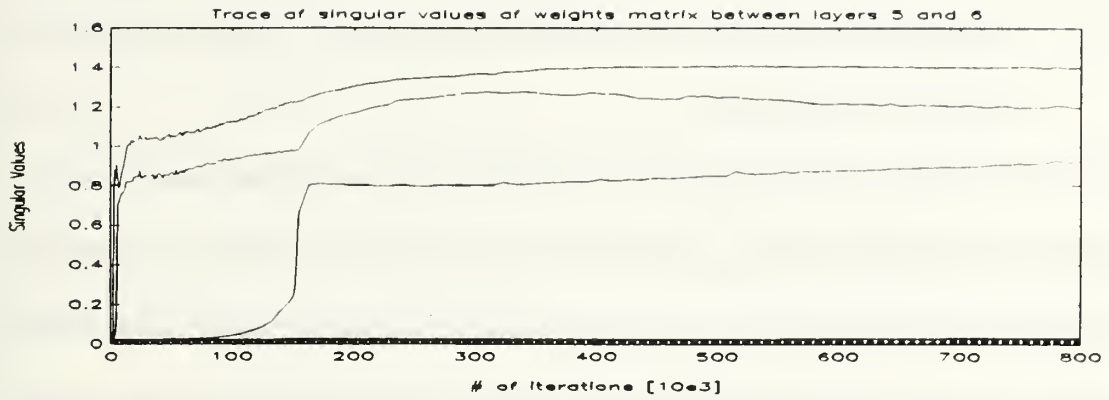
Figure 8.12: Singular Values Plot of the Minimized Network
