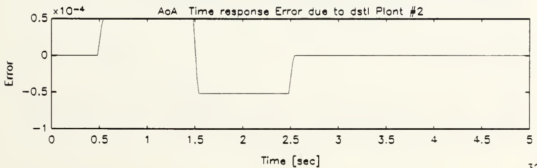
Figure B.18: Angle of Attack Response of Damaged Aircraft Due to Stabilators Dipole Command, Single Plant, Single Network Emulation
