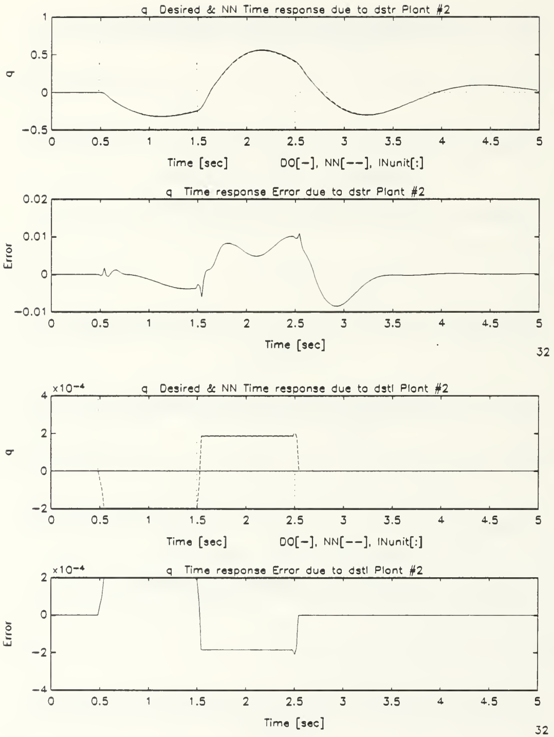
Figure B.13: Pitch Rate Response of Damaged Aircraft Due to Stabilizers Dipole Command, Single Plant, Single Network Emulation
