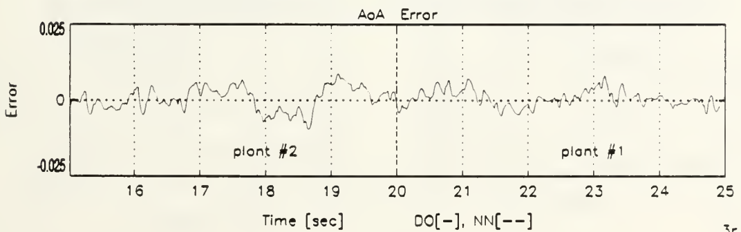
Figure B.42: Angle of Attack Response to RBS Excitation of All Inputs, Multiple-Plant, Single Network Emulation
