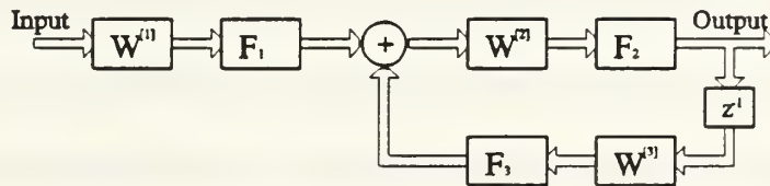
Figure 2.6: General Multi-Layer Building Block
