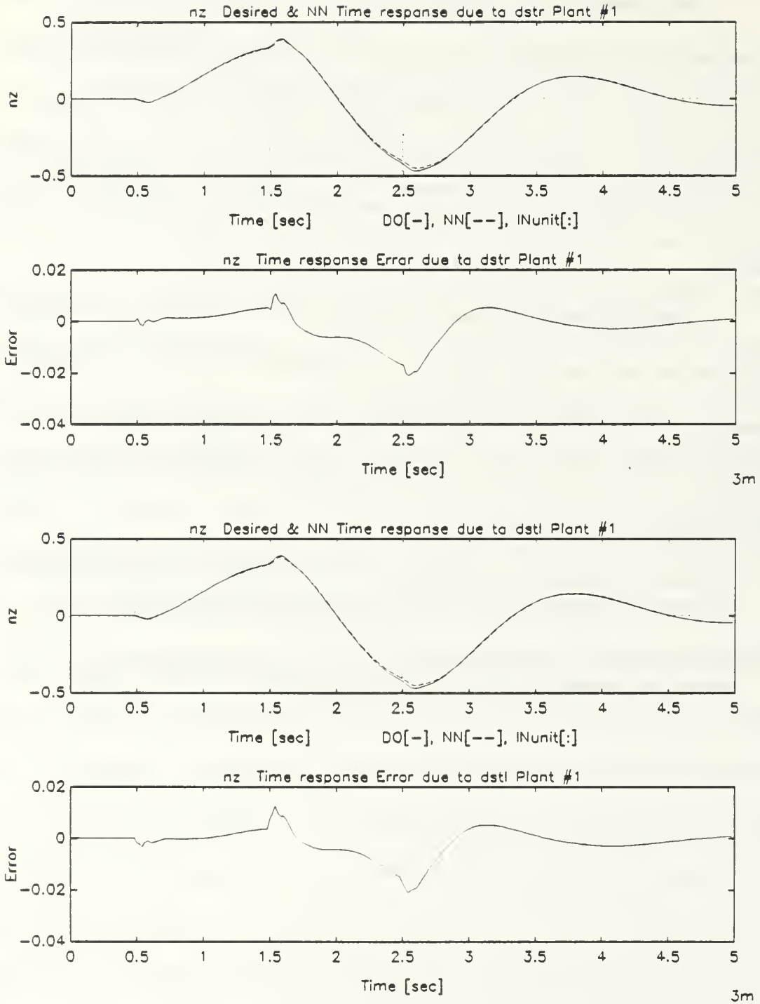
Figure 8.16: Normal Acceleration Response of the Undamaged Aircraft Due to Dipole Stabilators Command in a Minimized Multiple-Plant Network
