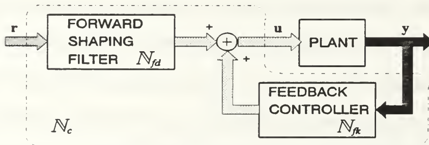
Figure 5.7: Control Architecture
