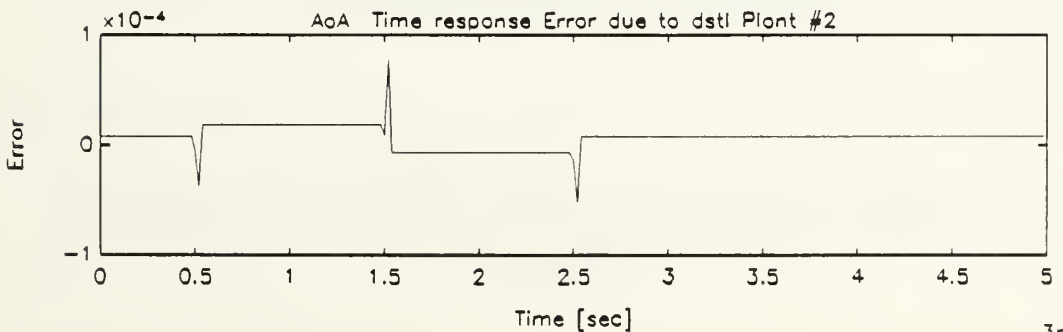
Figure B.60: Angle of Attack Response of Damaged Aircraft Due to Stabilators Dipole Command, Multiple-Plant, Minimized Network Emulation
