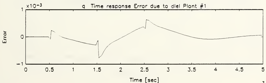
Figure B.6: Pitch Rate Response of Undamaged Aircraft Due to Leading Edge Flaps Dipole Command, Single Plant, Single Network Emulation
