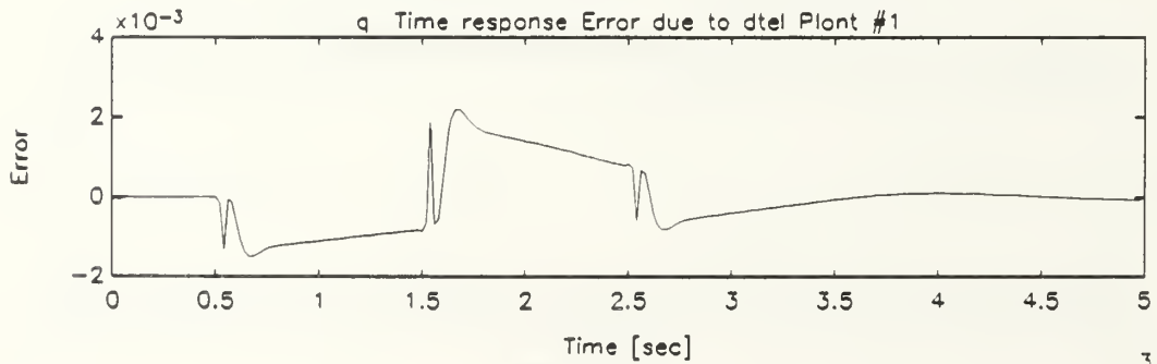
Figure B.7: Pitch Rate Response of Undamaged Aircraft Due to Trailing Edge Flaps Dipole Command, Single Plant, Single Network Emulation
