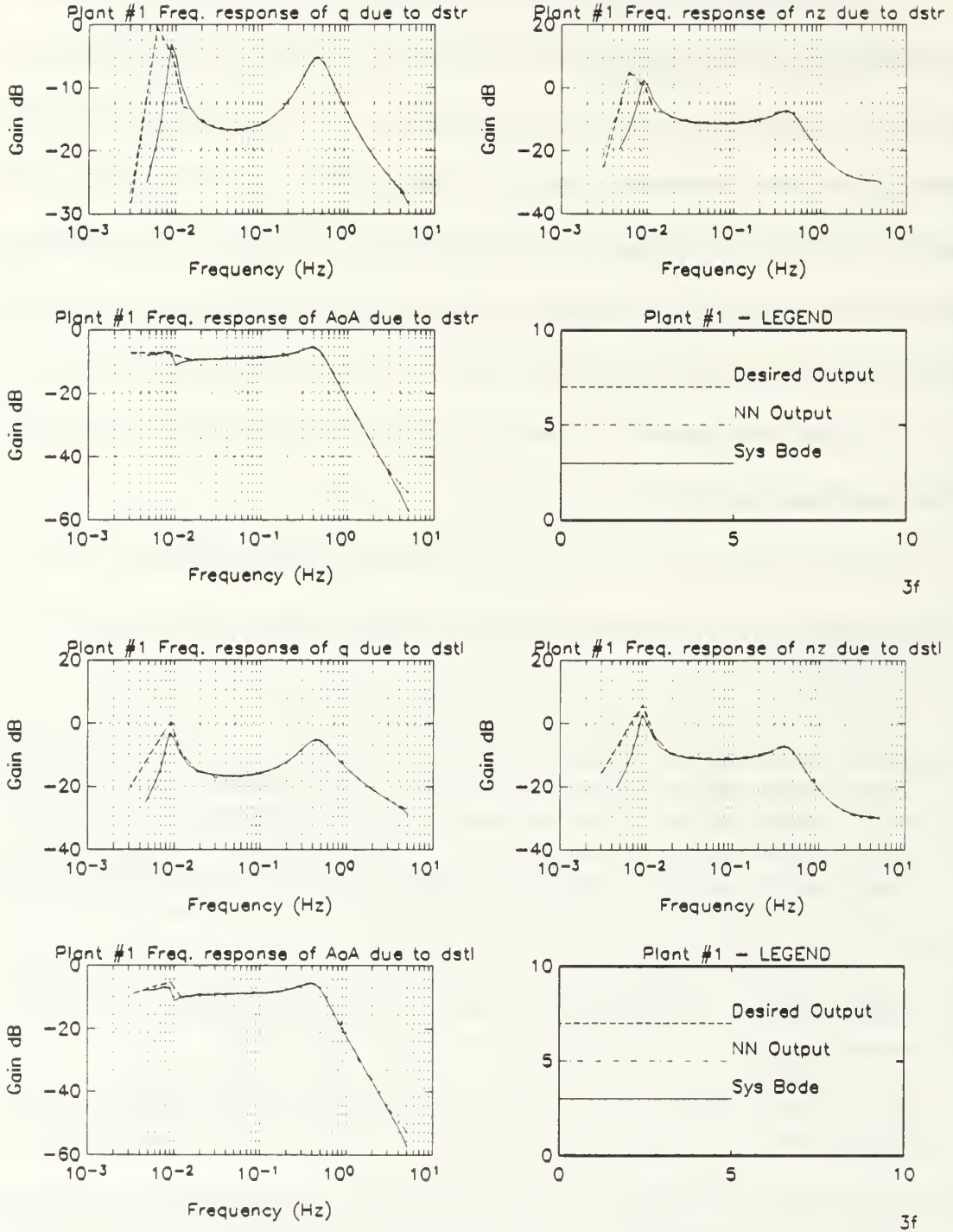
Figure 8.6: Spectral Response of Undamaged Aircraft Due to Stabilators in a Multiple-Plant Single Network Emulation
