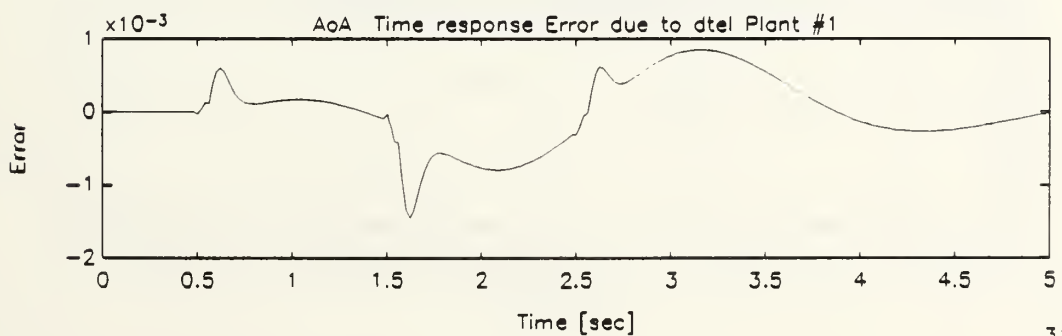
Figure B.12: Angle of Attack Response of Undamaged Aircraft Due to Trailing Edge Flaps Dipole Command, Single Plant, Single Network Emulation
