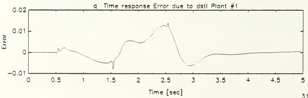
Figure B.5: Pitch Rate Response of Undamaged Aircraft Due to Stabilators Dipole Command, Single Plant, Single Network Emulation
