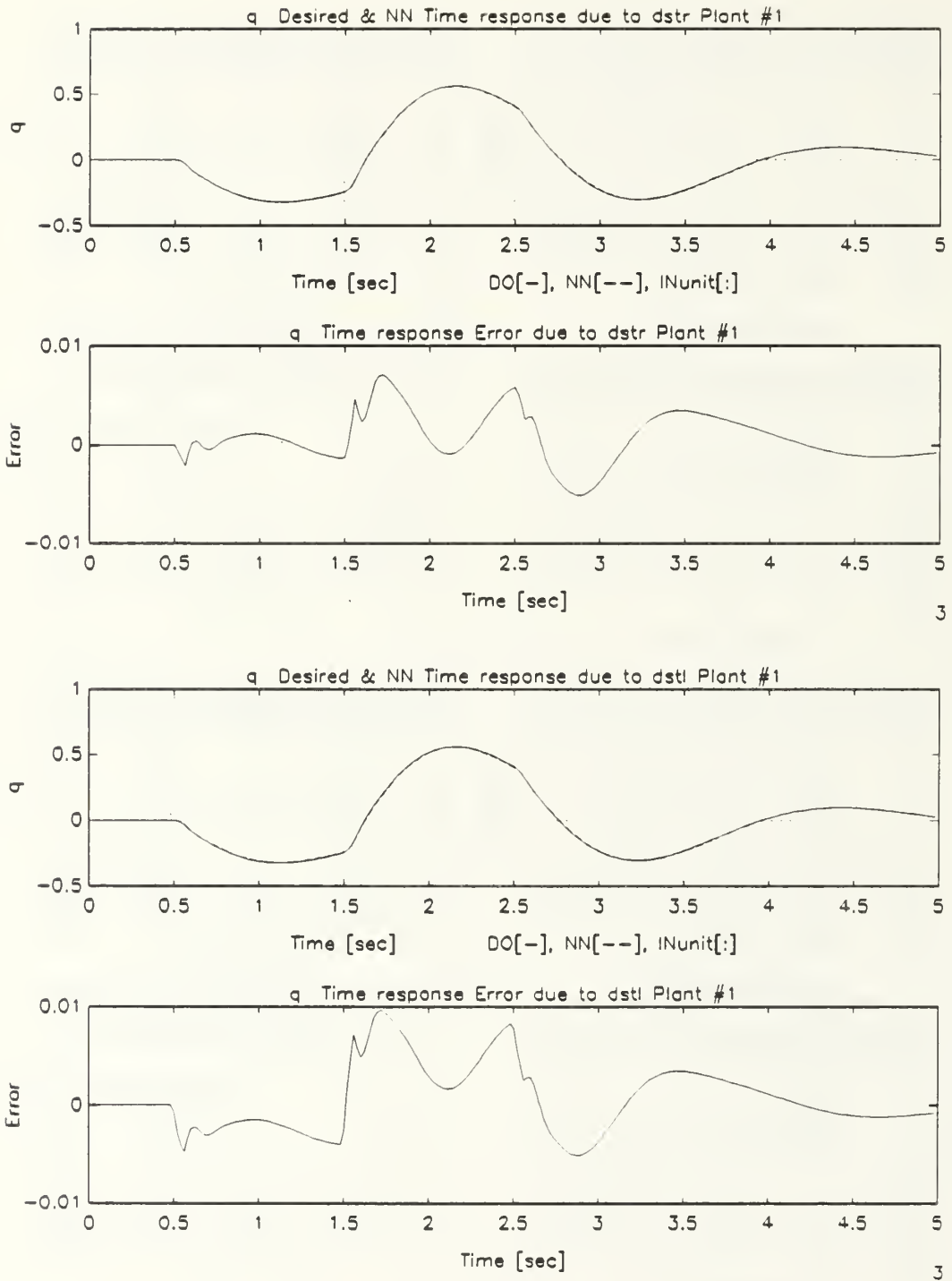
Figure B.25: Pitch Rate Response of Undamaged Aircraft Due to Stabilators Dipole Command, Multiple-Plant, Single Network Emulation
