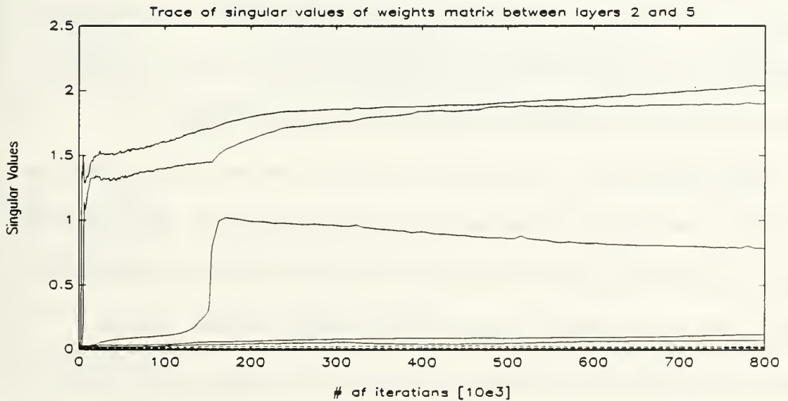
Figure C.6: Singular Values Plot of Weight Matrix from OutReg to outh1 , After Minimization
