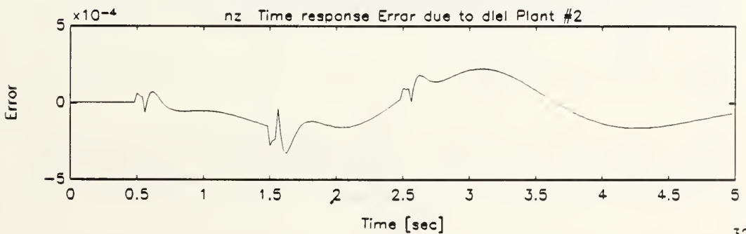
Figure B.16: Normal Acceleration Response of Damaged Aircraft Due to Leading Edge Flaps Dipole Command, Single Plant, Single Network Emulation
