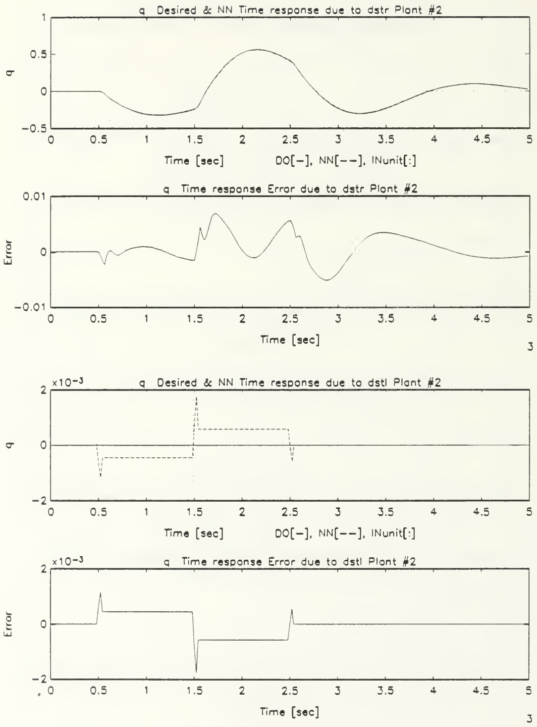
Figure B.33: Pitch Rate Response of Damaged Aircraft Due to Stabilators Dipole Command, Multiple-Plant, Single Network Emulation
