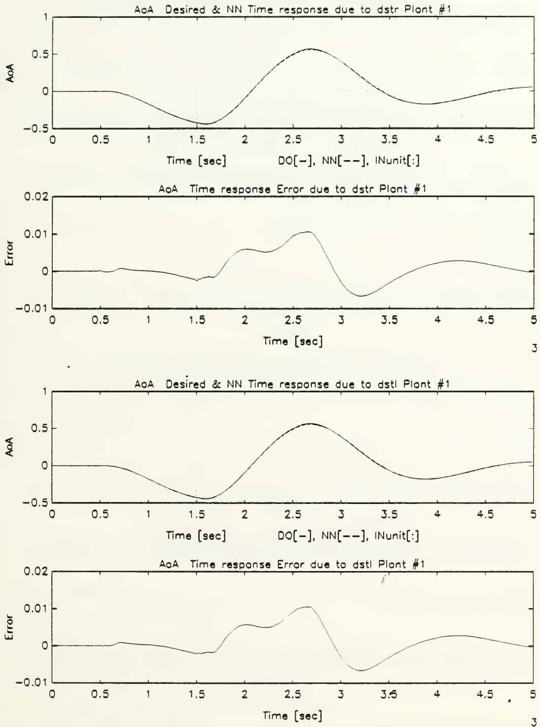
Figure B.30: Angle of Attack Response of Undamaged Aircraft Due to Stabilators Dipole Command, Multiple-Plant, Single Network Emulation
