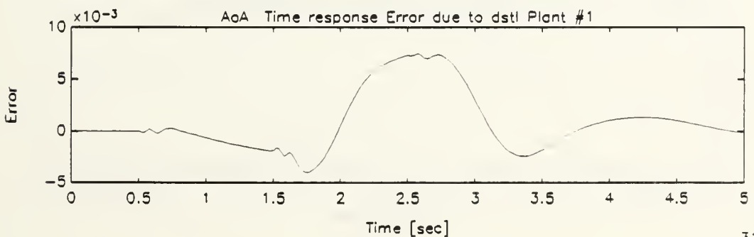
Figure B.10: Angle of Attack Response of Undamaged Aircraft Due to Stabilators, Dipole Command, Single Plant, Single Network Emulation
