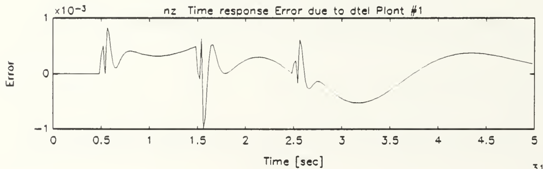
Figure B.9: Normal Acceleration Response of Undamaged Aircraft Due to Trailing Edge Flaps Dipole Command, Single Plant, Single Network Emulation
