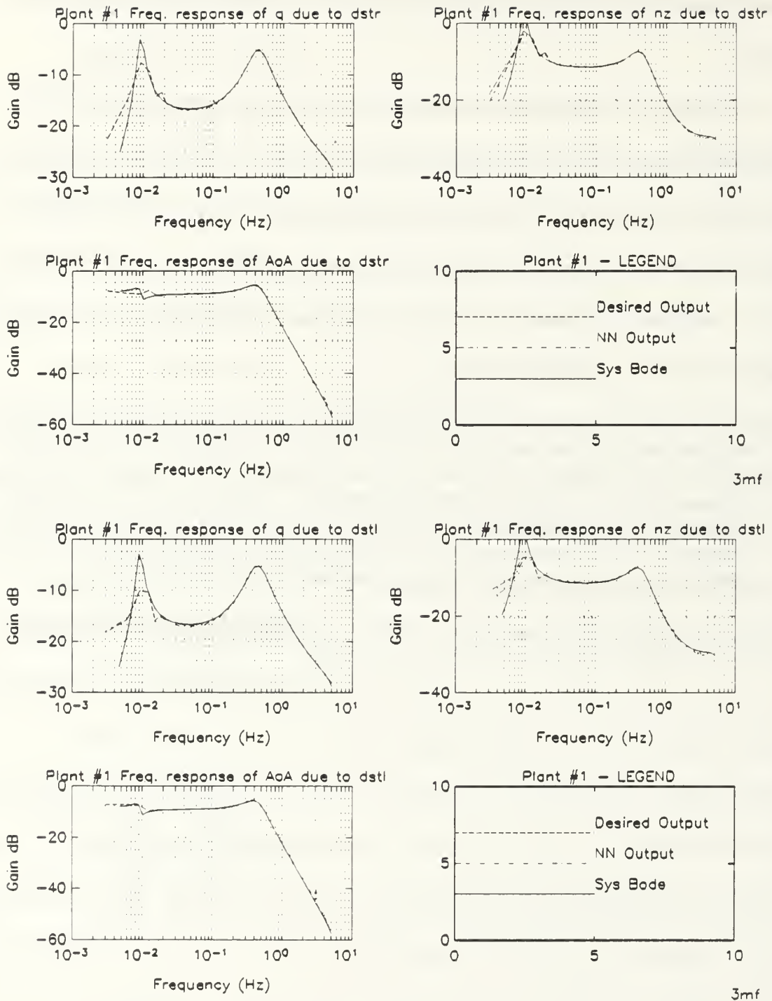
Figure 8.14: Spectral Response of Undamaged Aircraft Due to Stabilizers in a Minimally Realized Multiple-Plant Single Network Emulator
