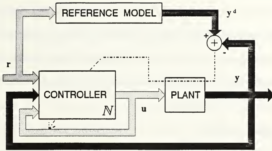
Figure 5.6: Direct Model-Reference Adaptive Control
