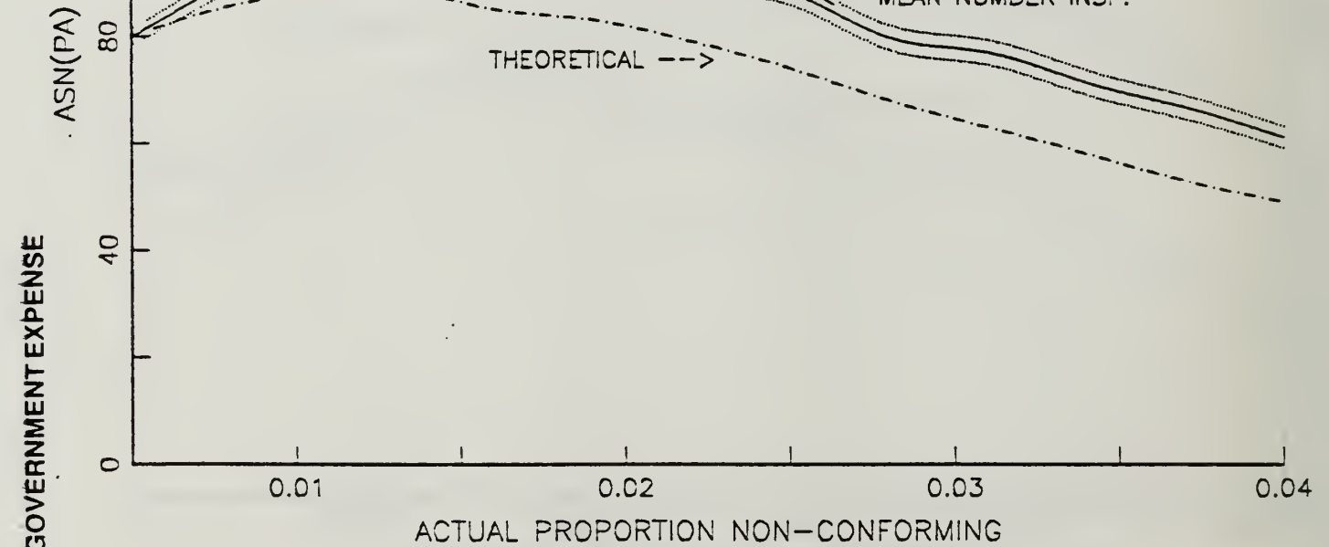
Figure 23 - ASN CURVE , PLAN SET I , CURVE D
