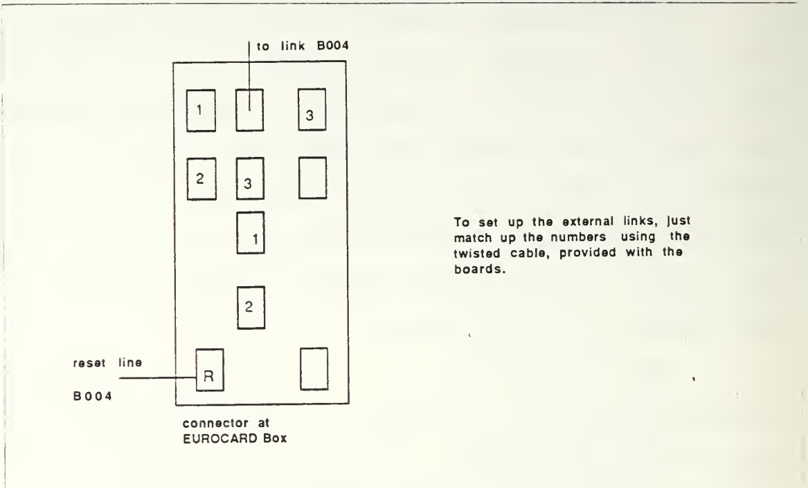
Figure 3.9 01 and 04 Transputer Networks Connections
