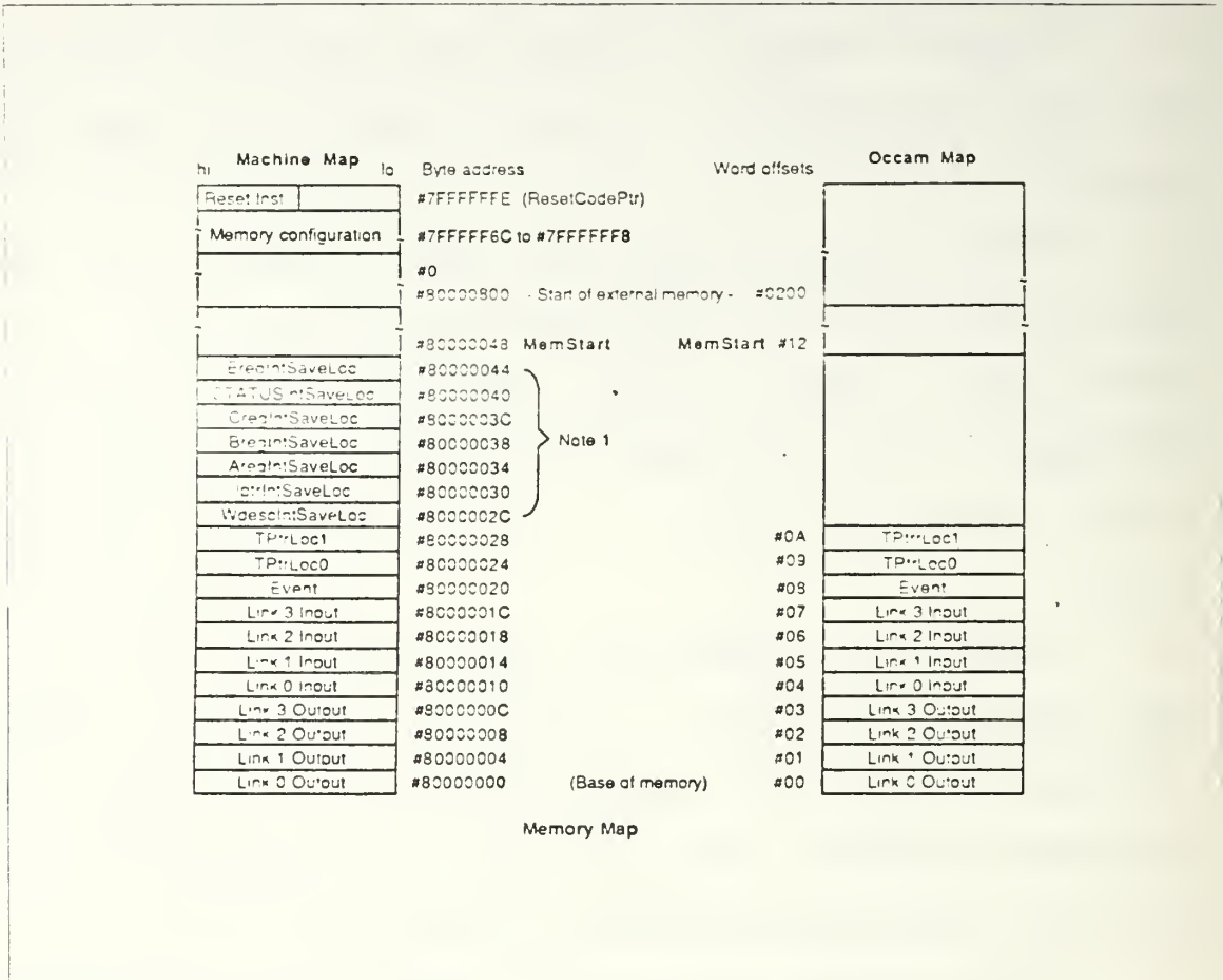
Figure 2.4 Memory Map
