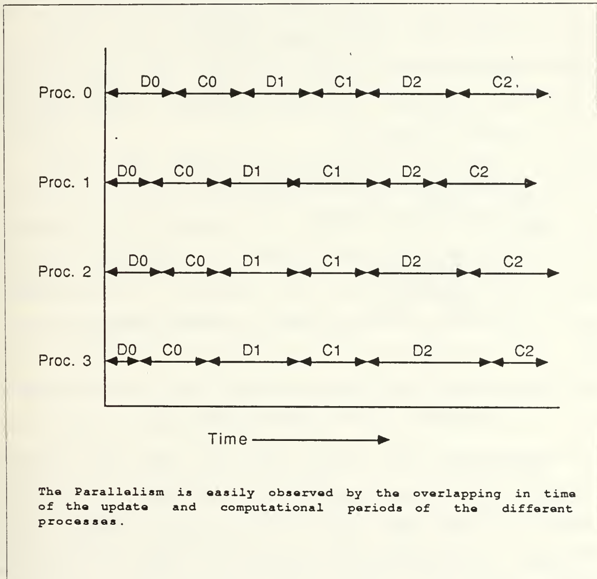
Figure 5.7 Timing Diagram
