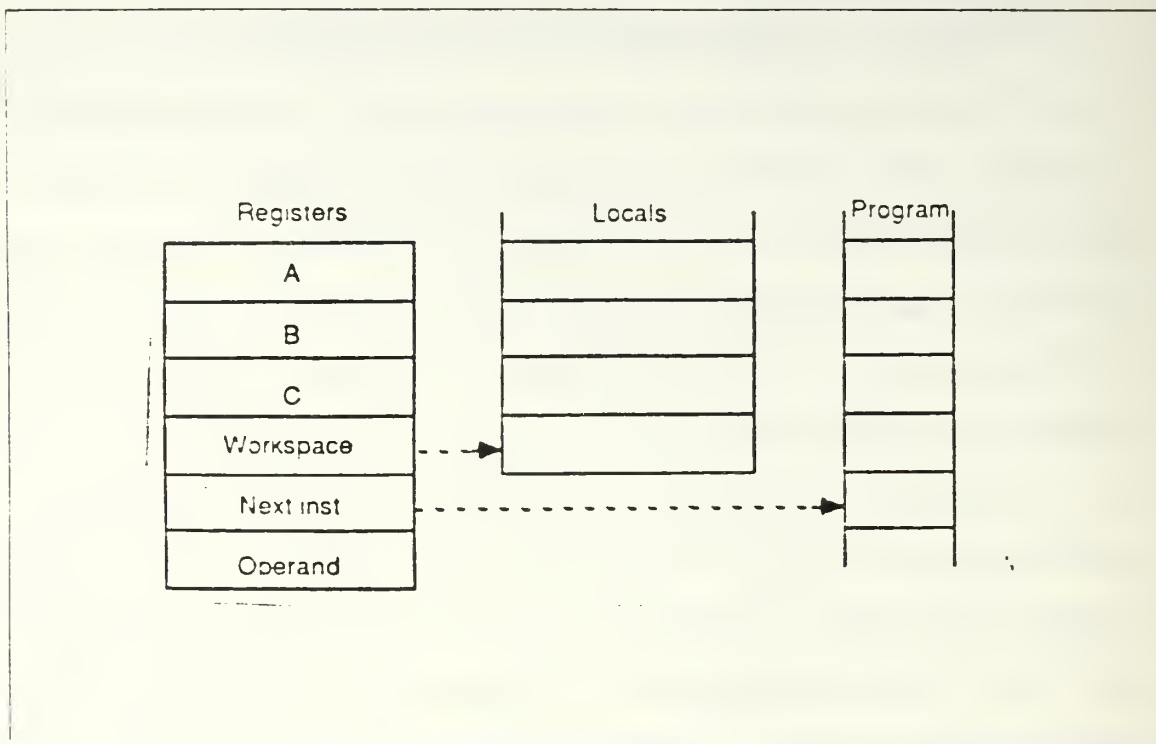
Figure 2.2 Transputer Registers
