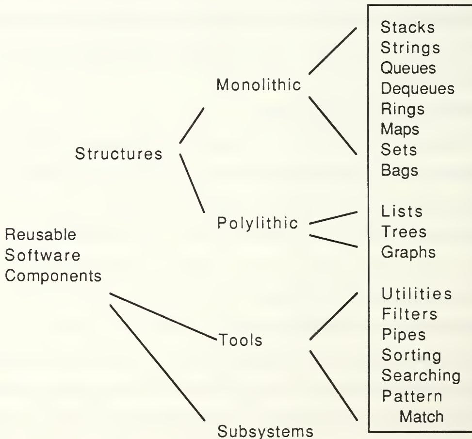
Figure 3. Booch Taxonomy
