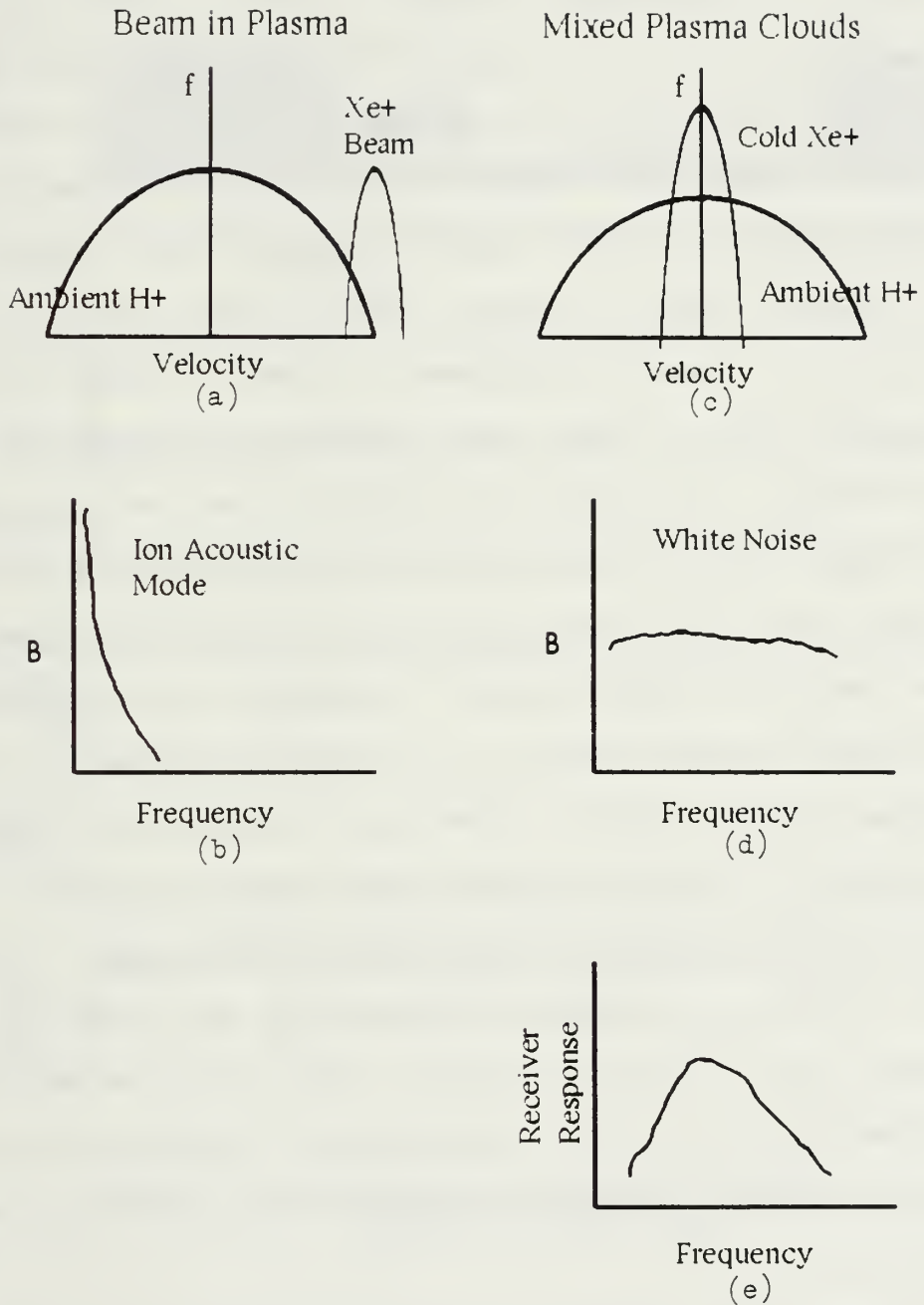
Figure 14. Plasma waves generated by beam-plasma interactions.
