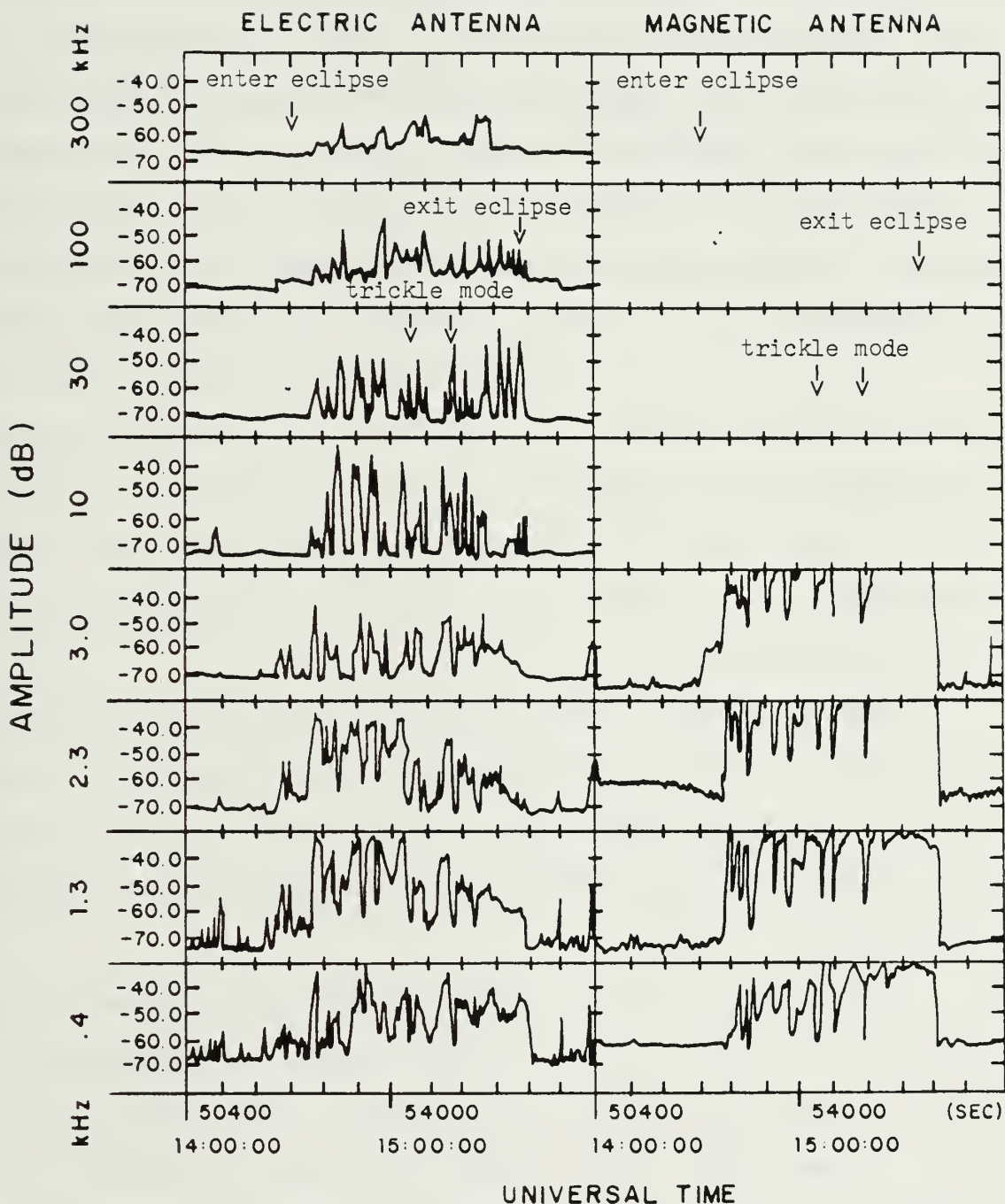
Figure 25. Narrowband filter data for 1400 - 1600 2 April 1979.
