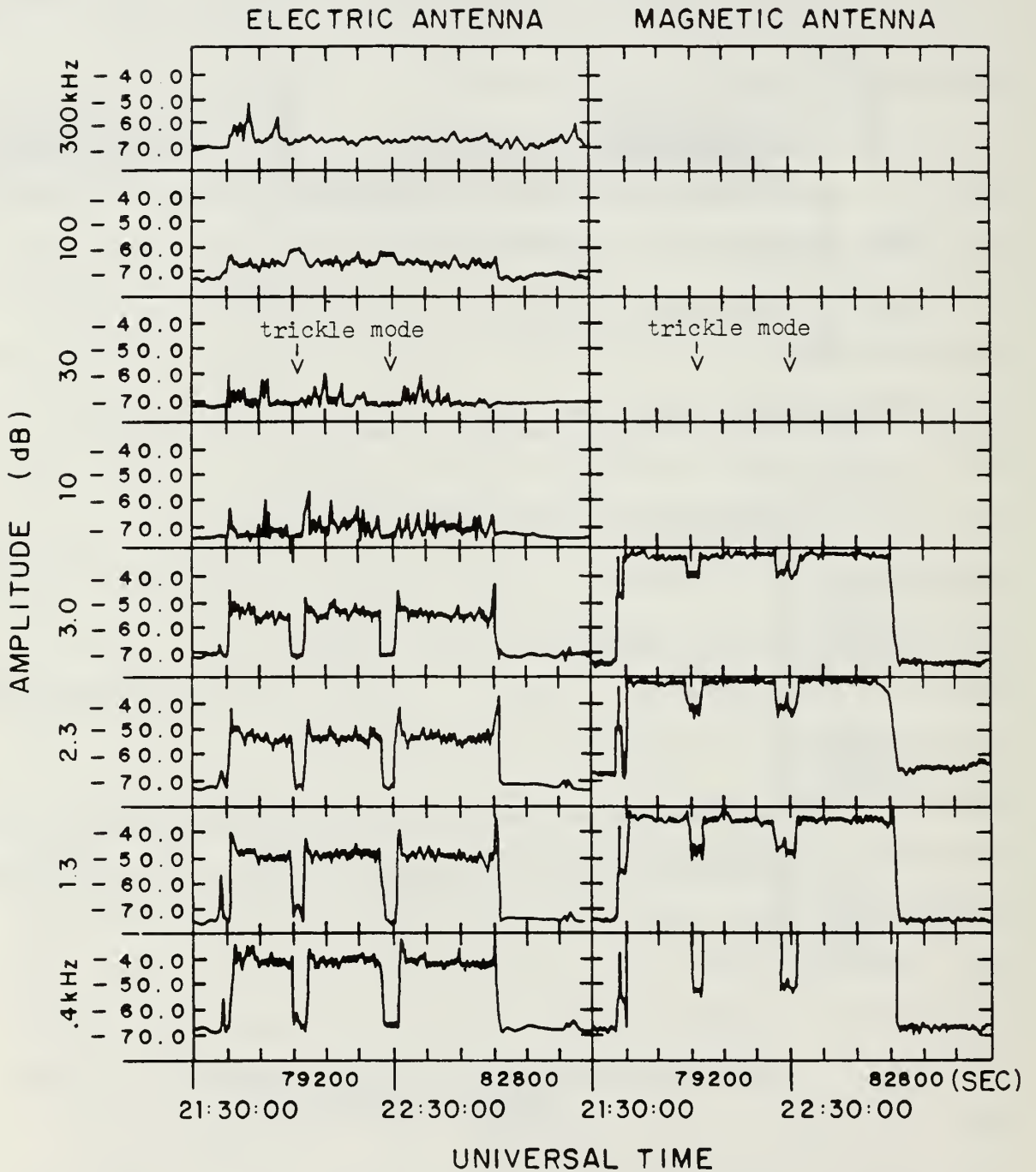
Figure 17. Narrowband filter data for 2130 - 2330 19 July 1979.
