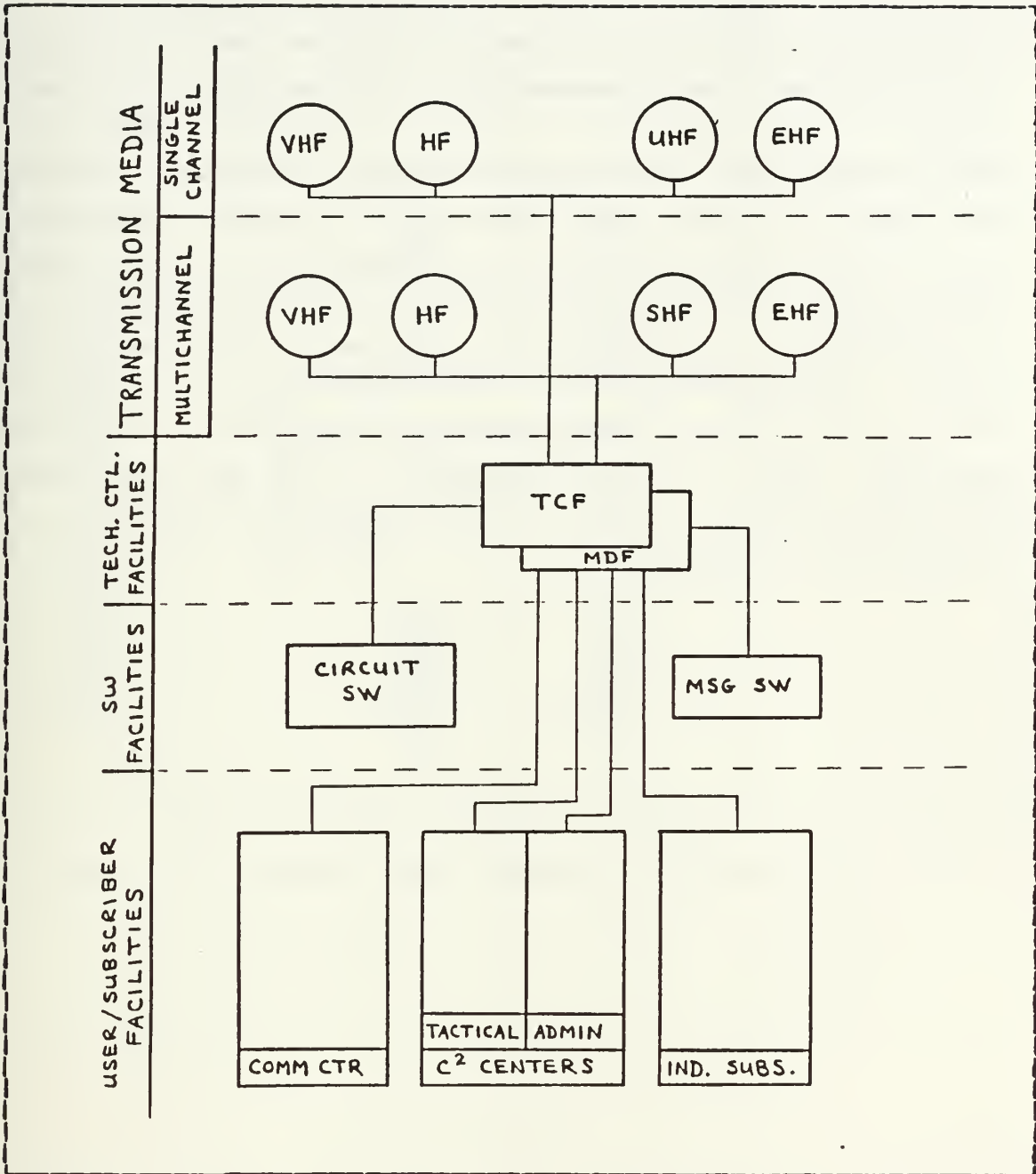
Figure D.3 Diagram of Generic LFICS Node.
