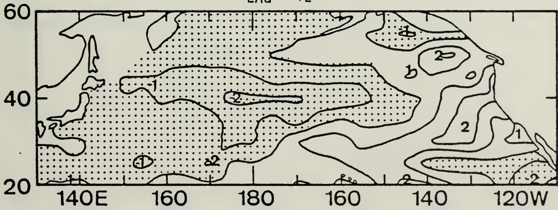
Figure 19. Same as Fig. 18 except for 0, +1, and +2 month lags.
