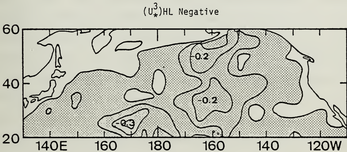
Figure 32. Correlations between (U_*^3) HL and \partial/\partial t SST 3 for positive (top) and negative (bottom) values of (U_*^3) HL separately. Contour interval is 0.1 and shaded areas denote negative correlations.
