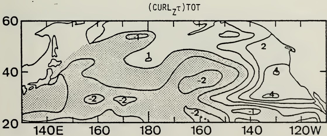
Figure 21. Normalized correlations at zero lag between \partial/\partial t SST and (\text{CURL}_{z\tau})_H , (\text{CURL}_{z\tau})_{HL} and (\text{CURL}_{z\tau})_{TOT} . Contour interval is 1 and shaded areas denote negative correlations.
