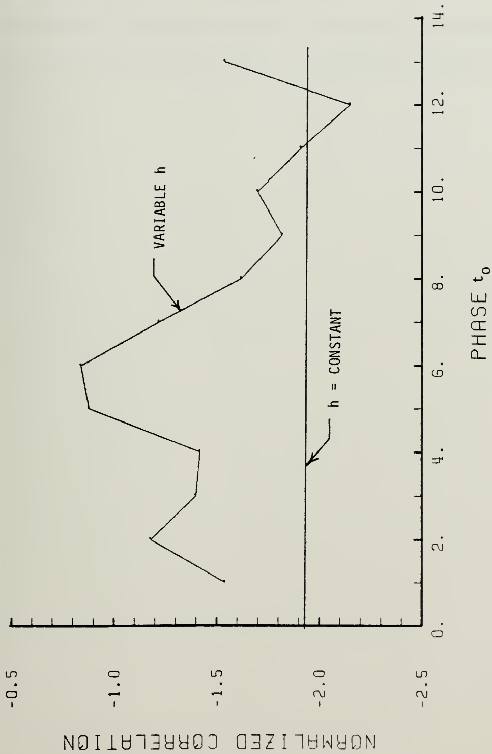
Figure 31. Same as Fig. 30 except for Central North Pacific Ocean Index Area.
