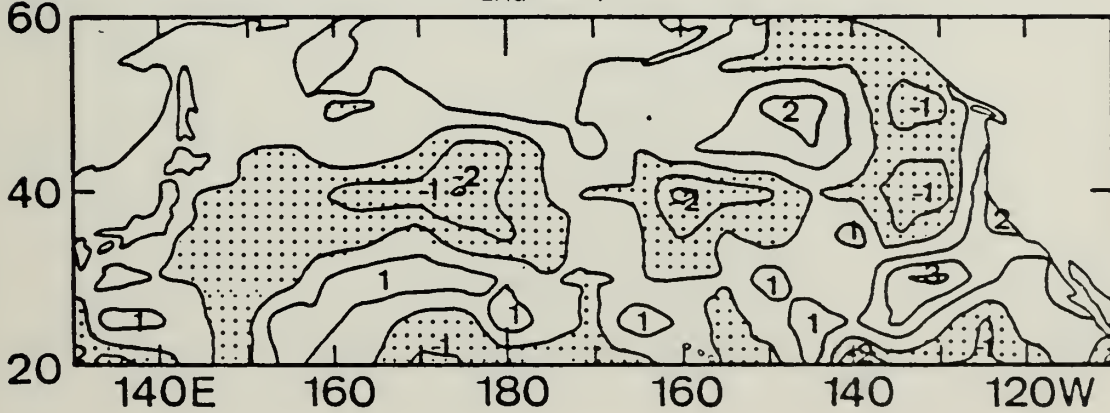
Figure 12. Same as Fig. 3 except for (\text{CURL}_Z \tau)H .
