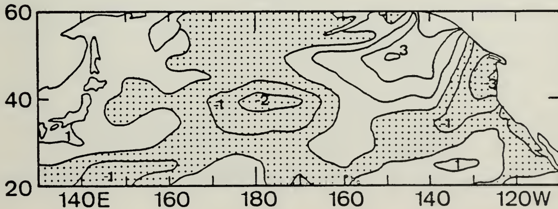
Figure 6. Same as Fig. 3 except for (U_{*}^3)HL .
