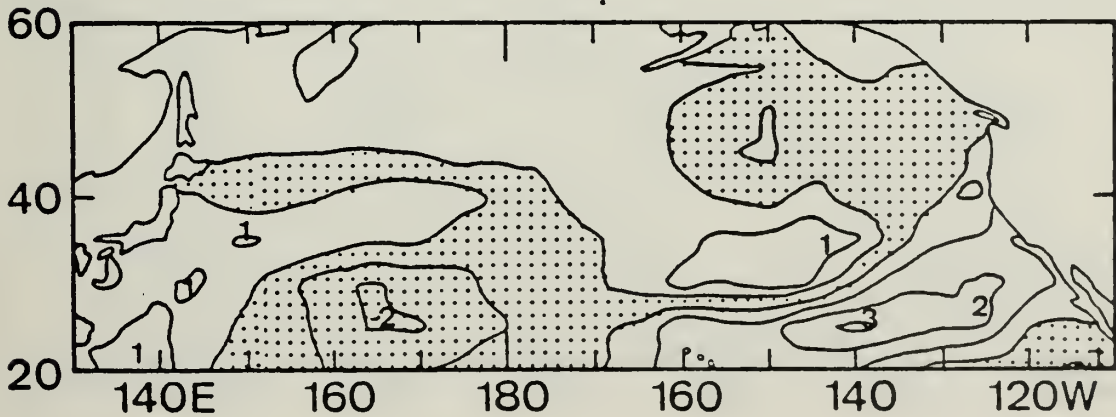
Figure 8. Same as Fig. 6 except for +3, +4 and +5 month lags.
