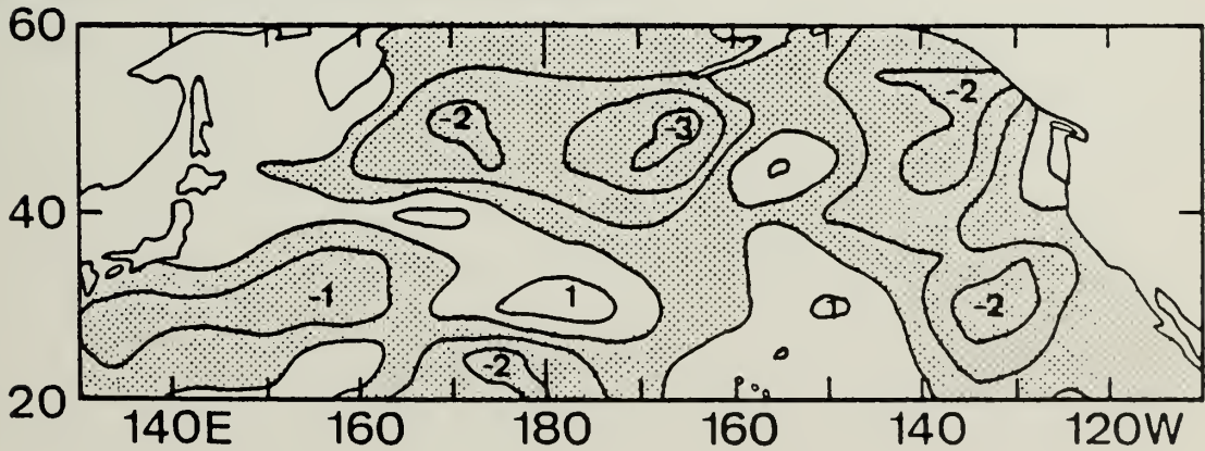
Figure 22. Same as Fig. 21 except for (U_{\star}^3)_H , (U_{\star}^3)_{HL} and (U_{\star}^3)_{TOT} .
