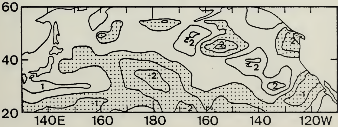
Figure 9. Same as Fig. 3 except for (U_*^3)_{TOT} .
