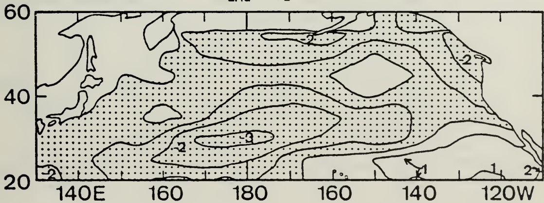
Figure 4. Same as Fig. 3 except for 0, +1 and +2 month lags.
