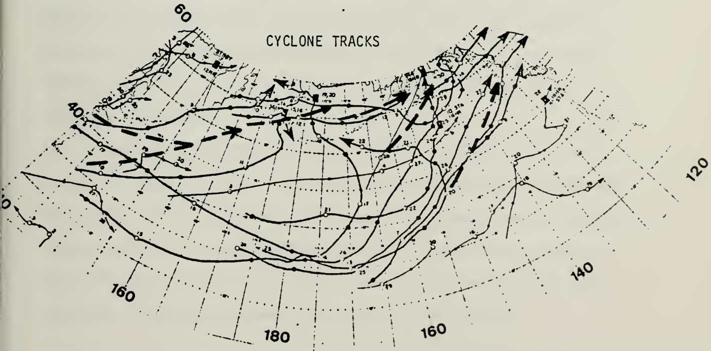
Figure 36. Same as Fig. 34 except for November, 1977.
