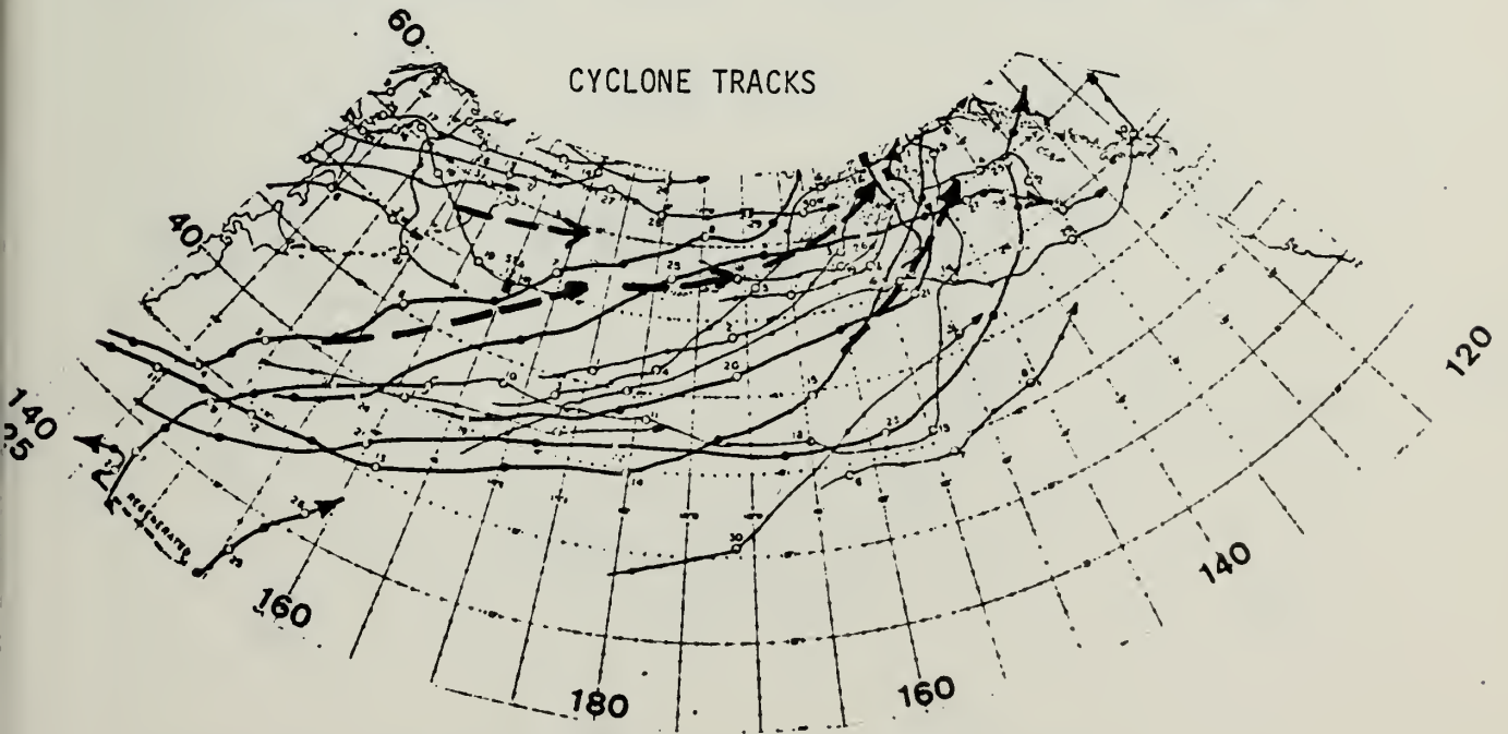
Figure 35. Same as Fig. 34 except for October, 1977.
