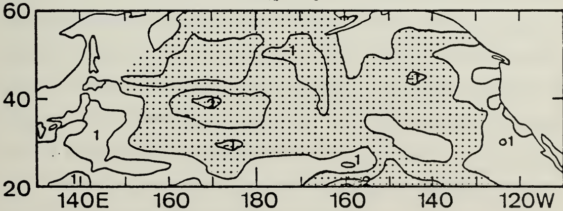
Figure 11. Same as Fig. 9 except for +3, +4 and +5 month lags.
