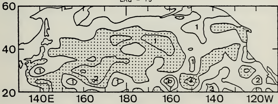
Figure 14. Same as Fig. 12 except for +3, +4 and +5 month lags.
