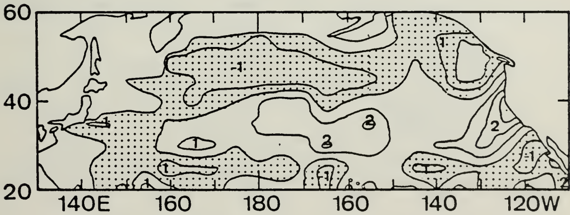
Figure 15. Same as Fig. 3 except for (\text{CURL}_Z \tau)_{HL} .
