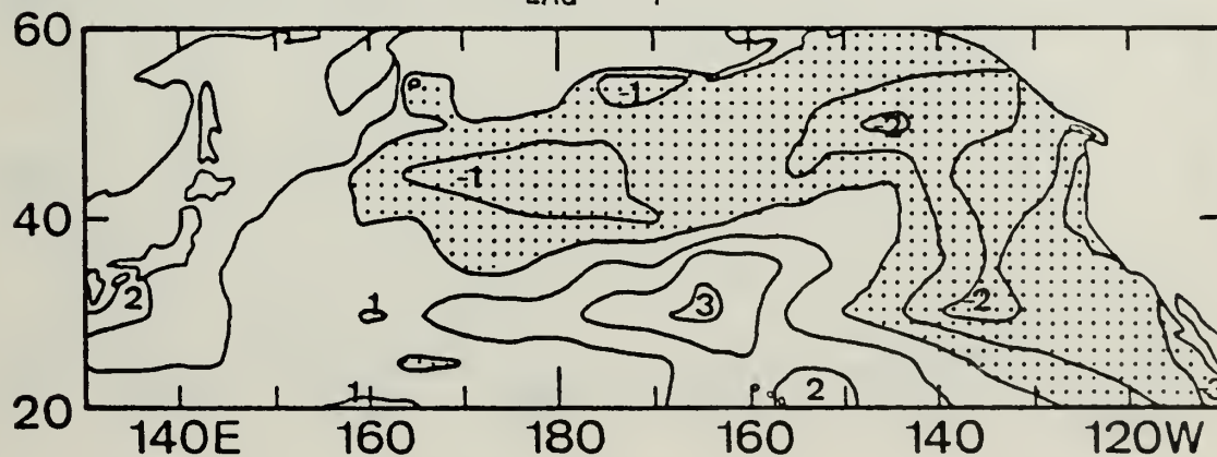
Figure 18. Same as Fig. 3 except for (CURL Z τ)TOT.
