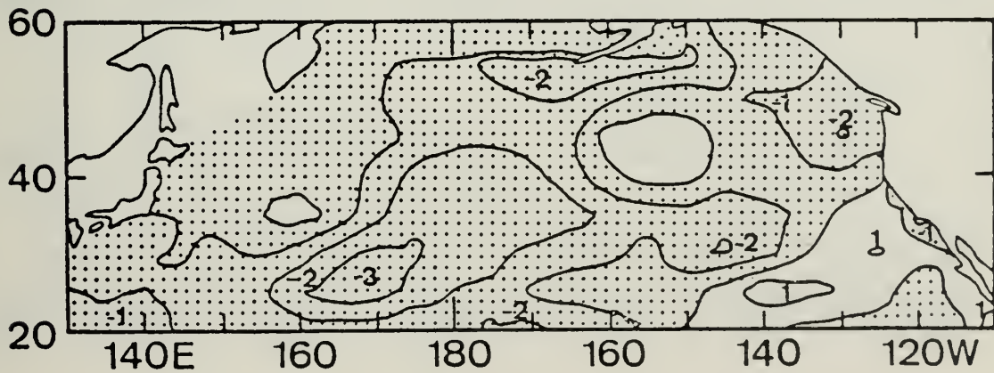
Figure 7. Same as Fig. 6 except for 0, +1 and +2 month lags.
