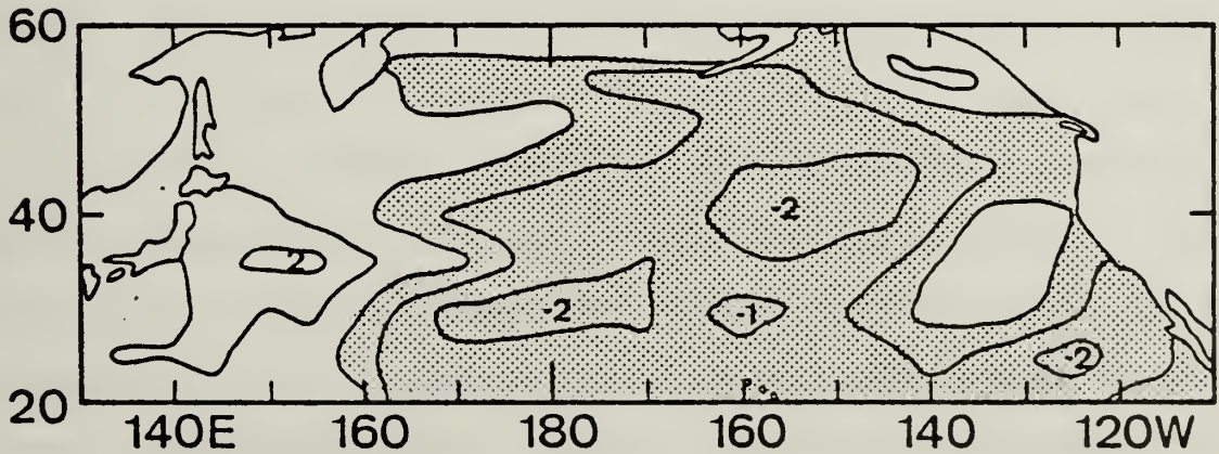
Figure 28. Same as Fig. 25 except for October, November and December.
