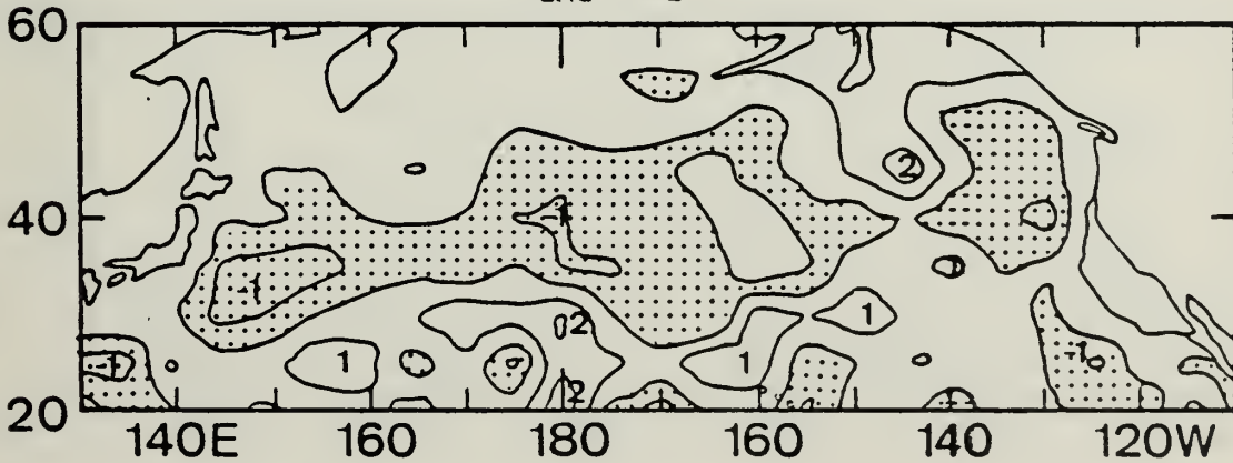
Figure 13. Same as Fig. 12 except for 0, +1 and +2 month lags.
