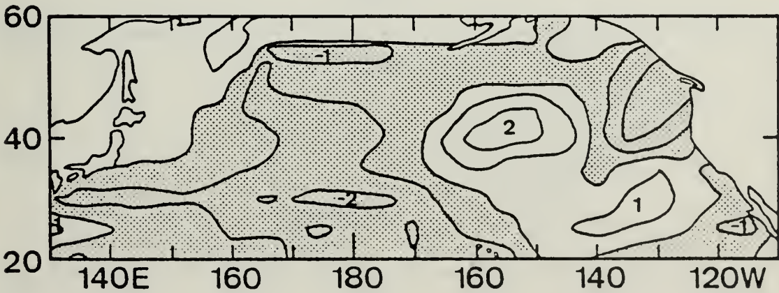
Figure 25. Subsample record correlations (nondimensionalized by \sigma_k^* ) between SST and (U_*^3)_{HL} for +1 month lag and starting months January (top), February (middle), and March (bottom). Contour interval is 1 and shading indicates negative correlations.
