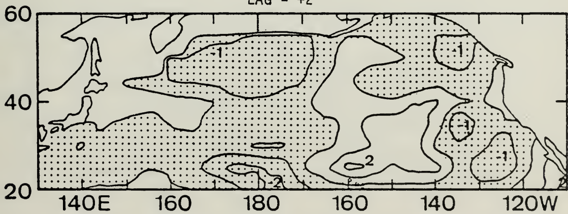
Figure 10. Same as Fig. 9 except for 0, +1 and +2 month lags.
