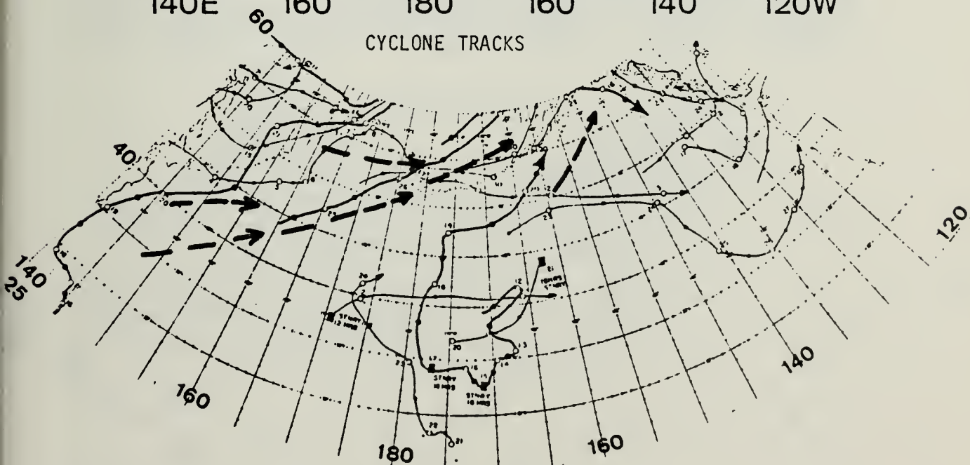
Figure 34. SST anomaly values ( ^{\circ}\text{C} ), (U_*^3)_{HL} anomaly values (units 10^4 (\text{cm}/\text{sec})^3 ) and cyclone tracks (Mariners Weather Log) for the month of September 1977. Contour interval is 0.5 and shaded areas denote negative values. Heavy dashes denote climatological tracks (Klein 1956).
