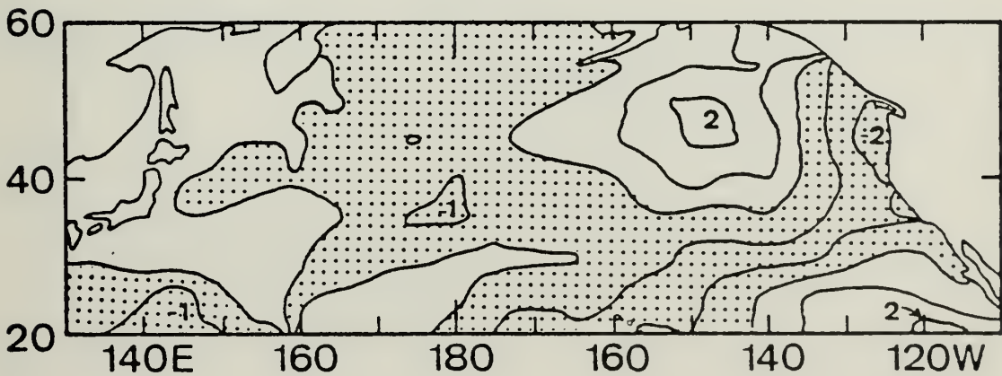
Figure 3. Normalized correlation between (U_*^3)H and SST at -3, -2, and -1 month lag. Contour interval is 1 and several closed contours are labeled. Shaded areas denote negative values.
