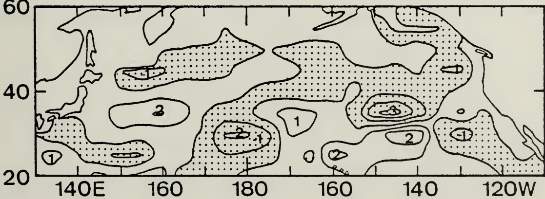
Figure 17. Same as Fig. 15 except for +3, +4 and +5 month lags.
