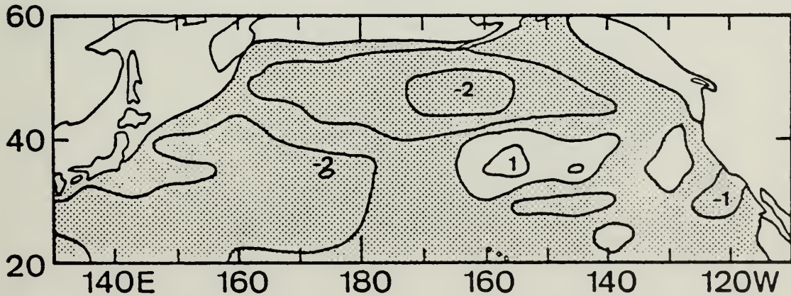
Figure 27. Same as Fig. 25 except for July, August and September.
