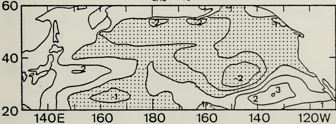
Figure 5. Same as Fig. 3 except for +3, +4 and +5 month lags.
