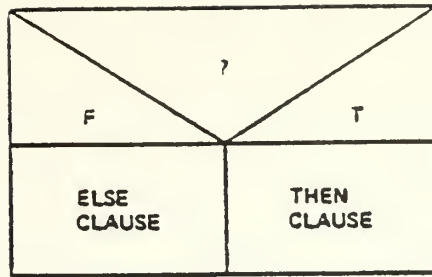
Decision Symbol
