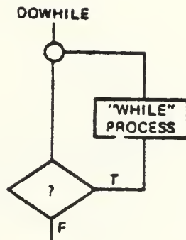
DO WHILE
