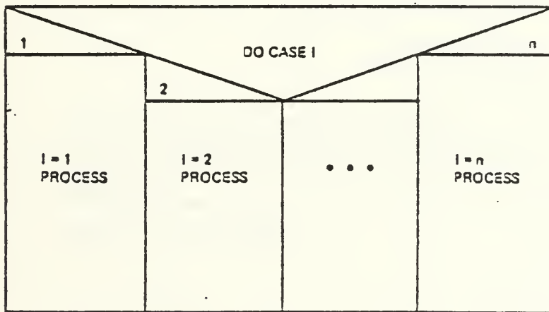
CASE Symbol
