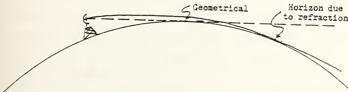
Figure 7. Horizon Extension Due to Refraction
