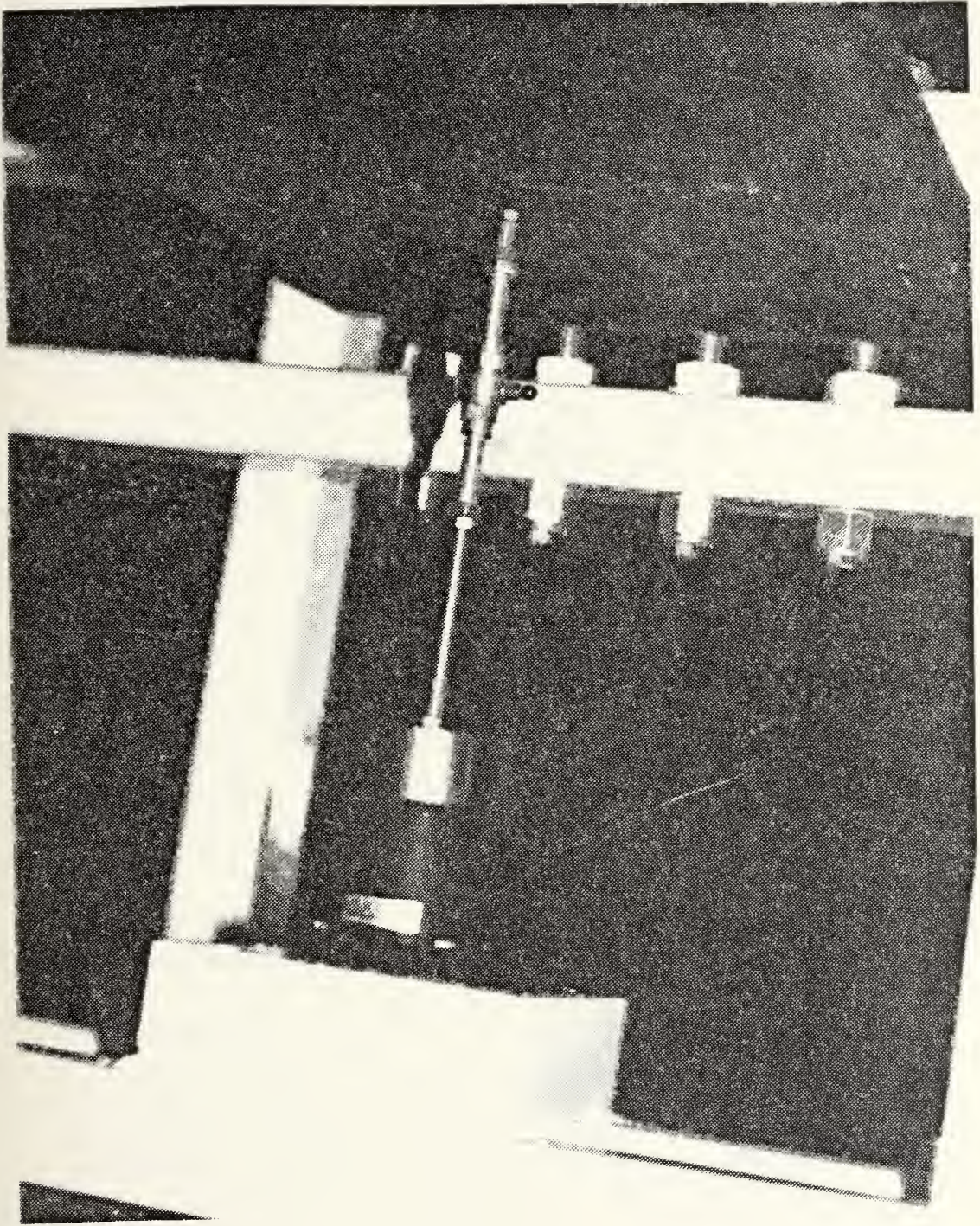
Figure 10. Exciter drive mechanism with force transducer
