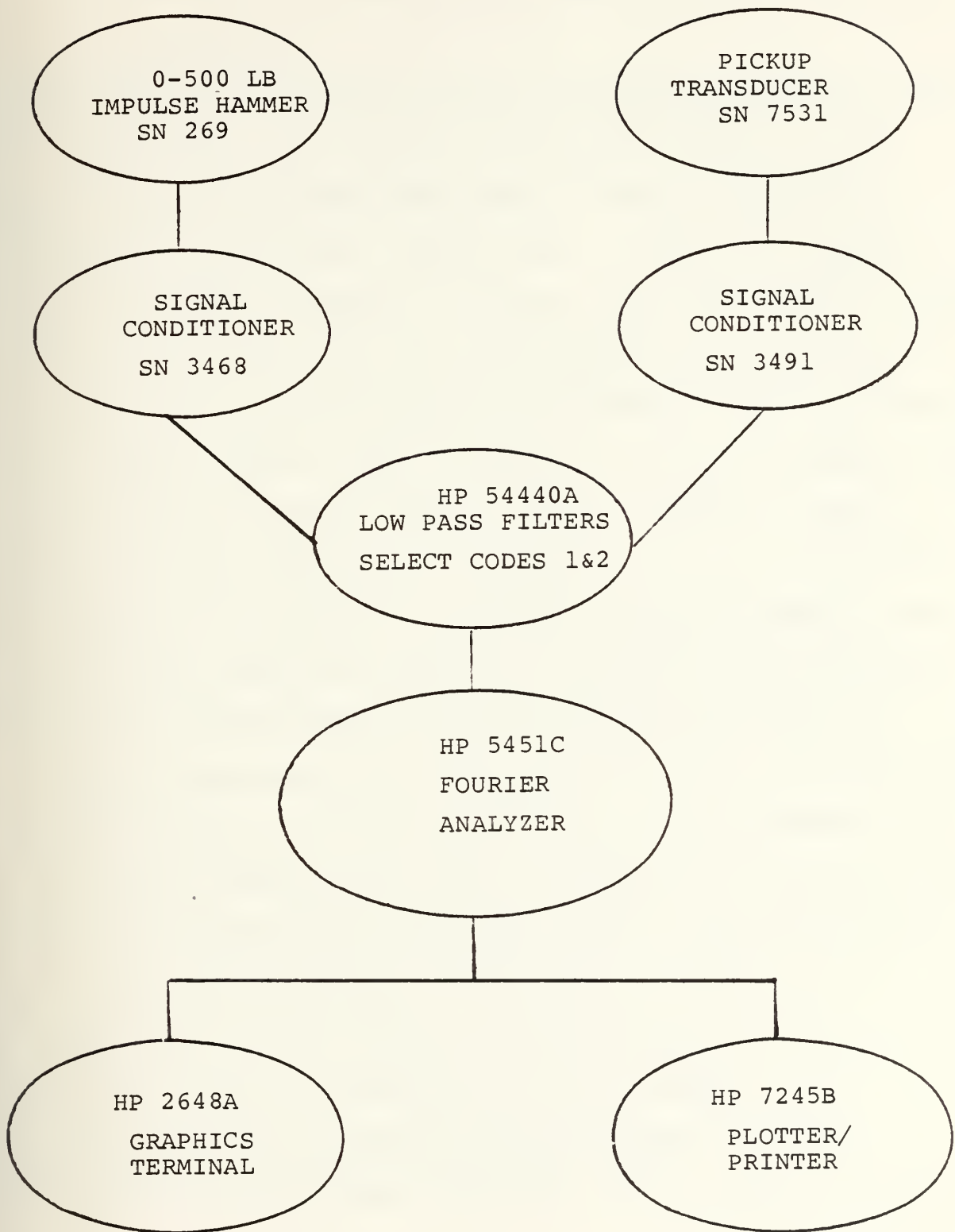
Figure 11. Impulse hammer technique flow chart
