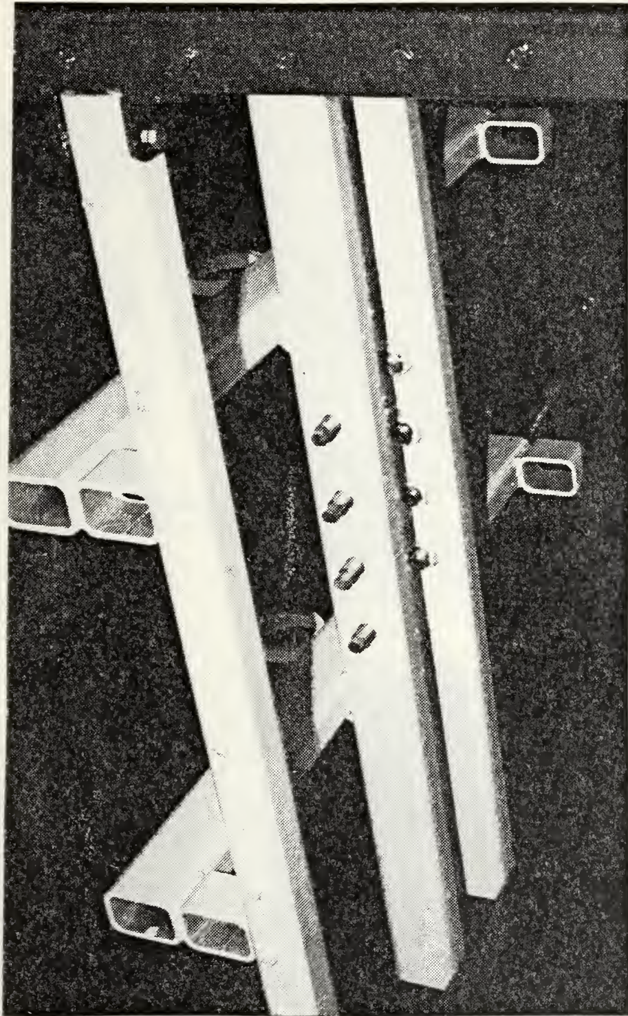
Figure 2. Detail of specimen support fixture
