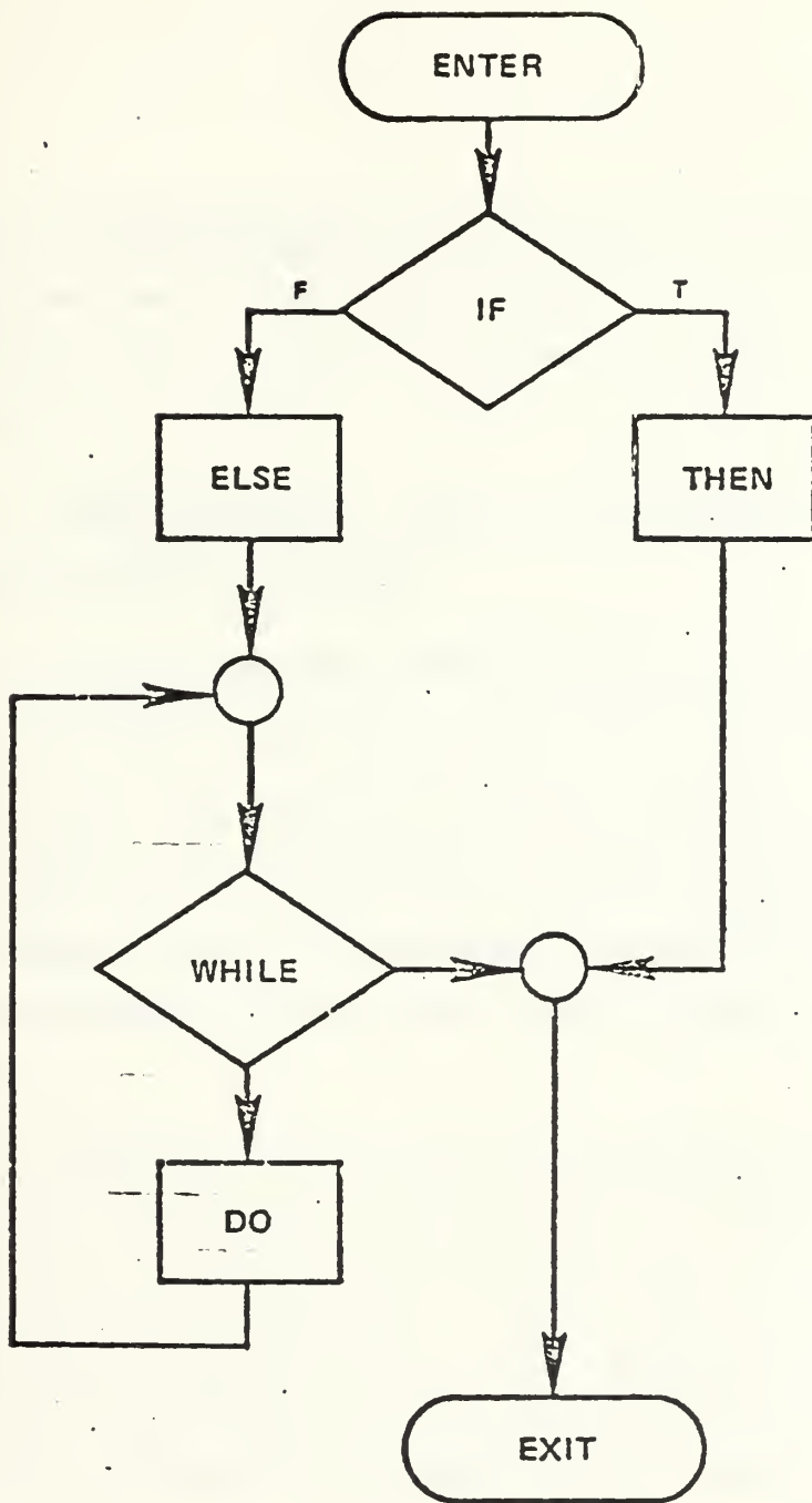
FIGURE 2. Nesting of Control Structures.
