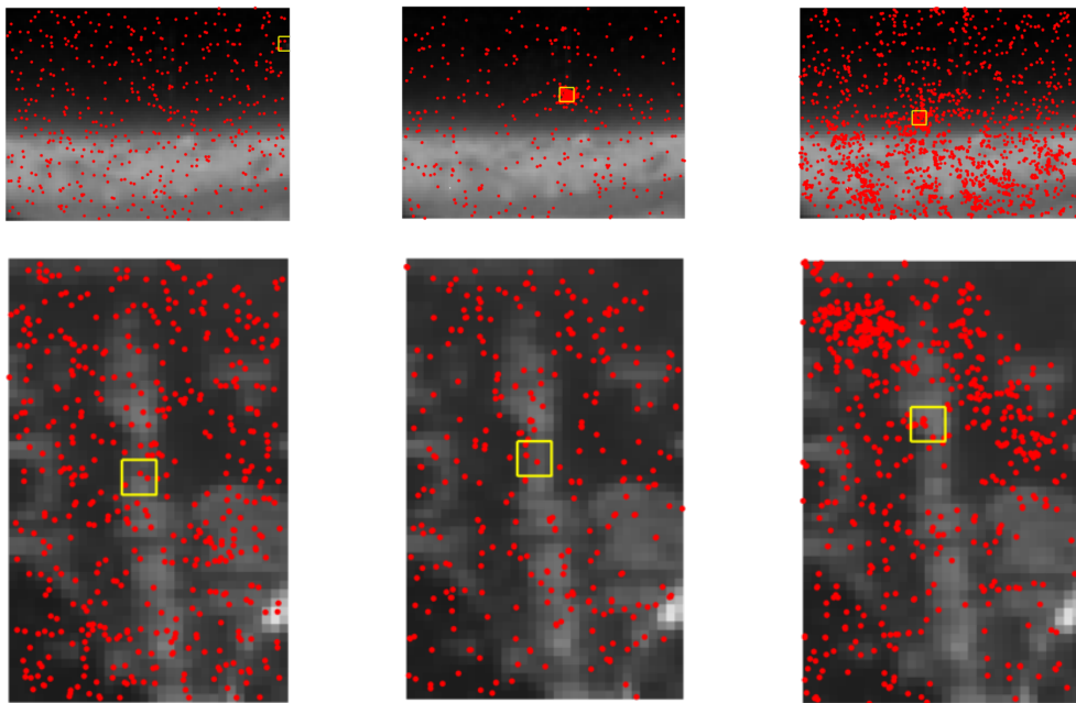
Figure 17: Three frames showing the TBD estimated paths for the “plane” and “car” quasi real-world data set. A box is drawn over the target in each frame, and the current path estimate is drawn as a white line. The top row contains frames 1, 245, and 491 from the plane data set. The second row contains frames 1, 150, and 301 from the car data set. The red dots indicate the particle distribution of the TBD filter at the current frame. All images have been contrast enhanced for clearer viewing.
