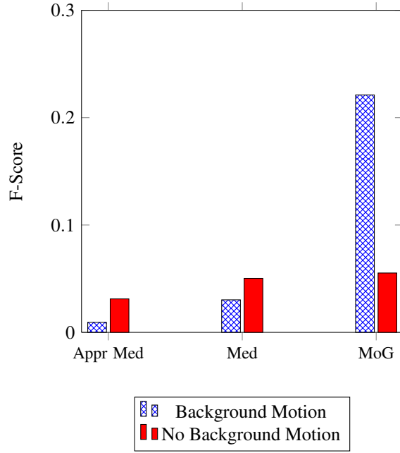
Figure 8: Comparison of F-scores for approximated median, median, and mixture of Gaussians background subtraction with a subpixel target in the foreground.
