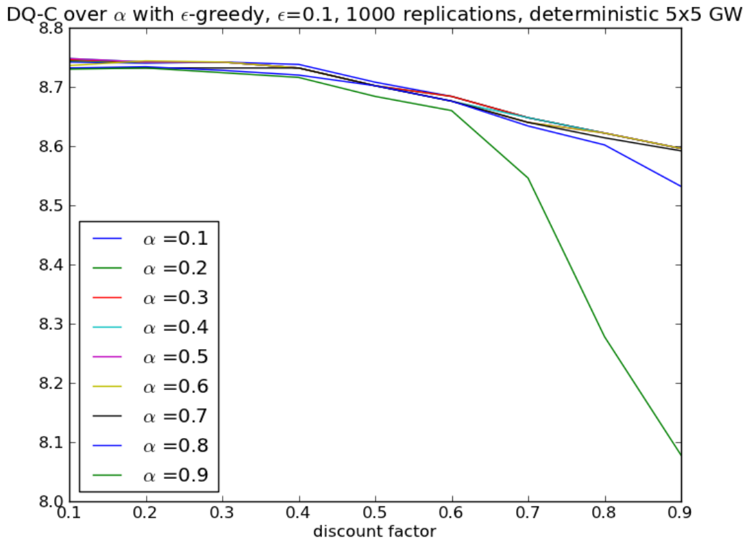
Figure 54: Performance of DQ-C in 5x5 deterministic grid world over \gamma by \alpha paired with \epsilon -greedy.
