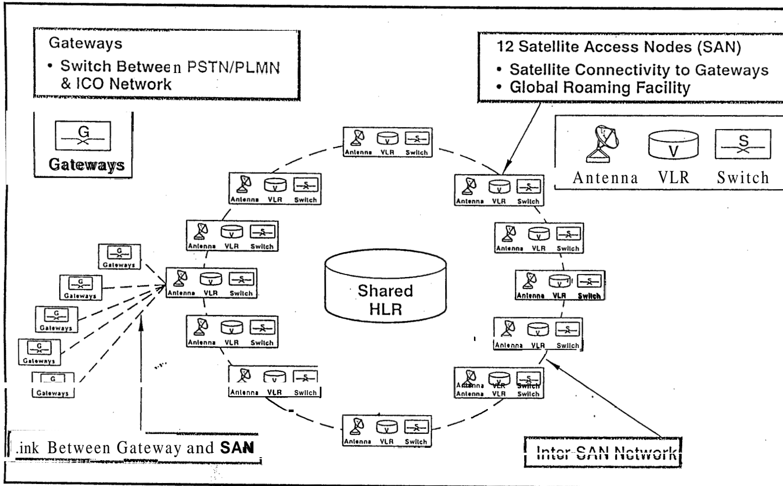
Figure 2.6 The ICO Network "From Ref. [16]."
