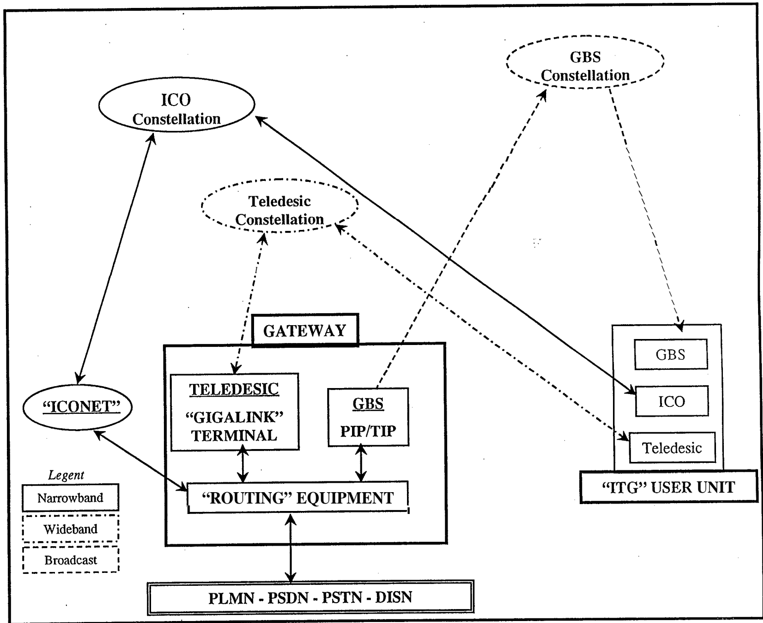
Figure 5.2 The "ITG" Flow of Information Diagram.
