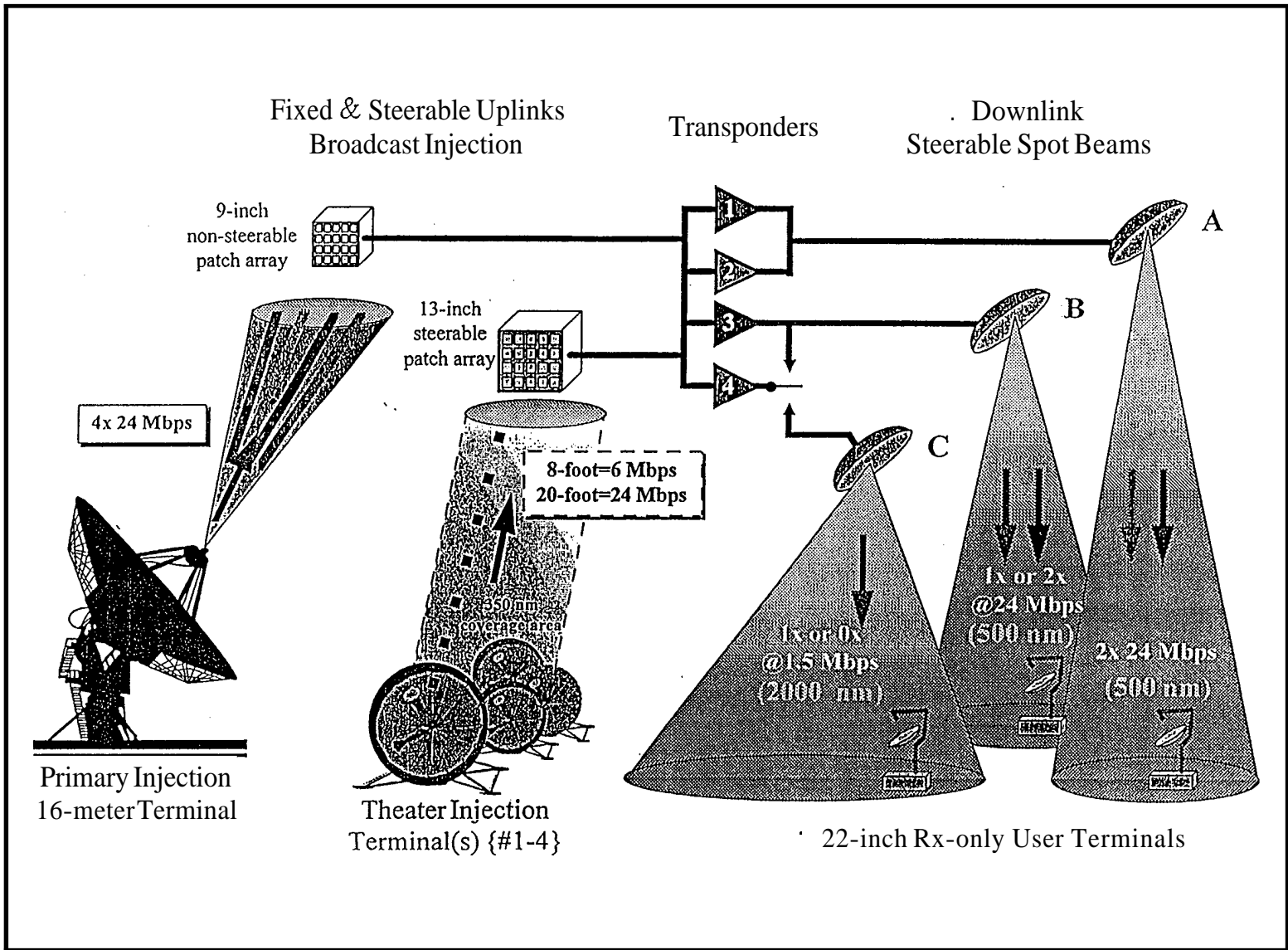
Figure 4.3 The GBS on UFO(Phase II) Configuration "From Ref. [25]."
