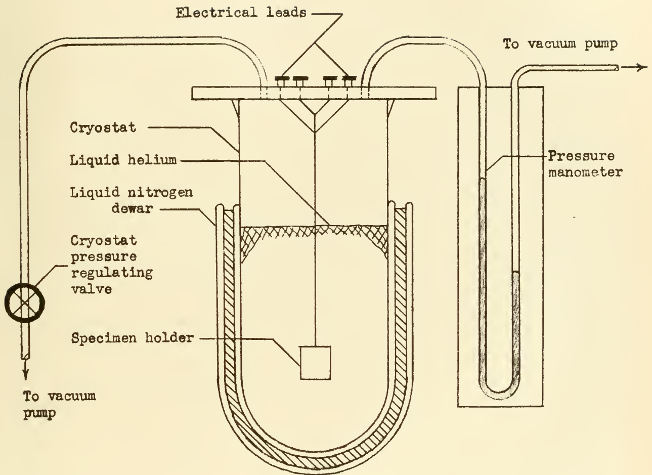
EQUIPMENT SCHEMATIC
