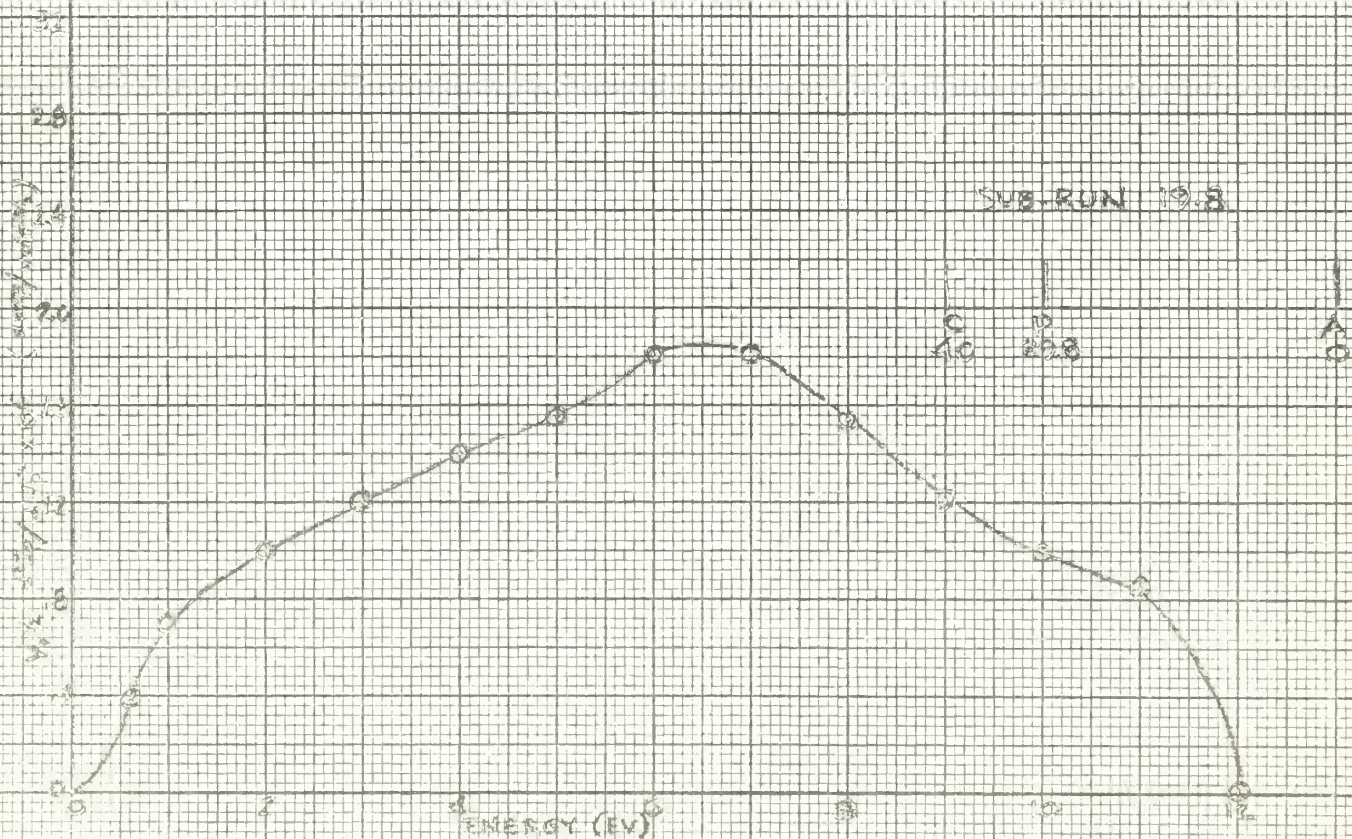
FIG. 57 ELECTRON ENERGY DISTRIBUTION, RUN 19 NEON
