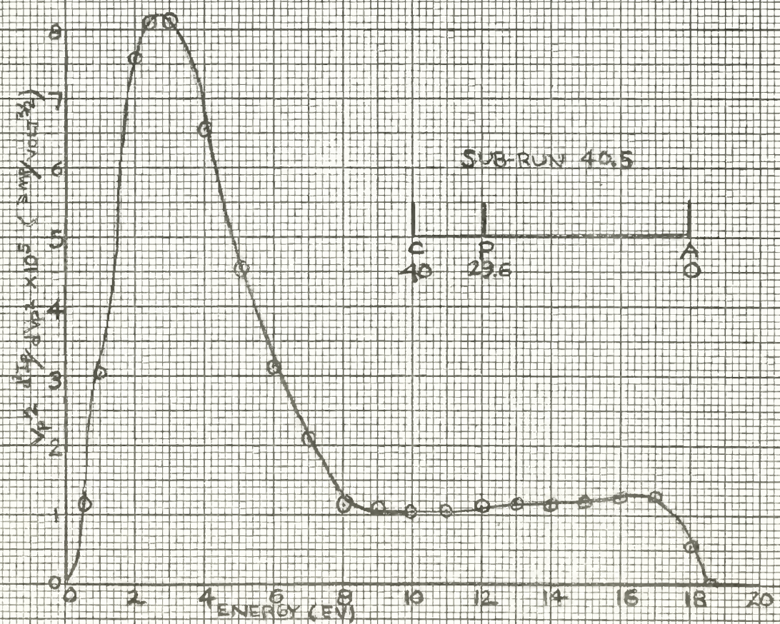
FIG. 65 ELECTRON ENERGY DISTRIBUTION, RUN 40 KRYPTON
