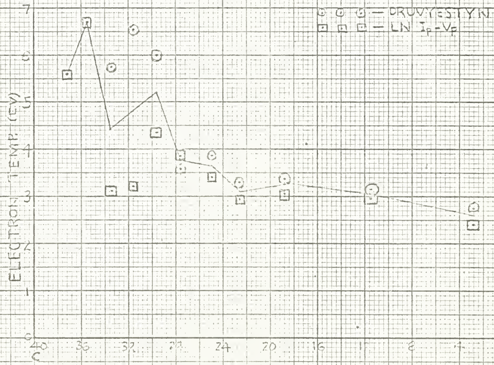
FIG. 55 ELECTRON TEMPERATURE VS. PROBE POSITION, RUN 40 KRYPTON
