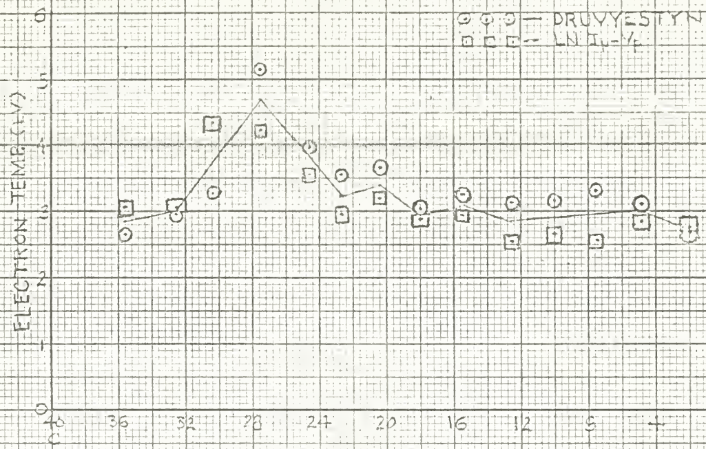
FIG. 54 ELECTRON TEMPERATURE VS. PROBE POSITION, RUN 39 ARGON
