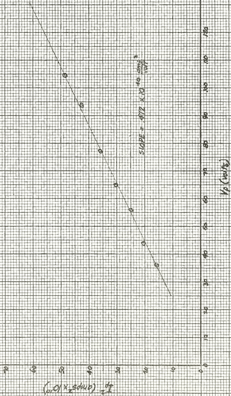
Figure 51. Sample I_p^2 versus V_p Plot (Run 39.7)
