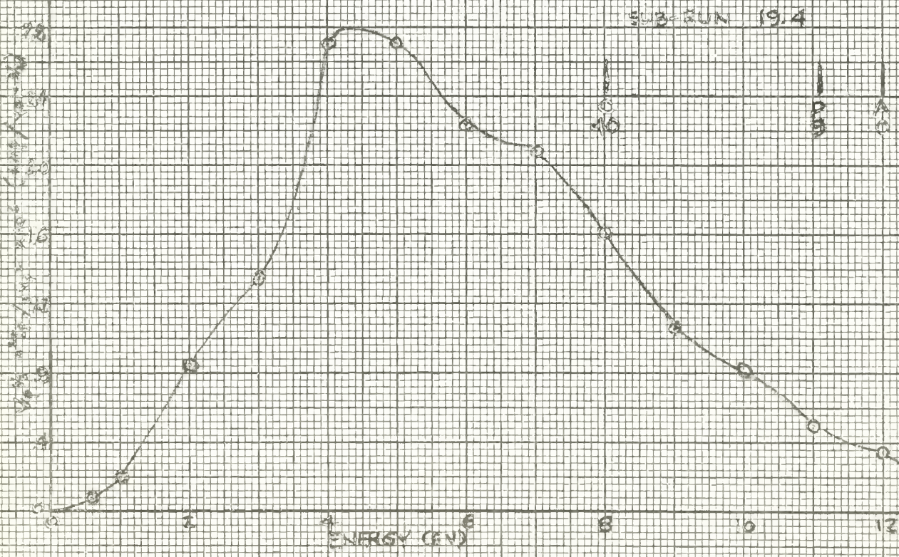
FIG. 56 ELECTRON ENERGY DISTRIBUTION, RUN 19 NEON
