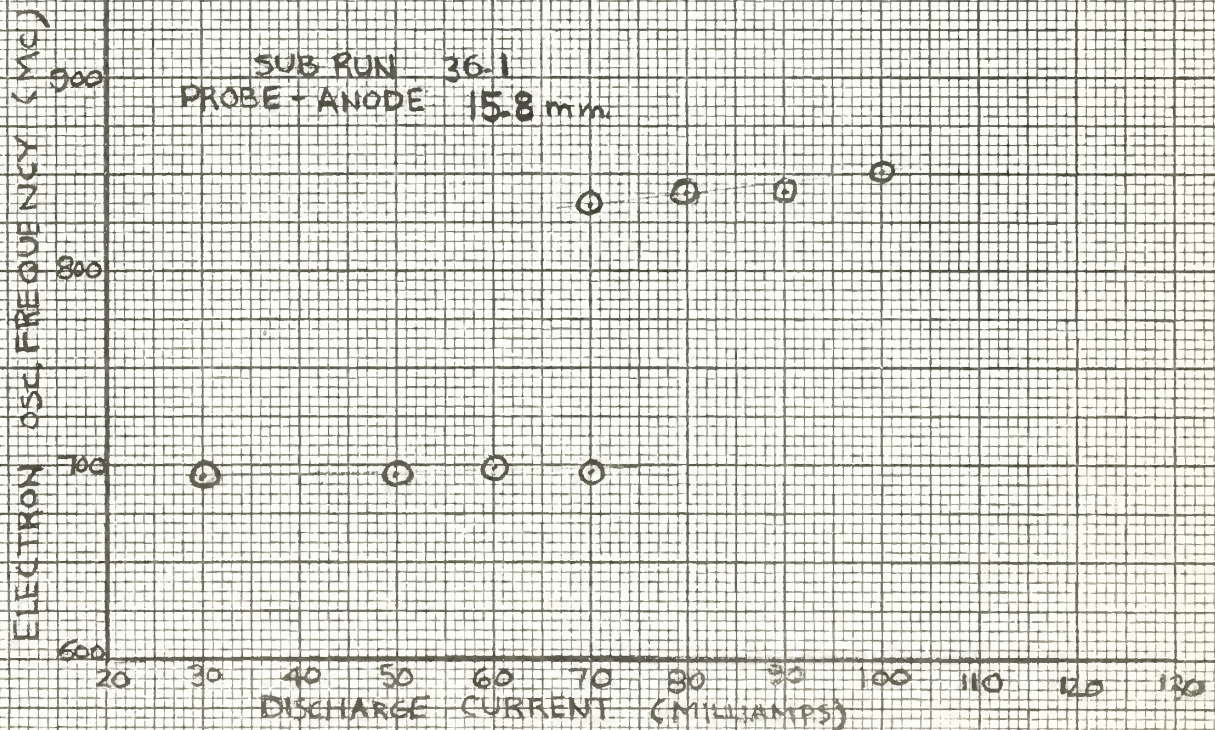
FIG. 76 ELECTRON OSCILLATION FREQUENCY VS. DISCHARGE CURRENT, ARGON 109
