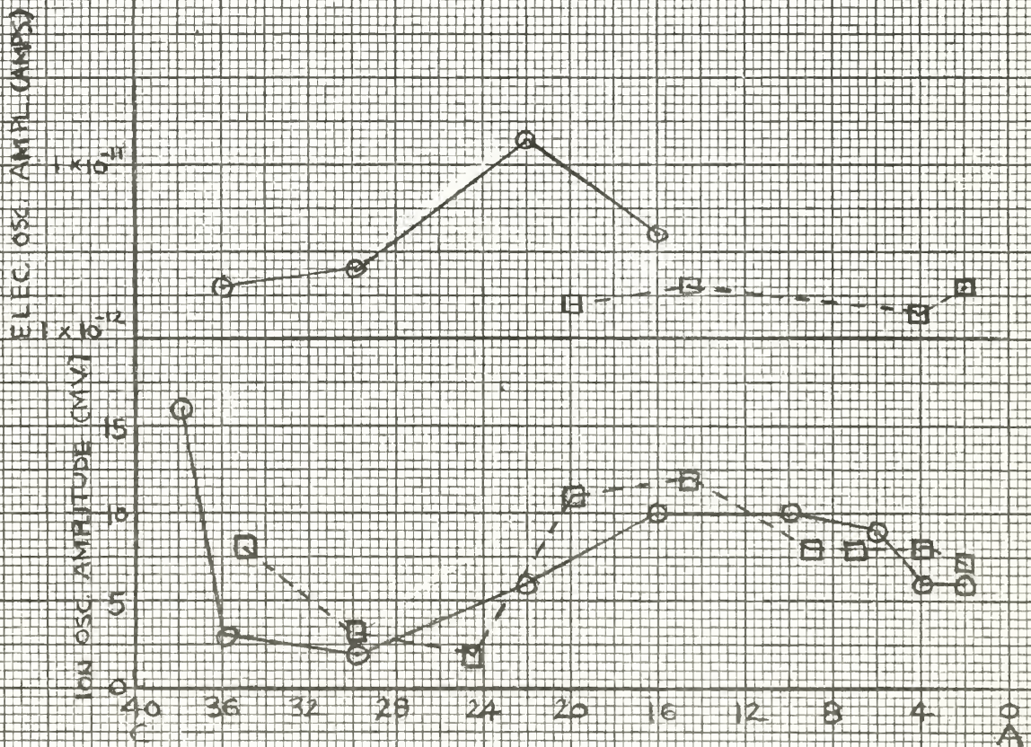
FIG. 72 ELECTRON OSCILLATION AMPLITUDE, ION OSCILLATION AMPLITUDE, ELECTRON DENSITY VS POSITION □ □ □ - RUN 19, NEON ○ ○ ○ - RUN 21, NEON
