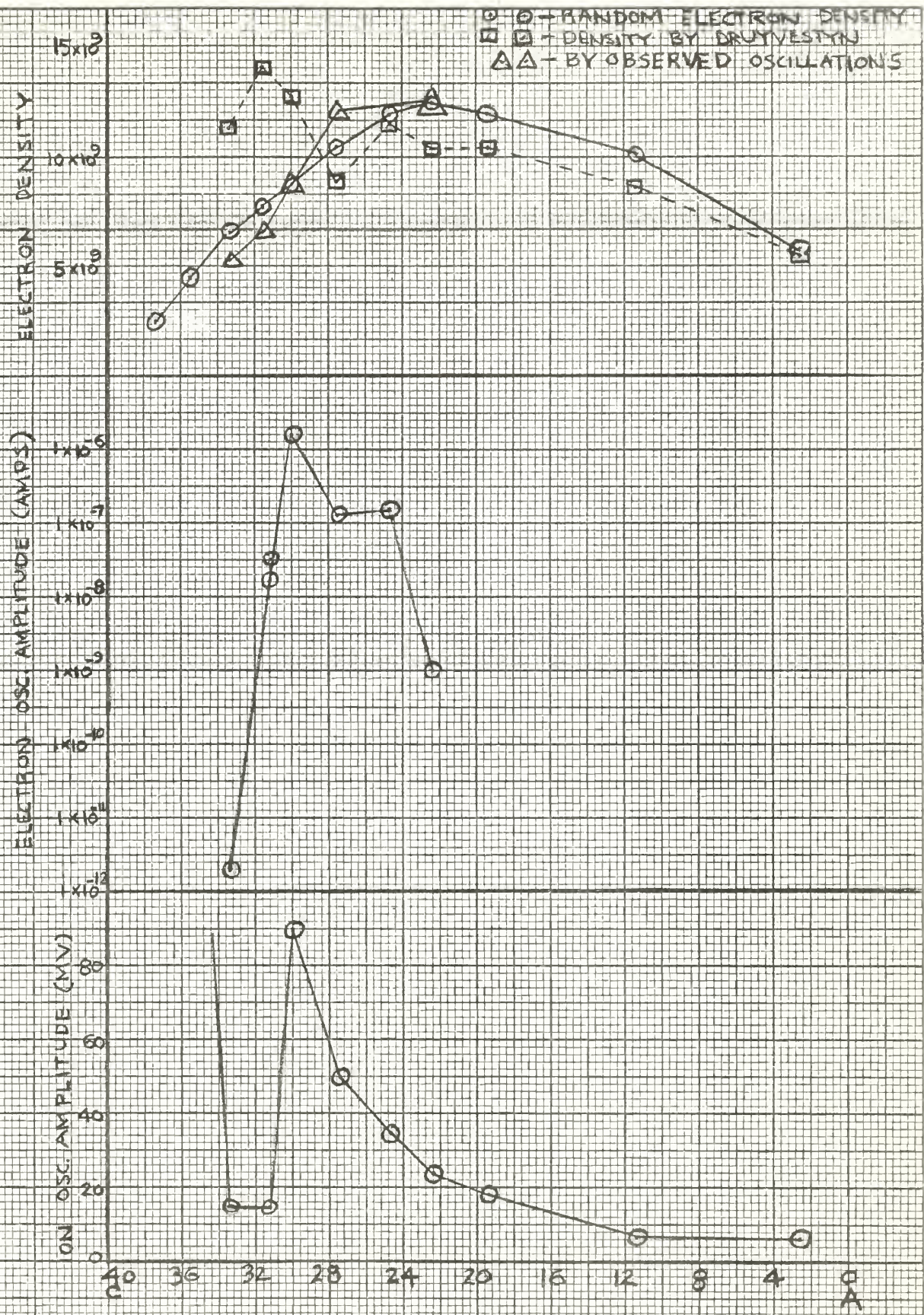
FIG 74 ELECTRON OSCILLATION AMPLITUDE, ION OSCILLATION AMPLITUDE, ELECTRON DENSITY VS POSITION RUN 40, KRYPTON 107
