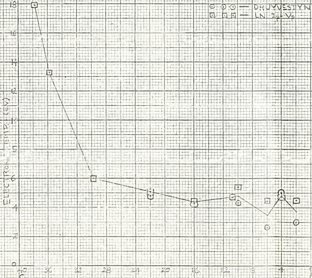
FIG. 53 ELECTRON TEMPERATURE VS. PROBE POSITION, RUN 21 NEWM
