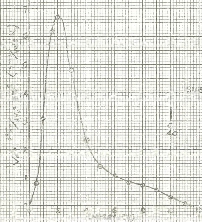
FIG. 60 ELECTRON ENERGY DISTRIBUTION, RUN 39 ARGON
