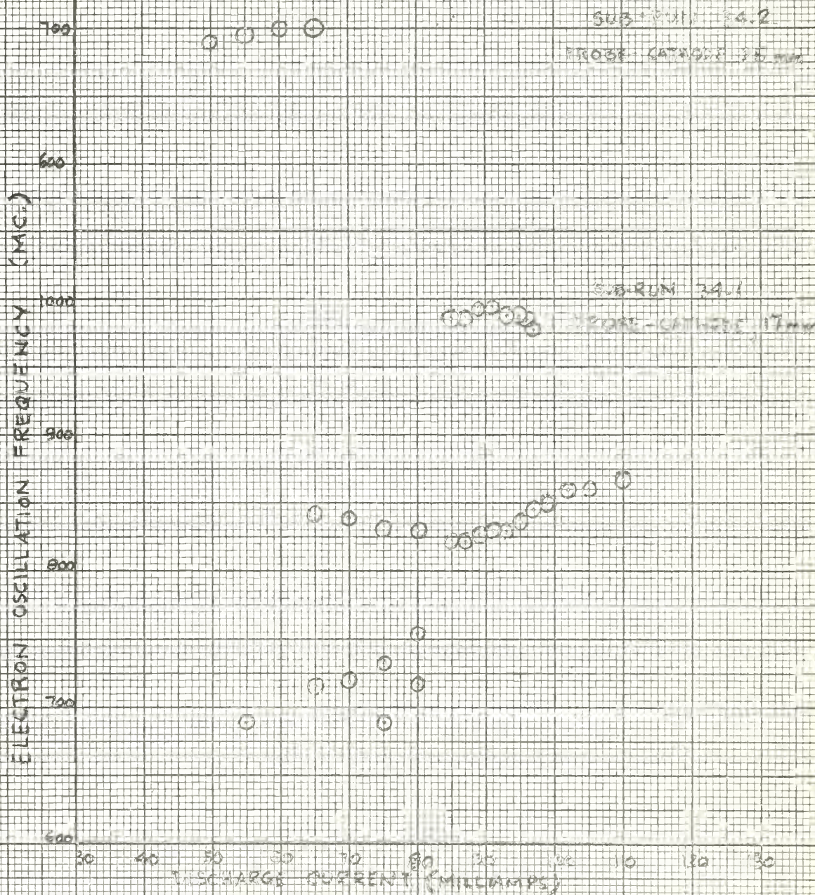
FIG. 75. ELECTRON OSCILLATION FREQUENCY VS. DISCHARGE CURRENT, ARGON
