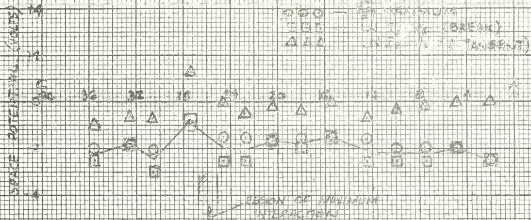
FIG. 44 SPACE POTENTIAL VS. PROBE POSITION, RUN 39, ARGON
