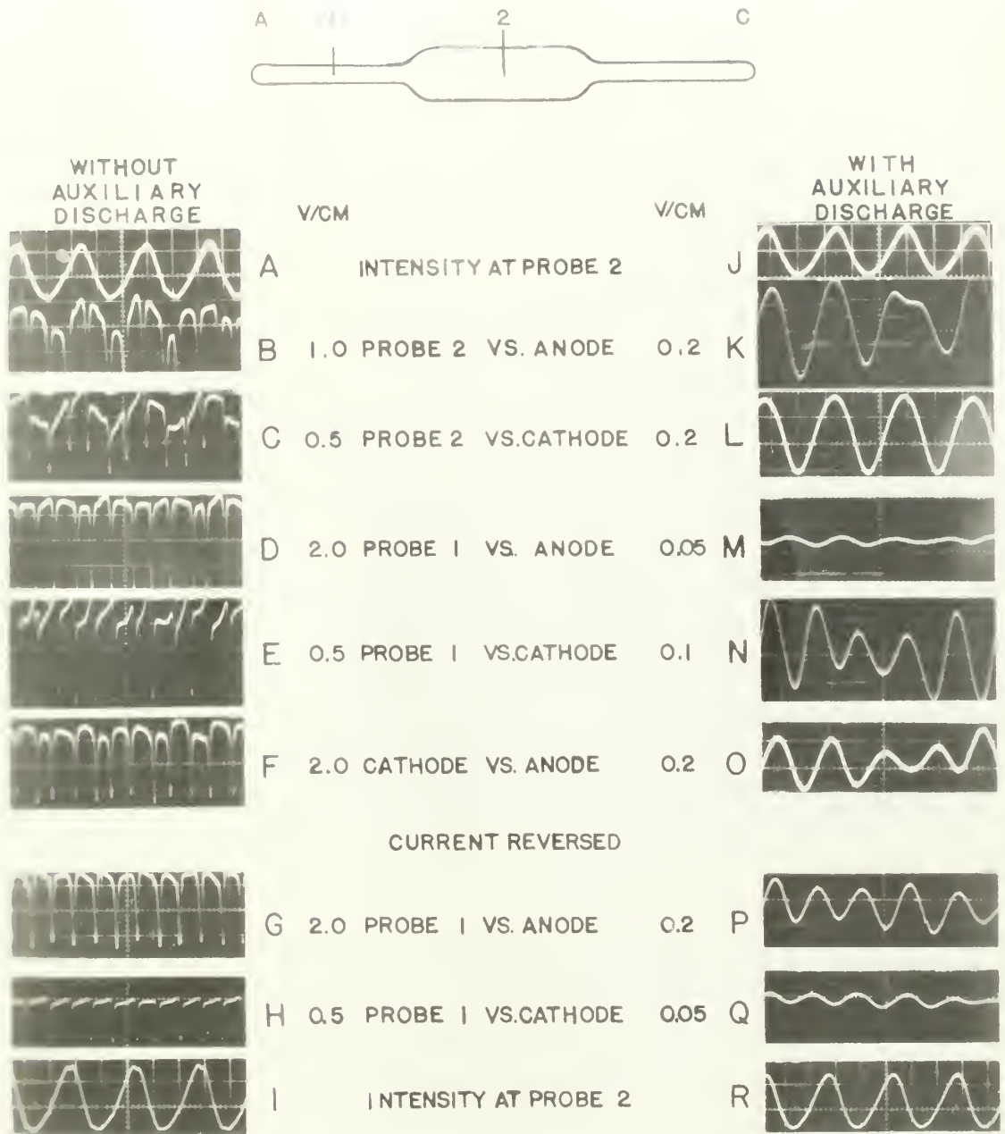
FIG. 43 LIGHT INTENSITY AND FLOATING POTENTIAL WAVEFORMS IN TUBE 3 ARGON 9.5 MM HG. CURRENT 475 MA.
