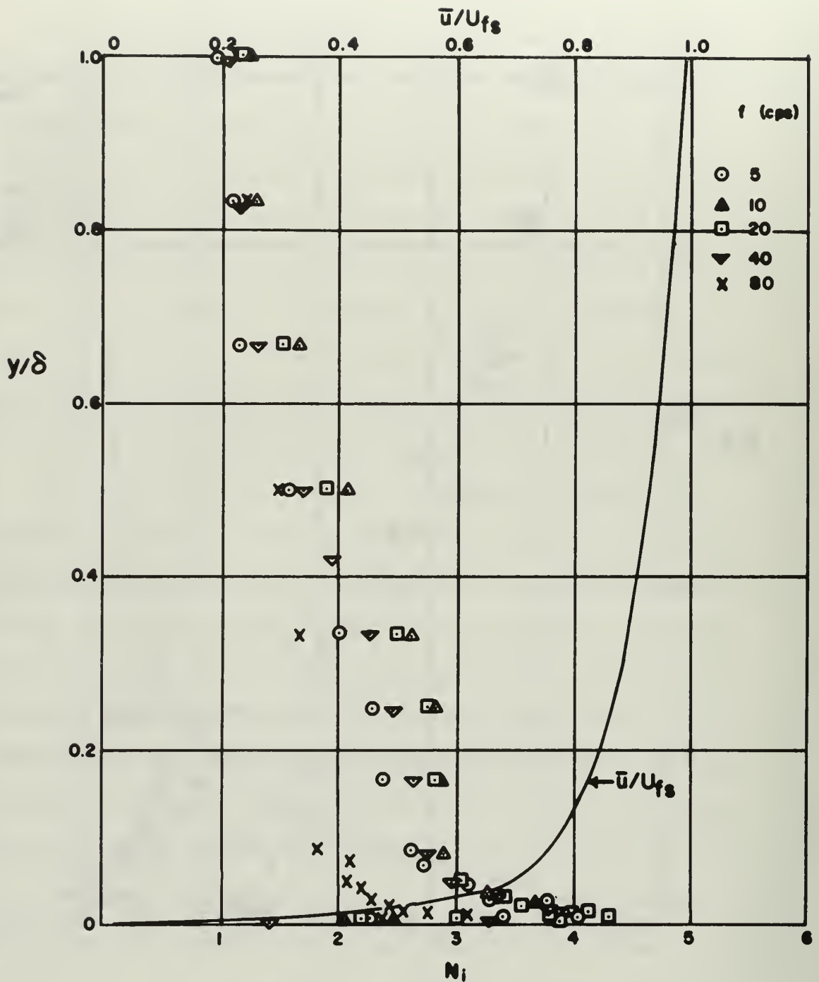
FIGURE 12 DISTRIBUTION OF TURBULENT INTENSITIES. N_e = .18 R_x = 1.5 \times 10^6
