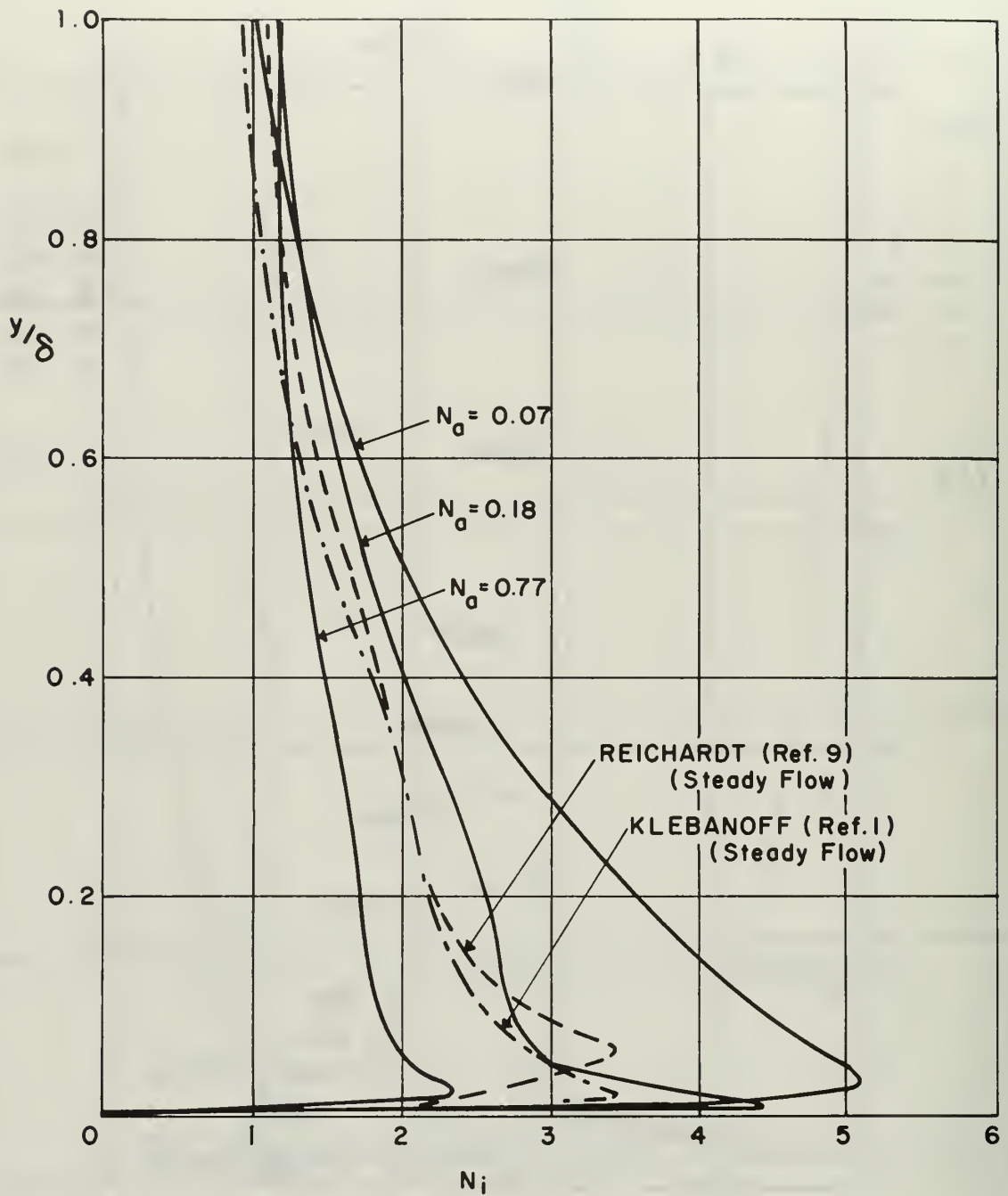
FIGURE 14 COMPARISON OF TURBULENT INTENSITY DISTRIBUTIONS VARIOUS FLUCTUATION AMPLITUDES AND STEADY FLOW RESULTS
