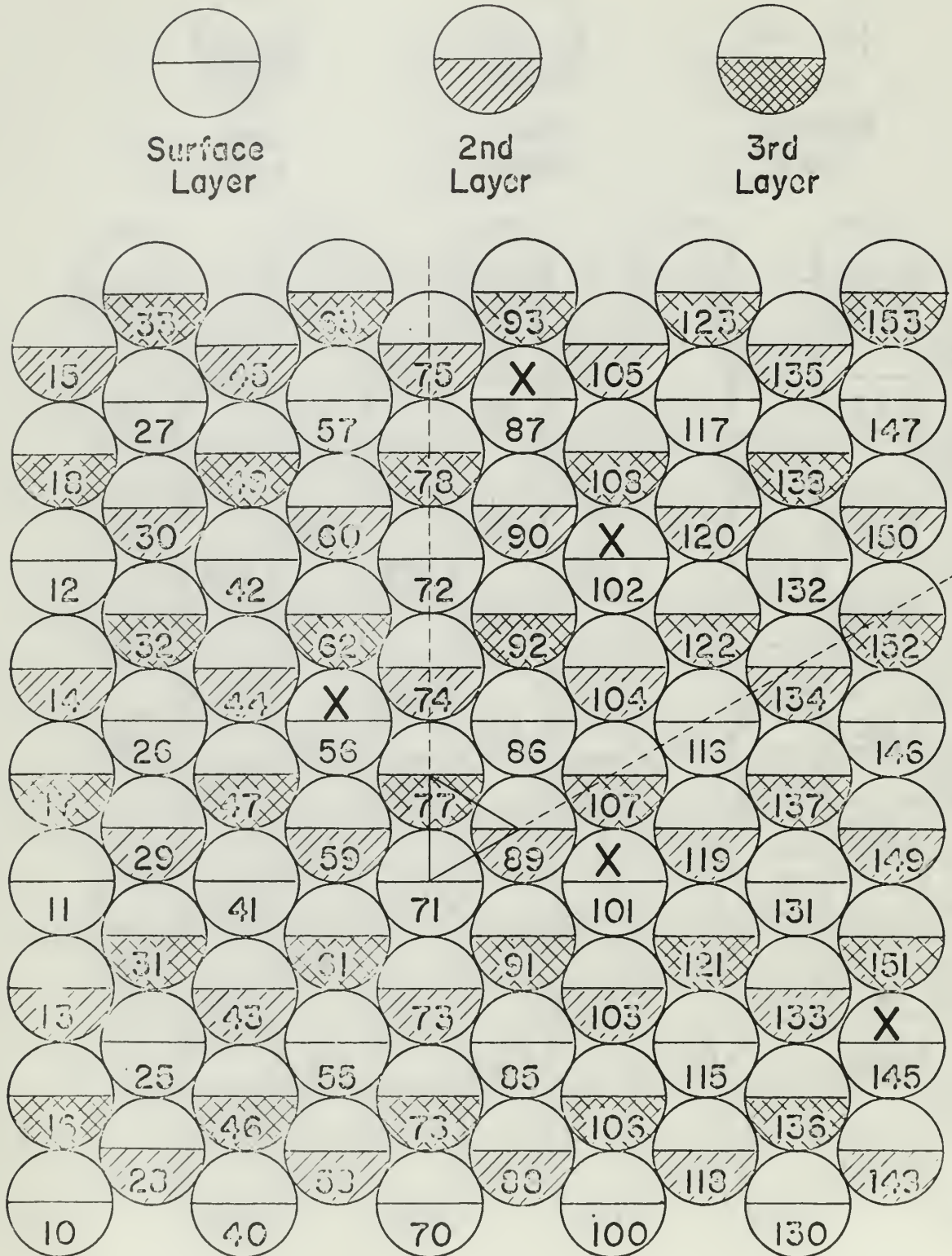
Sputtering frequency-location diagram for (111) surface. 4 keV
