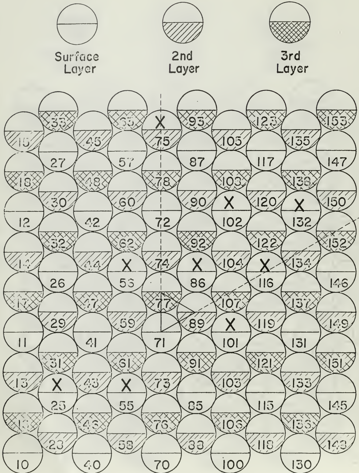
Sputtering frequency-location diagram for (111) surface. 7 keV
