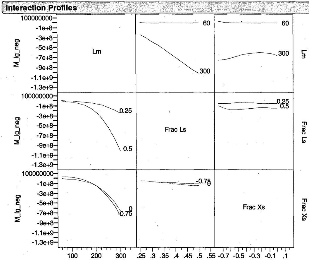
Figure 26 – Longitudinal Wave Side Hull Negative Twisting Independent Variable Interaction
