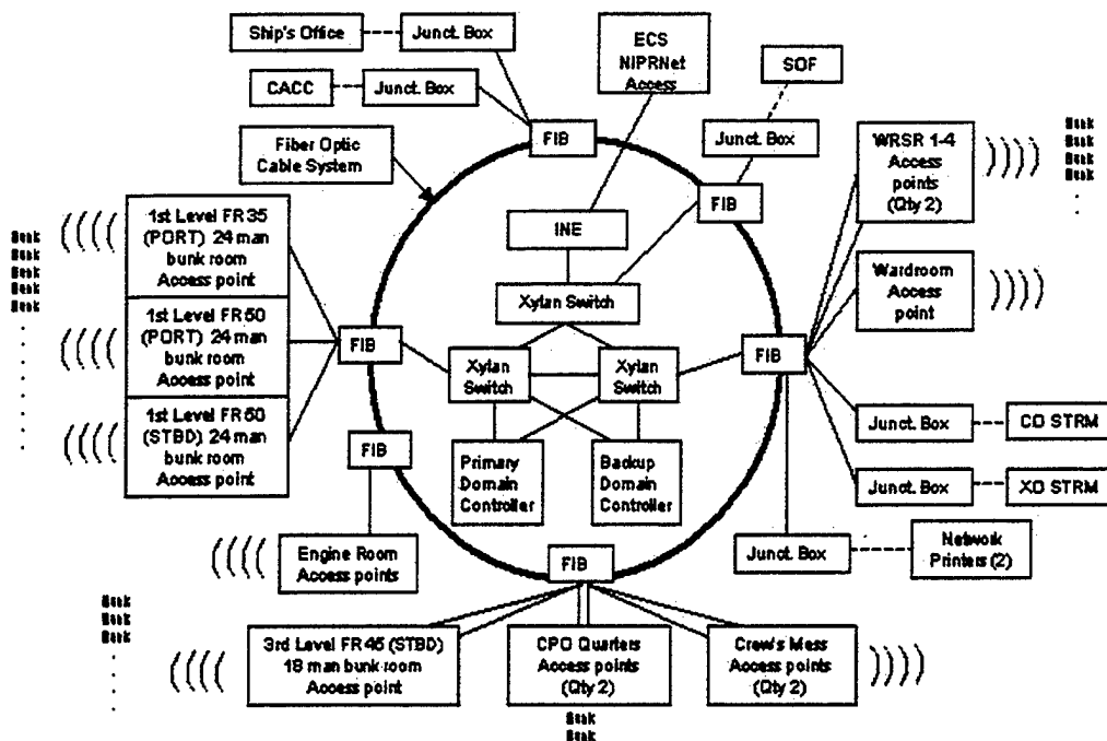
Figure 29 - "Original Design" LAN
