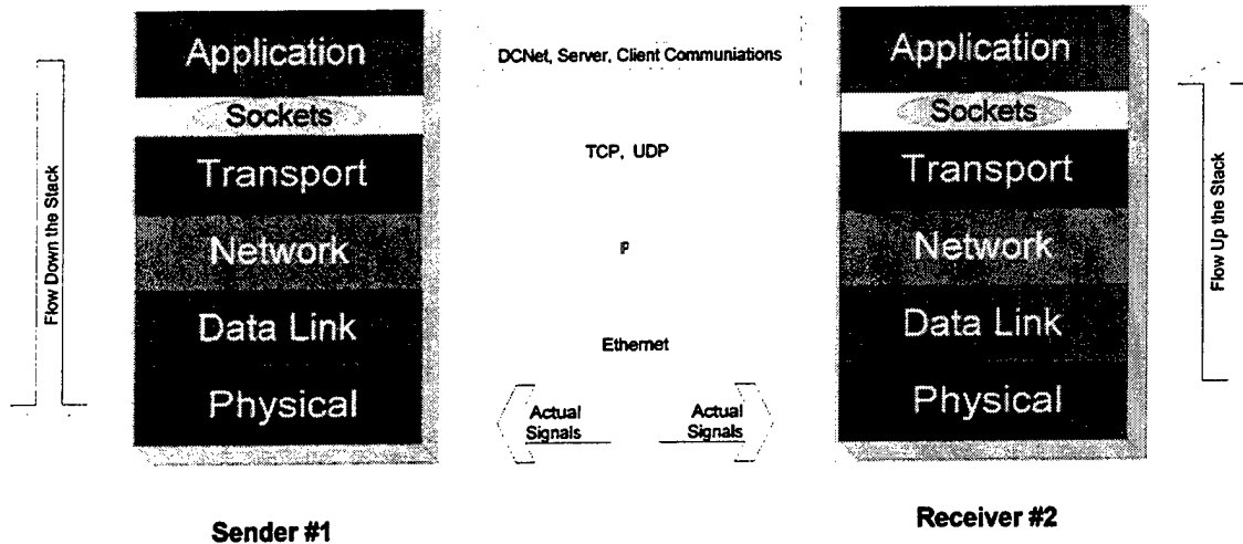
Figure 19 - TCP/IP Model
