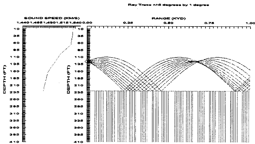
c. Maximum Detection Range (DR) for a 26 ft. Target Depth = 615 yd
