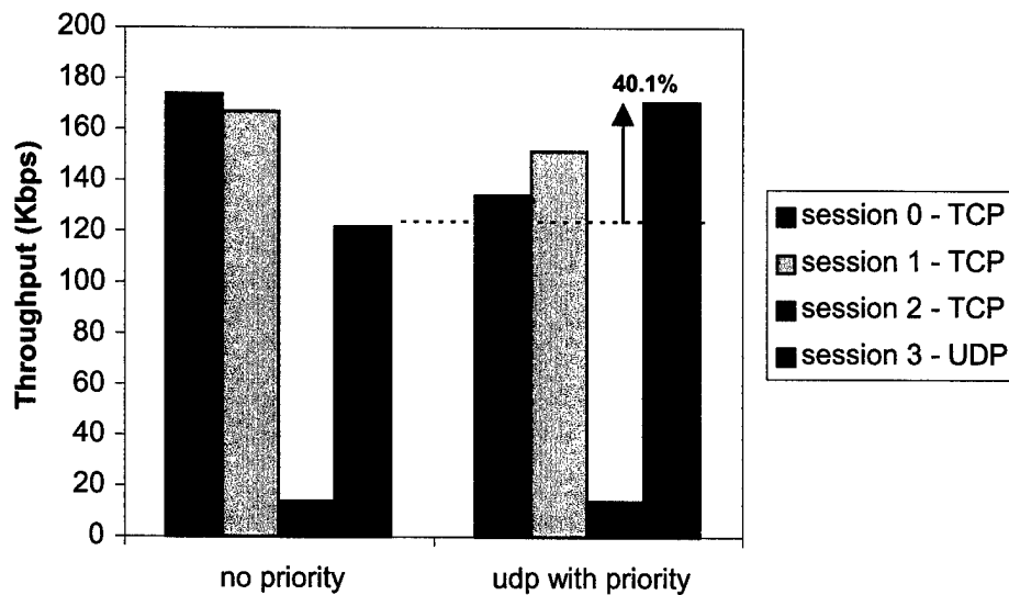
Figure 7.25 CBR/UDP Relative Improvement in the Average Throughput over a 50 km × 50 km, 50 Nodes, and High Mobility Scenario.
