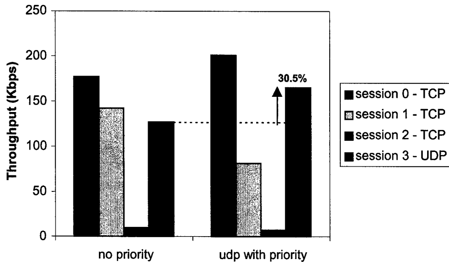
Figure 7.24 CBR/UDP Relative Improvement in the Average Throughput over a 40 km \times 40 km, 10 Nodes, and High Mobility Scenario.
