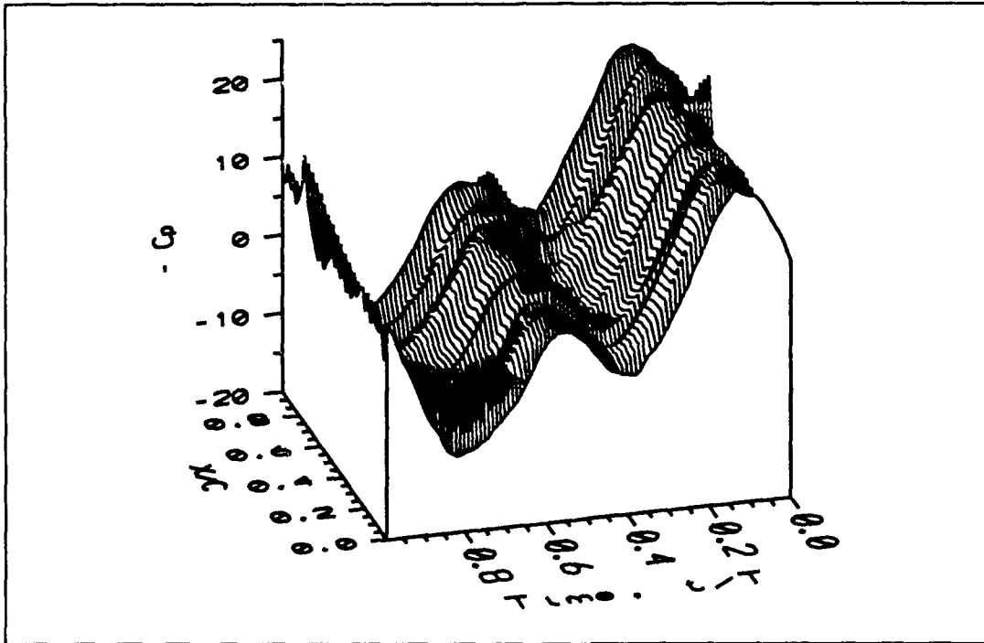
Figure 42. Lower Surface Pressure Coefficient at 35° Angle of Attack in Oscillating Flow.
