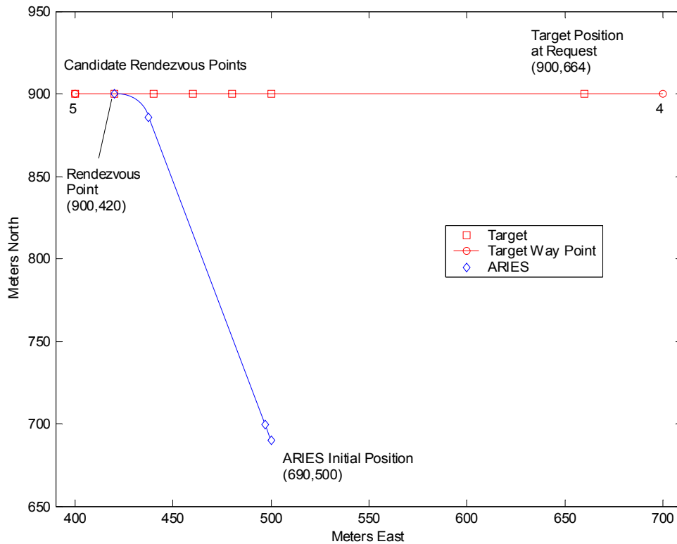
Figure 40. Mission Planning, Energy-Optimal Rendezvous, Laboratory Run
