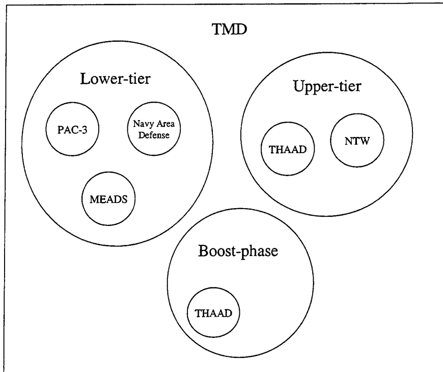
Figure 5. TMD Subcommunity
