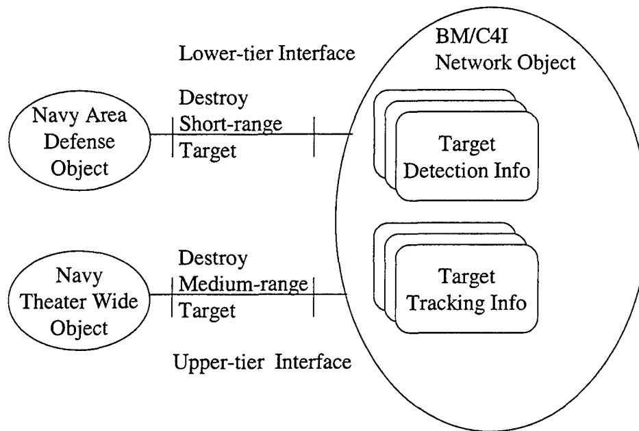
Figure 8. Computational Viewpoint
