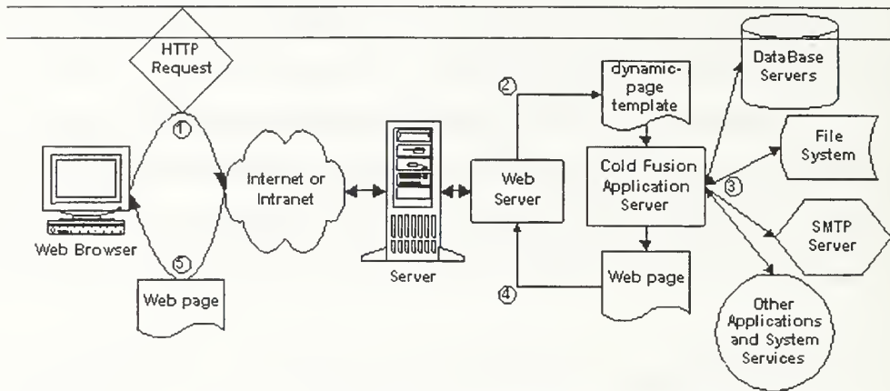
Figure 6. Cold Fusion Application Server
