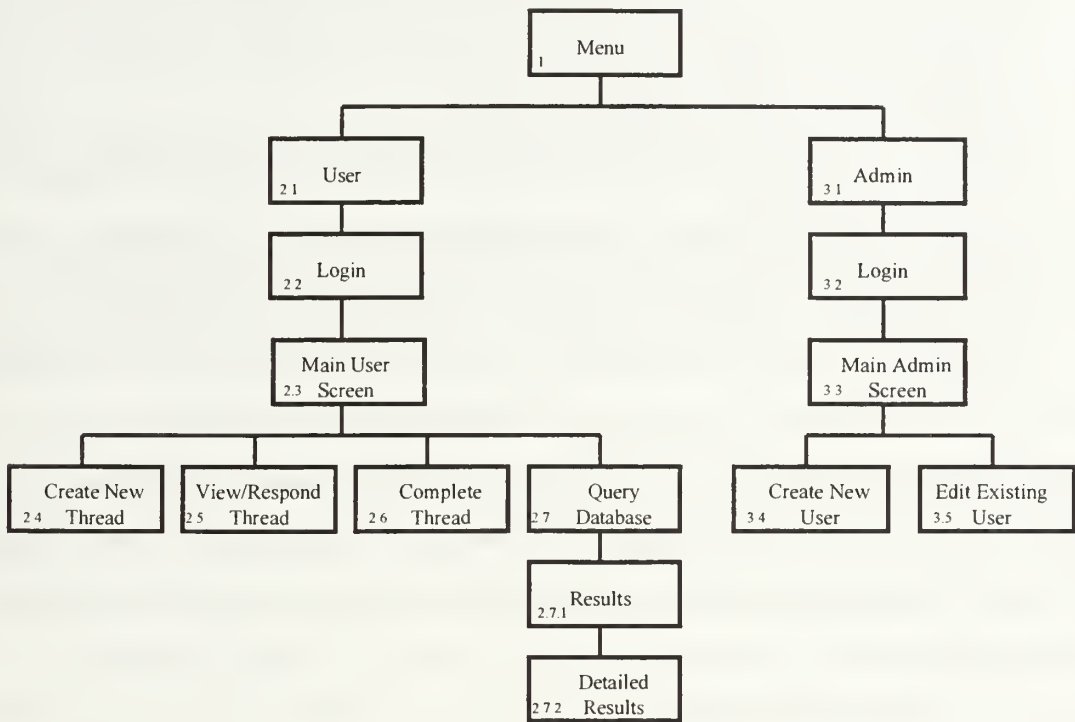
Figure 7. ARBAS-IOM Story-Board Application
