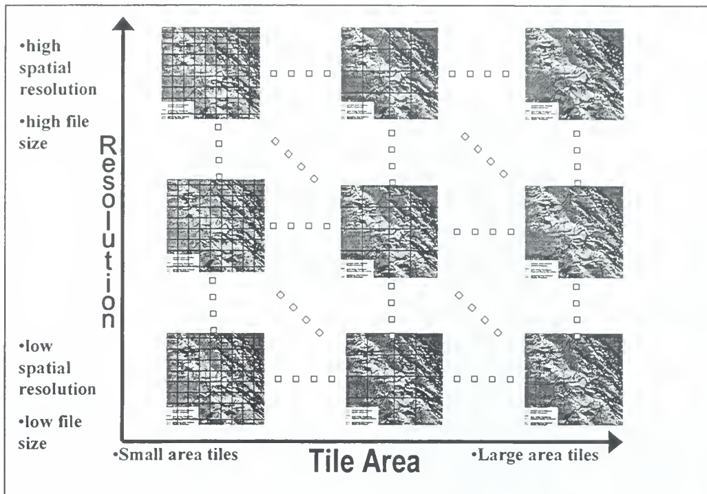
Figure 3.1. Tile Transitions
