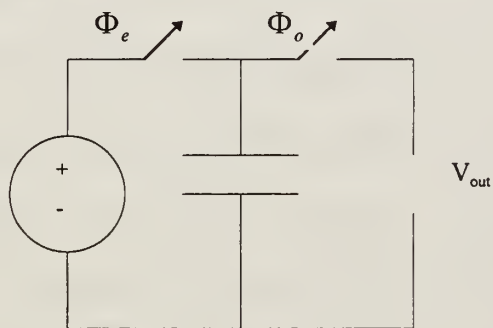
Figure 5.2 Switched Capacitor Network, Allen (1984)
