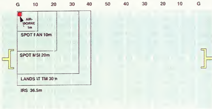
Figure 2.9. Spectral Resolution of Common Sensors (From MUG, 1995)
