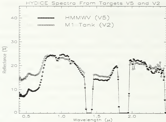
Figure 5.10. Mean Spectra From Targets V5 and V2
