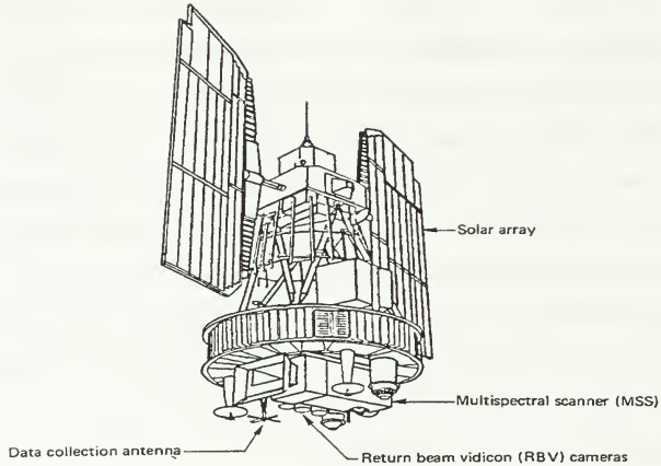
Figure 2.11. LANDSAT MSS (From LANDSAT Advertisement, 1985)
