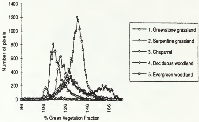
Figure 2.17. Green Vegetation Fractions for June, 1992 (From Ustin et al., 1994)
