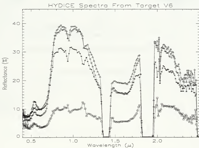
Figure 5.5. Scene-Derived Spectra From V6 (HMMWV)
