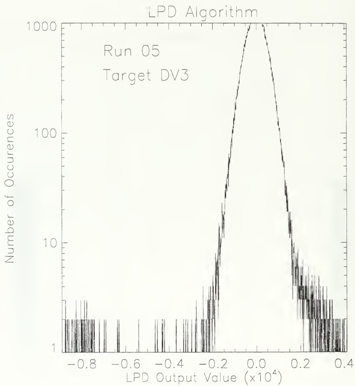
Figure 5.20. LPD Data Distribution Using DV3 Target Spectra
