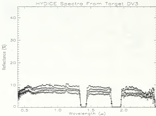
Figure 5.7. Scene-Derived Spectra From DV3 (Decoy)
