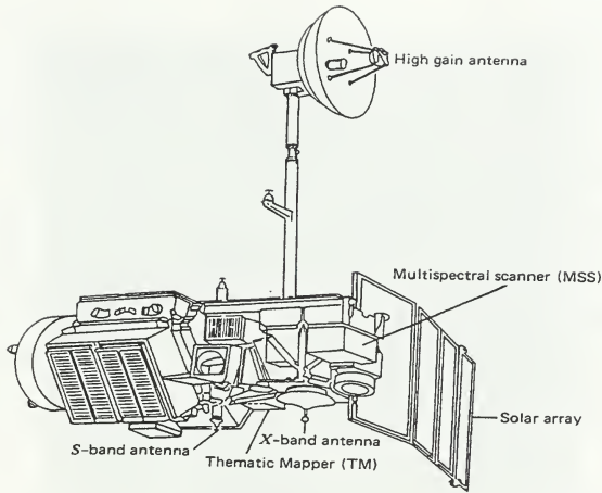
Figure 2.12. LANDSAT TM (From LANDSAT Advertisement, 1985)
