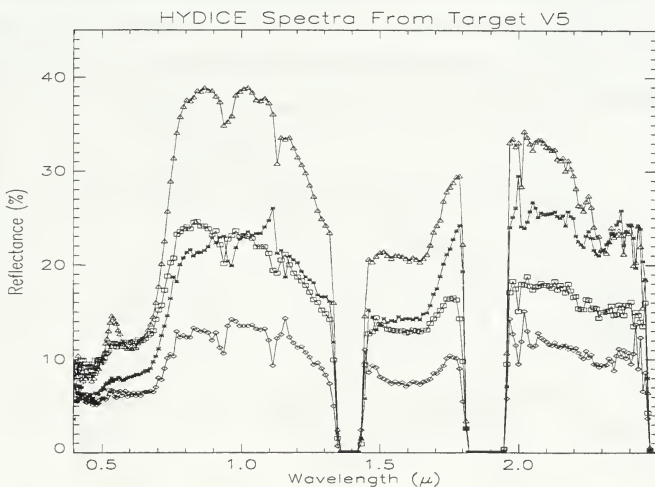
Figure 5.3. Scene-Derived Spectra From V5 (HMMWV)
