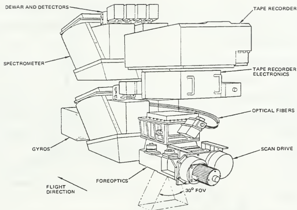
Figure 2.16. AVIRIS Sensor (From Vane, 1987)
