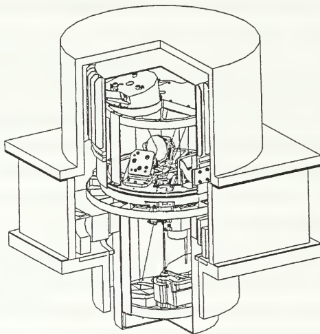
Figure 4.6. HYDICE Instrument (From Anderson, 1995)
