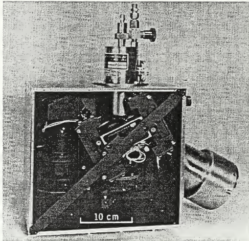
Figure 2.13. Airborne Imaging Spectrometer (From Vane et al., 1988)
