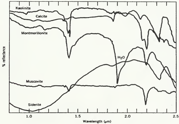
Figure 2.6. Mineral Surface Reflectance (From Rinker, 1990)
