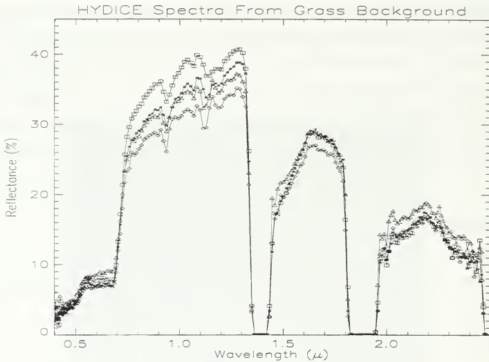
Figure 5.2. Scene-Derived Spectra From Natural Grass Background
