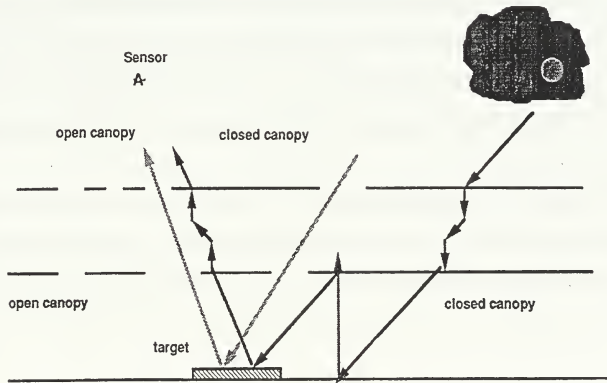
Figure 4.5. Canopy Geometry for Concealed Targets (From Anderson, 1995)
