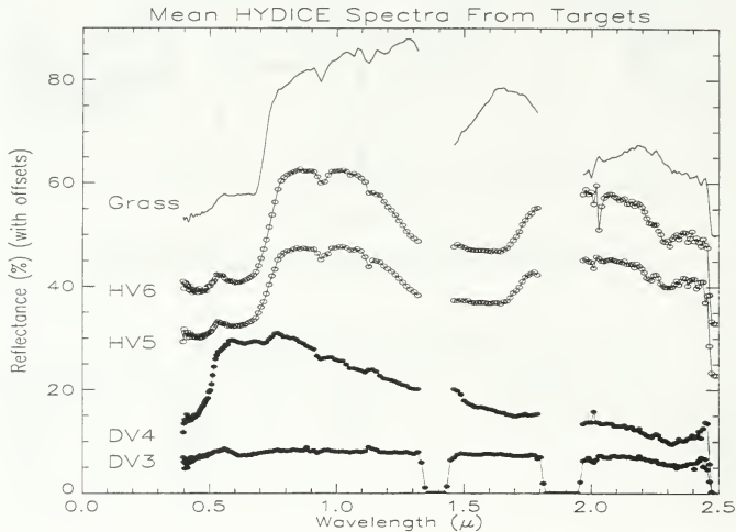
Figure 5.9. Mean Spectra From Targets of Interest
