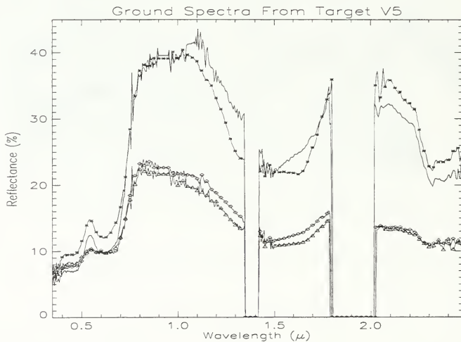
Figure 5.4. Ground-Truth-Derived Spectra From V5 (HMMWV)
