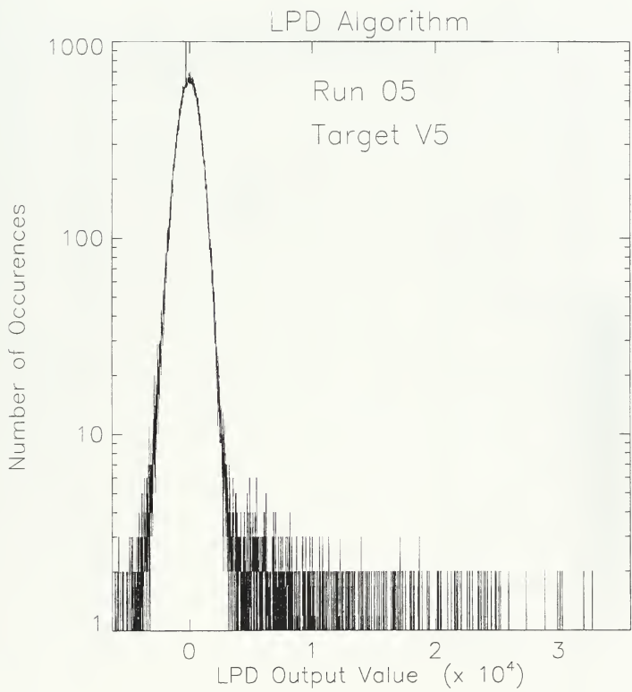
Figure 5.15. LPD Data Distribution Using V5 Target Spectra
