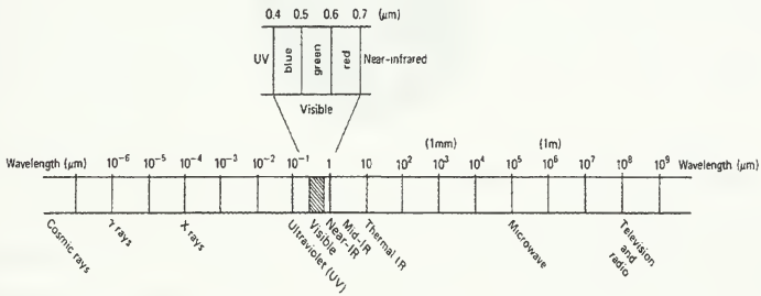
Figure 2.2. Electromagnetic Spectrum
