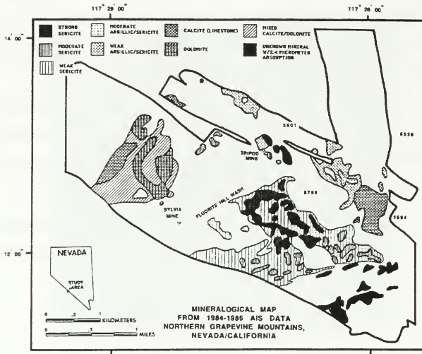
Figure 2.15. Mineralogical Map of Northern Grapevine Mountains (From Kruse, 1987)
