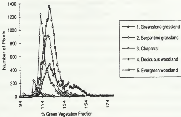
Figure 2.19. Green Vegetation Fractions for October, 1992 (From Ustin et al., 1994)
