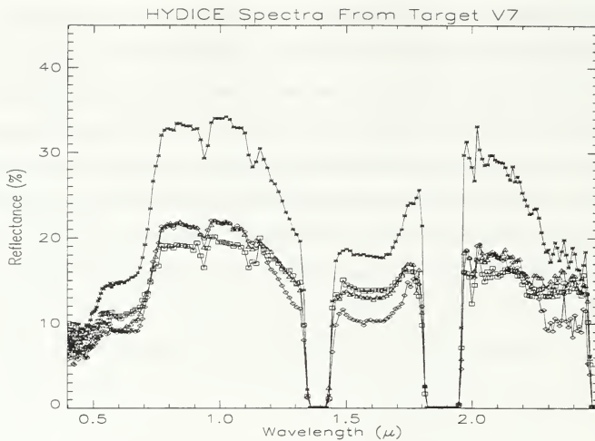
Figure 5.6. Scene-Derived Spectra From V7 (HMMWV)
