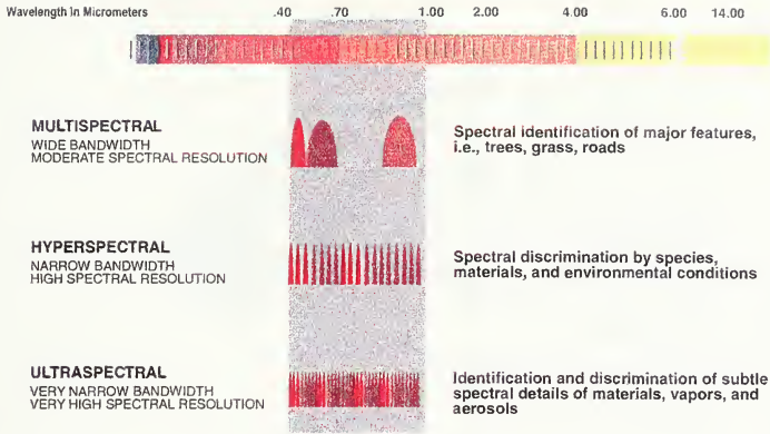
Figure 2.4. Spectral Imaging Types (From MUG, 1995)
