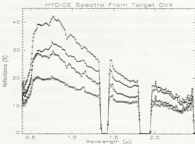
Figure 5.8. Scene-Derived Spectra From DV4 (Decoy)
