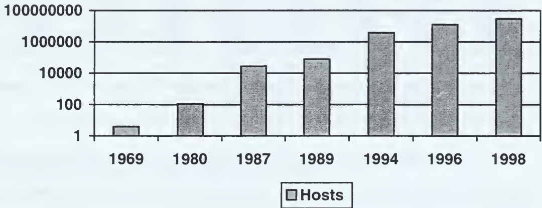
Figure 2: Historical growth of Internet hosts (logarithm scale)
