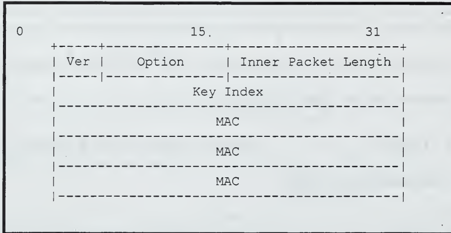
Figure 31. Authentication Trailer format
