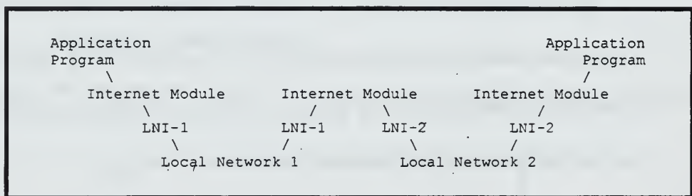
Figure 39. Transmission path
