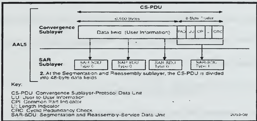
Figure 8. Cell preparation From (Cabletron 1997)
