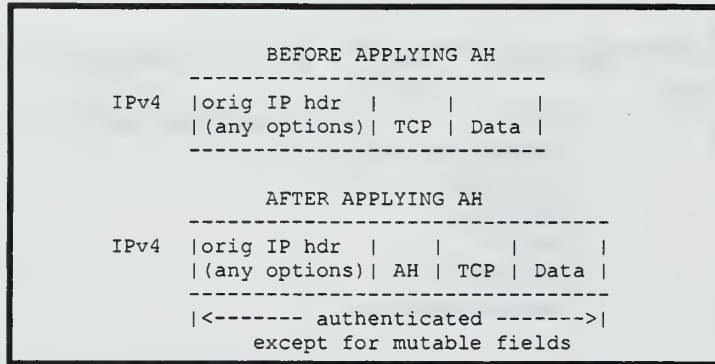
Figure 18. IPv4 before & after AH applied From (Kent and Atkinson 1998)
