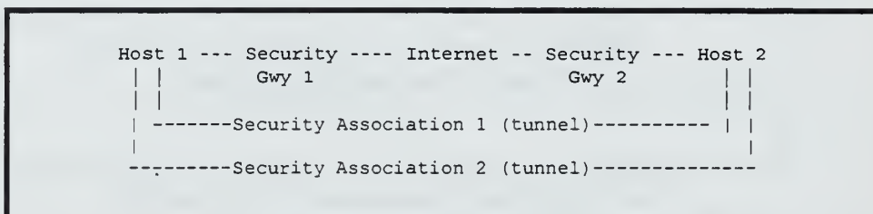
Figure 14. Same SA endpoints From (Kent and Atkinson 1998)
