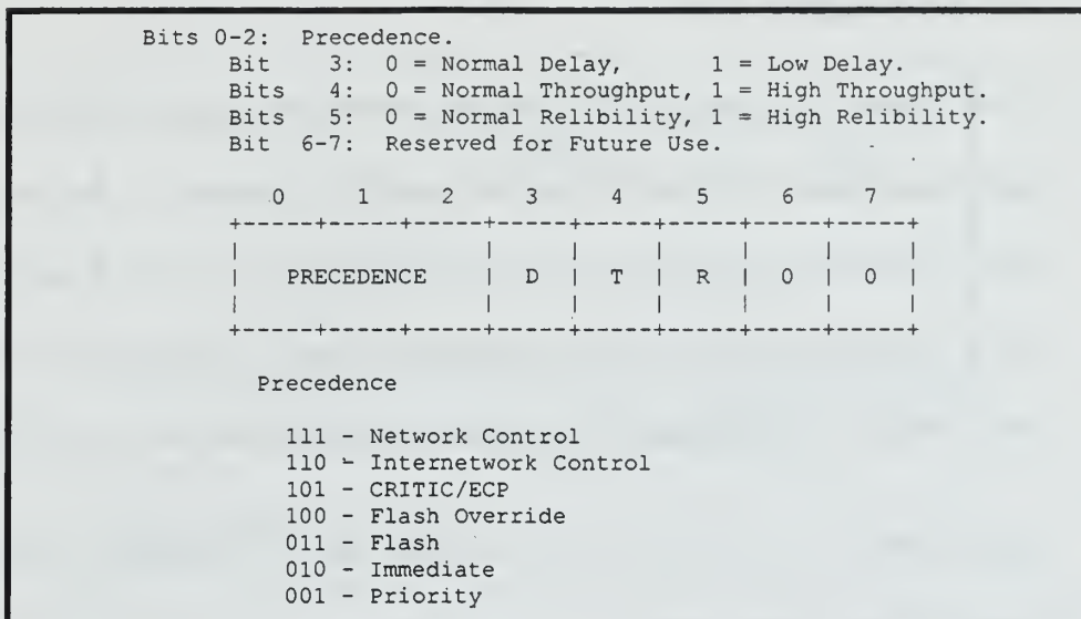
Figure 42. Type-of-Service
