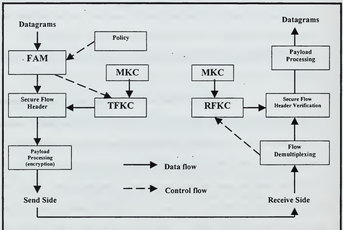
Figure 27. FBS protocol architecture and Operation From (Mitra and Woo 1997)
