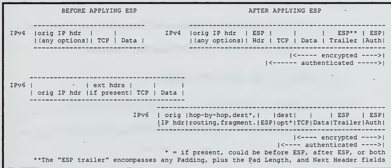
Figure 22. ESP header transport mode application to IP packet From (Kent and Atkinson 1998)
