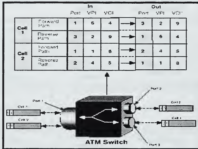
Figure 5. Switching table and cell routing From (Cabletron 1997)
