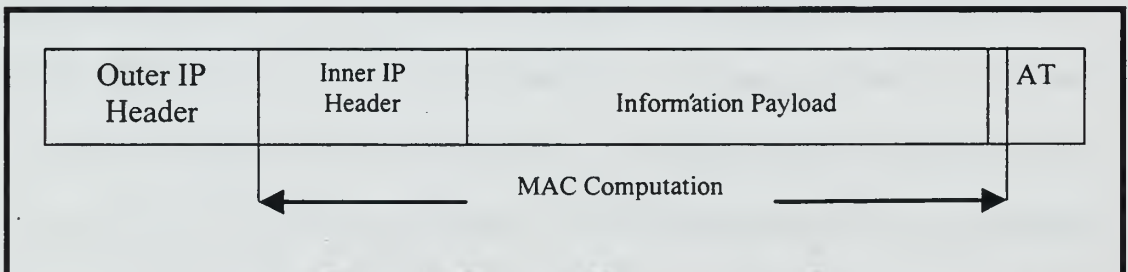
Figure 32. Tunneled IP packet with AT
