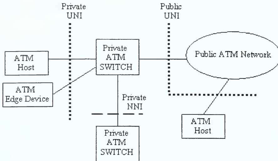
Figure 2.2 ATM Interfaces After Ref. [7]:p. 148
