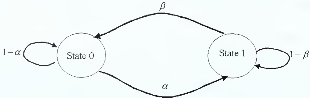
Figure 3.4 Two-State Cell Injection MMPP Model.
