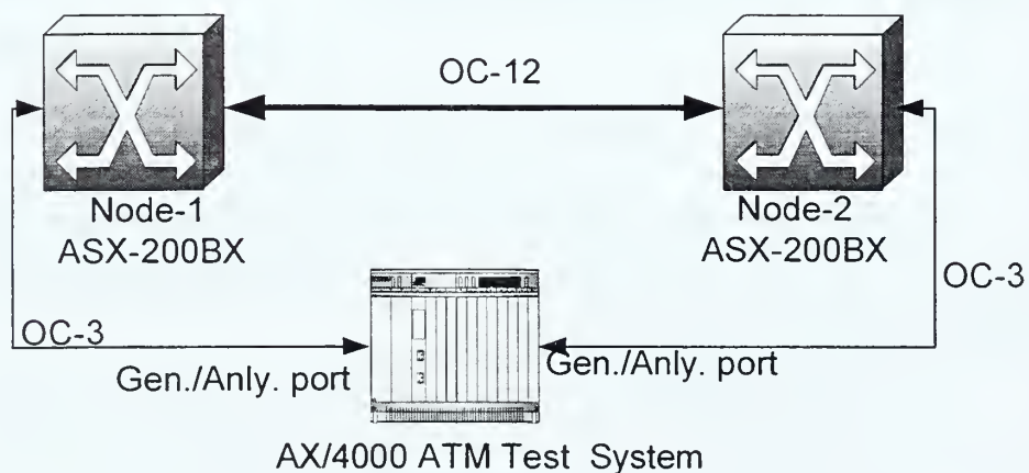
Figure 4.3 Physical Layout.
