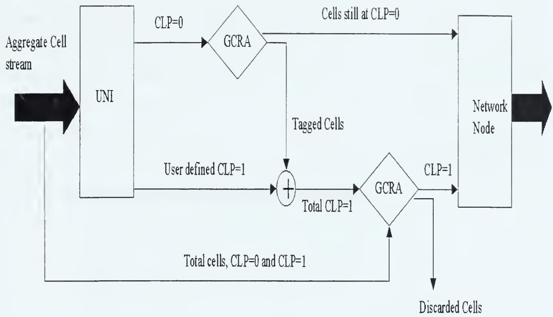
Figure 2.11 Dual Leaky Bucket GCRA [10].
