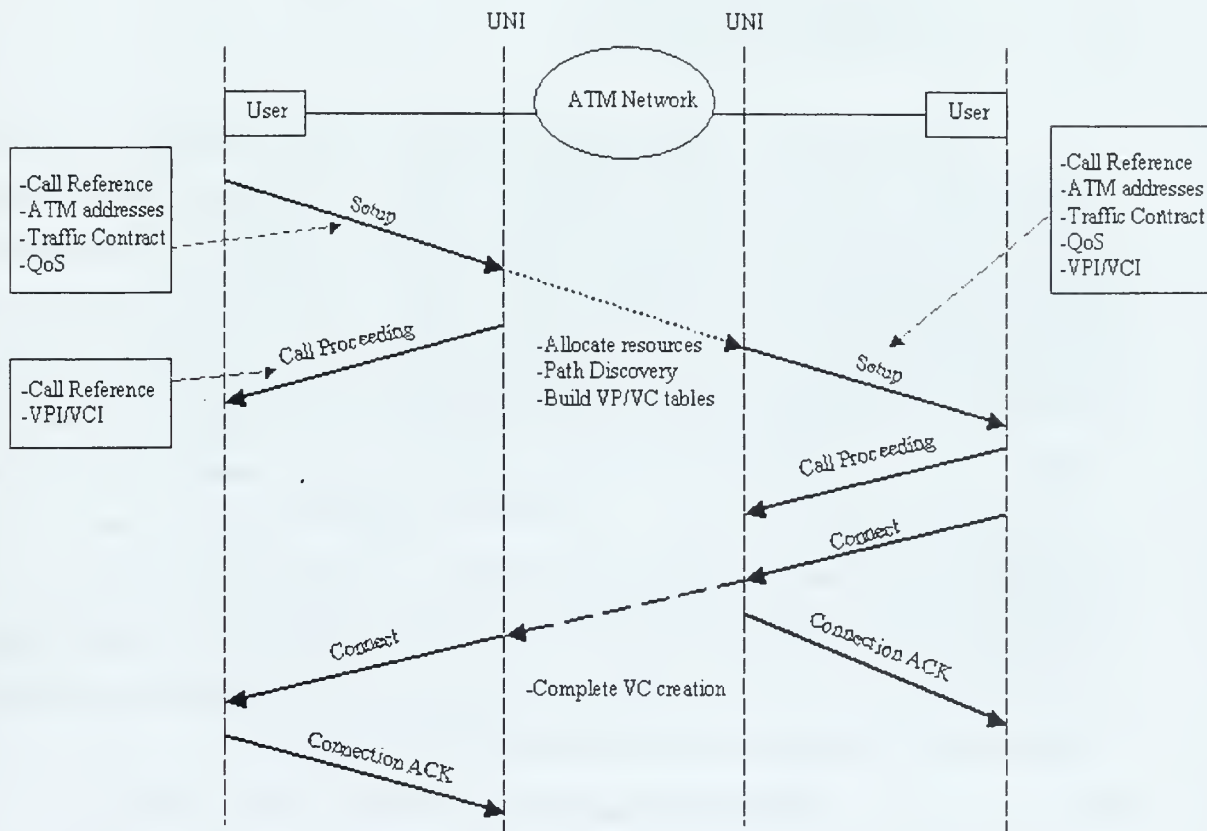
Figure 2.8 Connection Setup [10].
