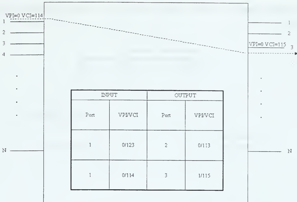
Figure 2.5 ATM Switch. After Ref. [9]:p. 182
