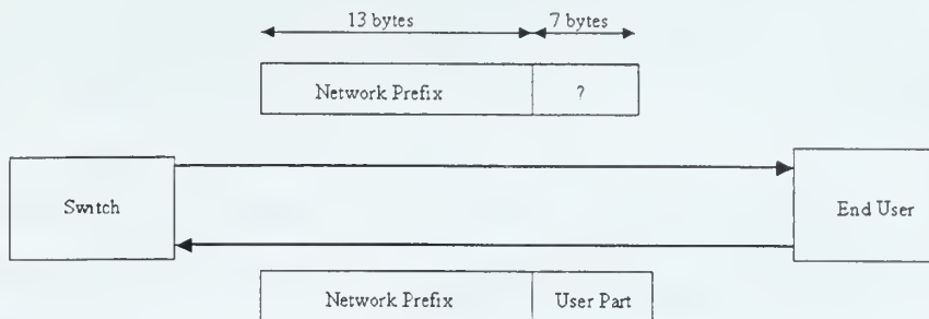
Figure 2.7 Address Registrations.
