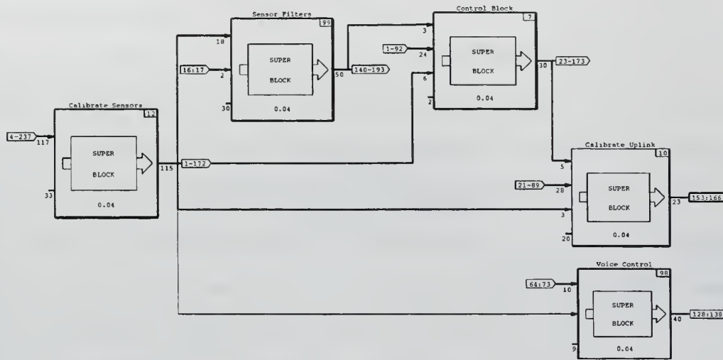
Figure 16. Flight Management SuperBlock
