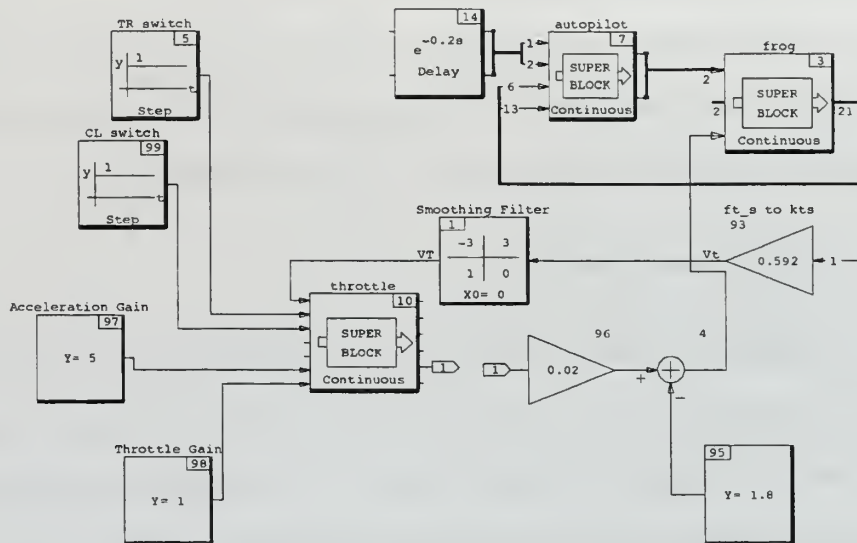
Figure 21. Control Loop
