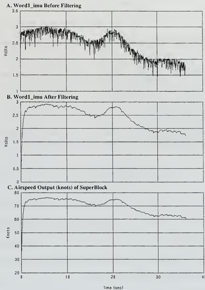
Figure 26. Airspeed Filtering
