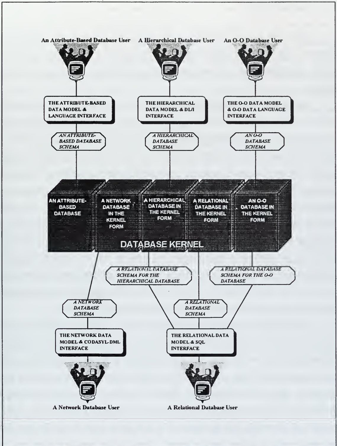
Figure 1. M 2 DBMS Cross-Model Accessing Capability.
