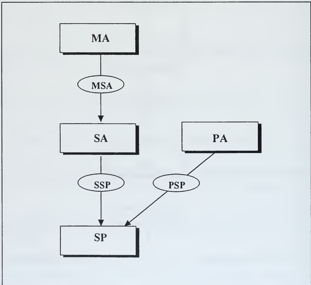
Figure 46. PARTS5 Database.
