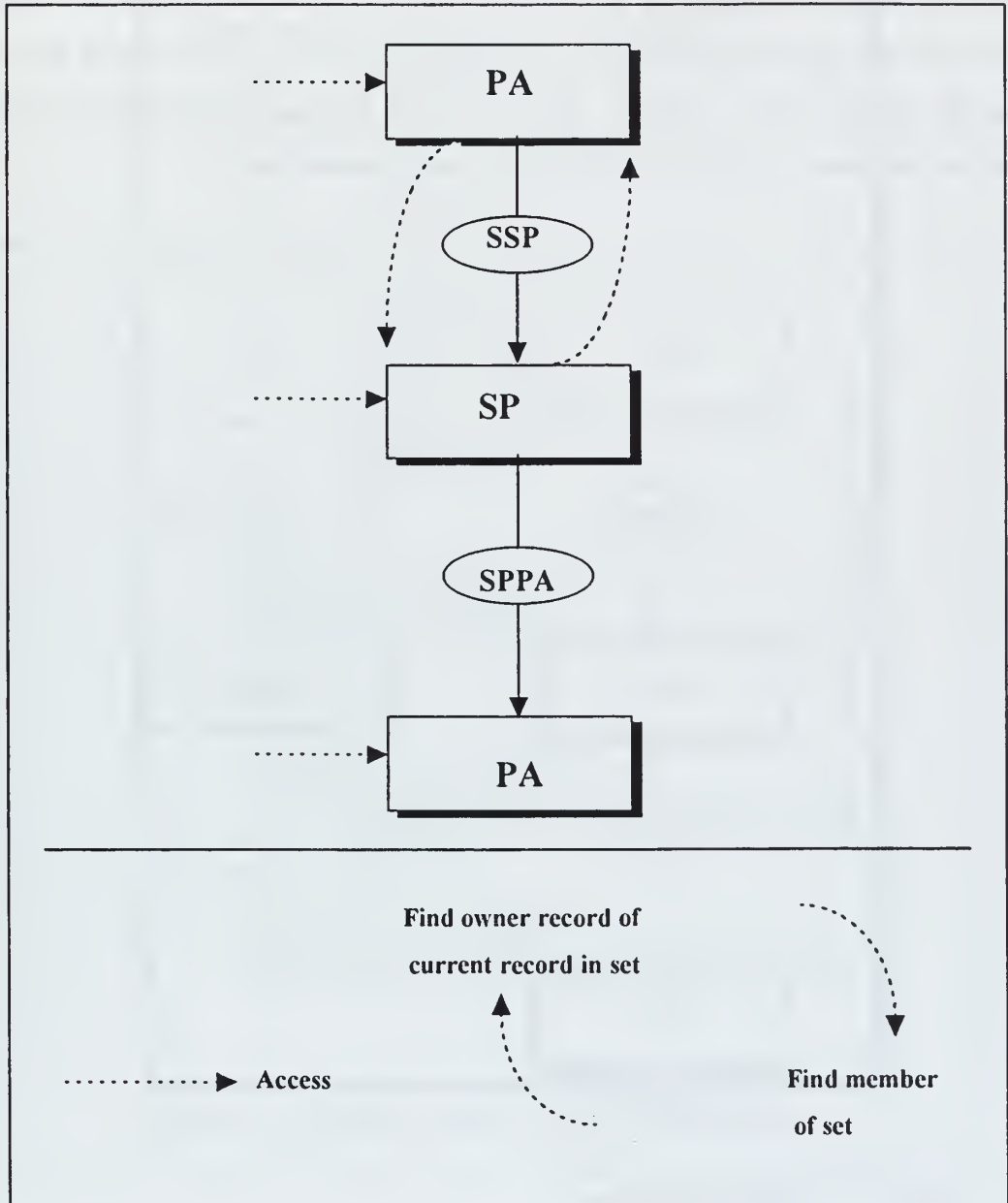
Figure 45. PARTS4 Query Access and Navigation.
