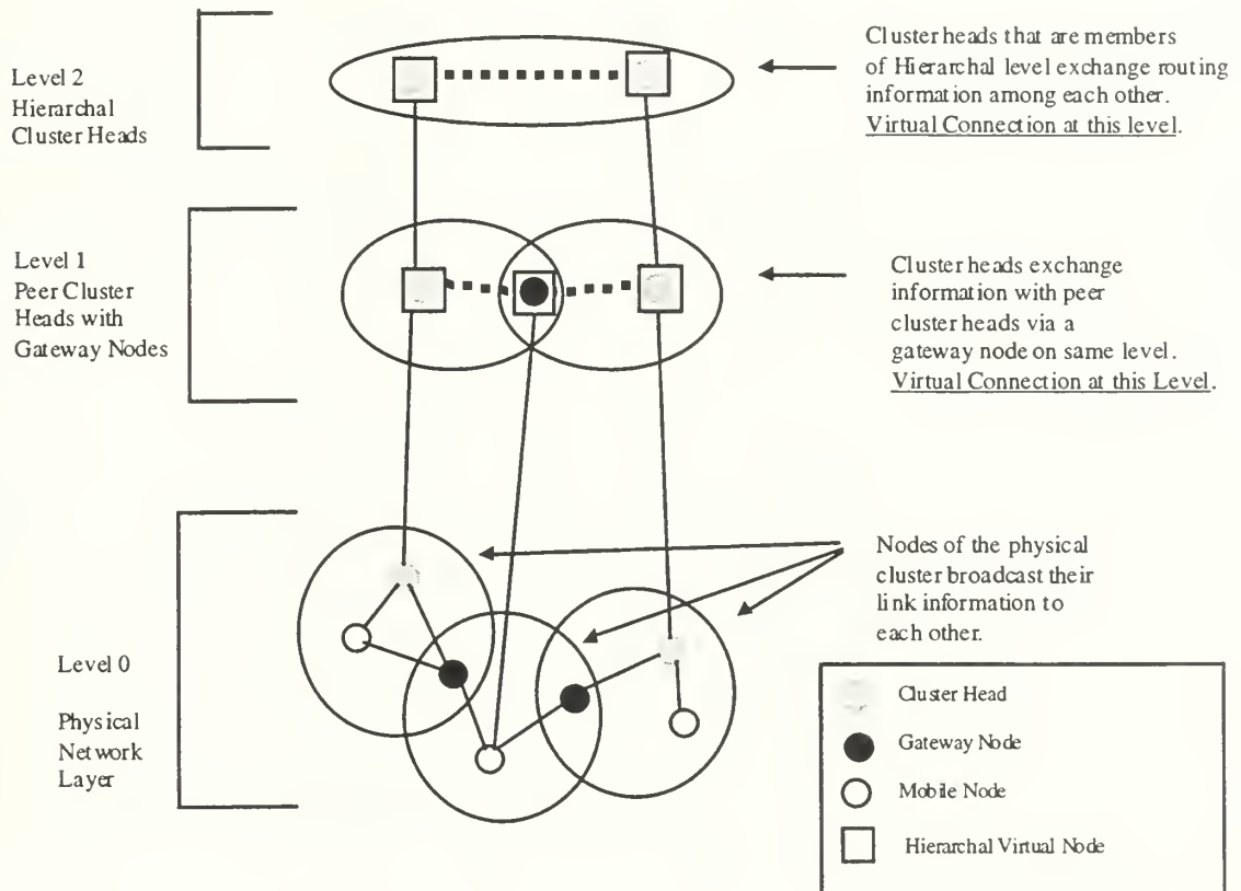
Figure 4. An Example of Clustering in HSR (After Ref. [7]).
