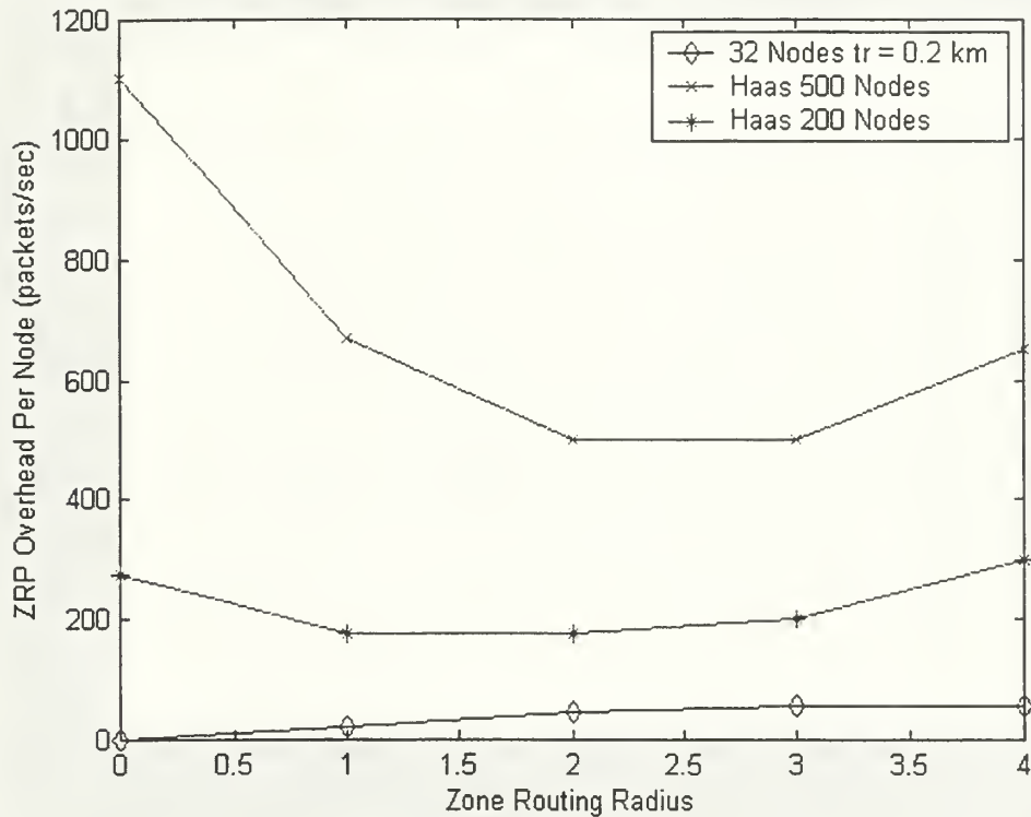
Figure 23. ZPR Traffic Per Node (After Ref. [4]).
