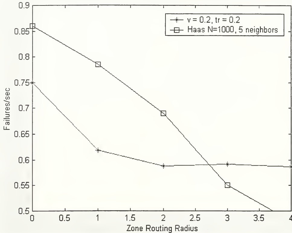
Figure 25. Link Failure Percentage With Increasing Zone Routing Radius (After Ref. [4]).
