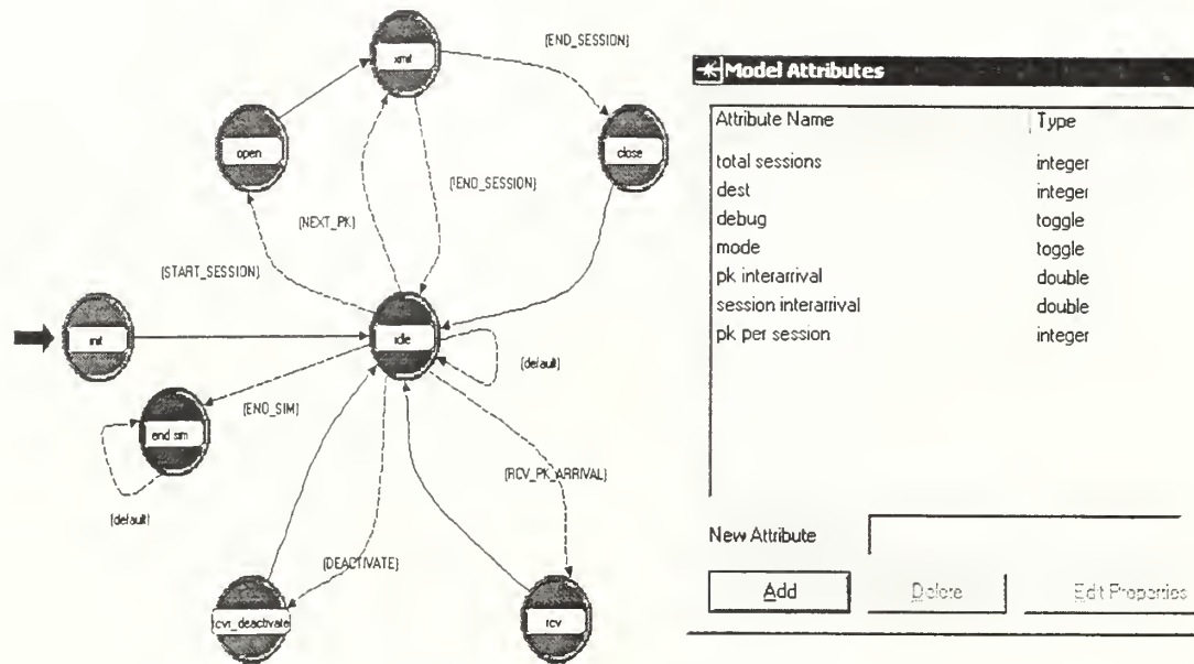
Figure 17. APP Process Model and Attribute Window.
