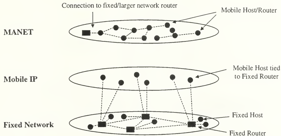
Figure 1. MANET Layer In Perspective (After Ref. [2]).
