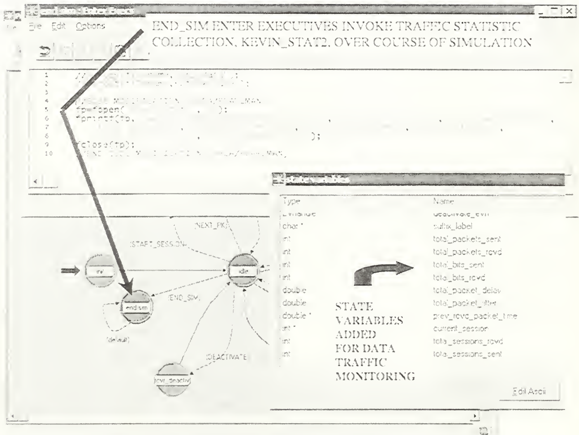
Figure 19. Example Of END_SIM Statistical Collection.
