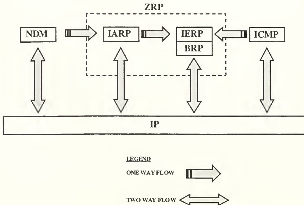
Figure 7. ZRP Architecture (After Ref. [11]).
