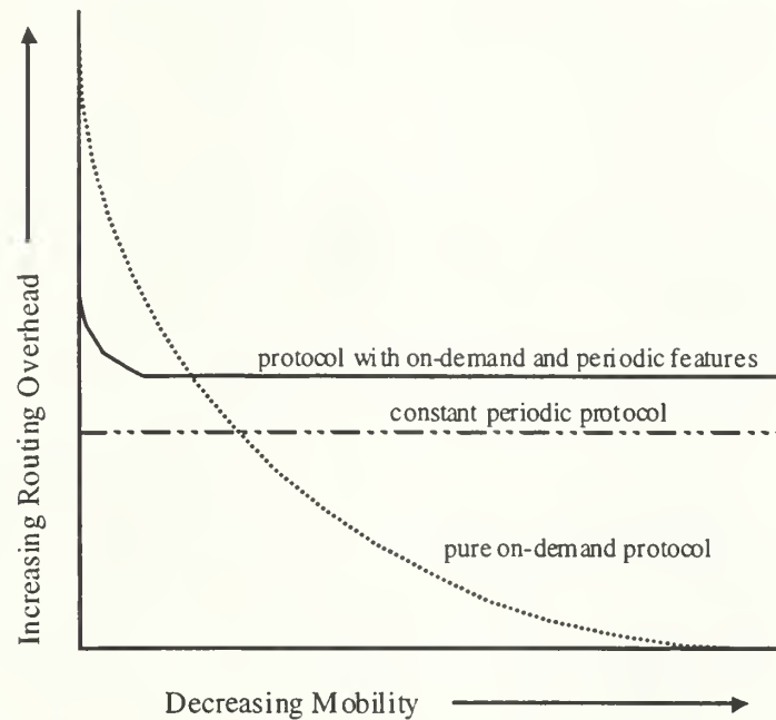
Figure 3. Behavior of On-demand and Periodic Mechanisms (From Ref. [6]).
