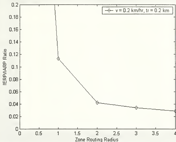
Figure 28. IERP/IARP Routing Zone Optimization.
