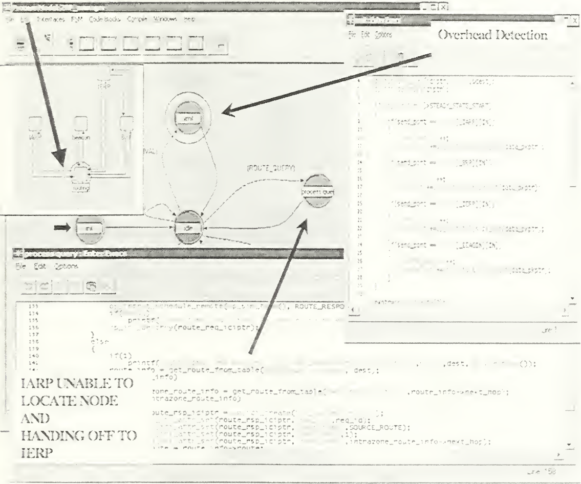
Figure 13. Depiction of Routing Node Object Within ZRP_Manager.
