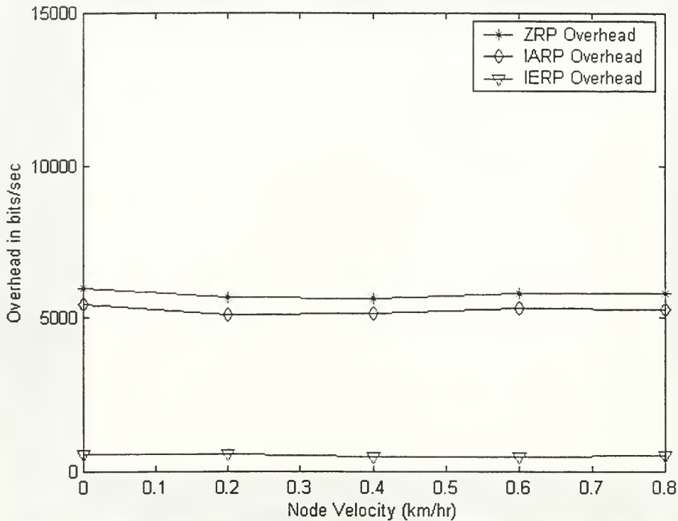
Figure 24. ZRP Overhead With Changing Velocity.
