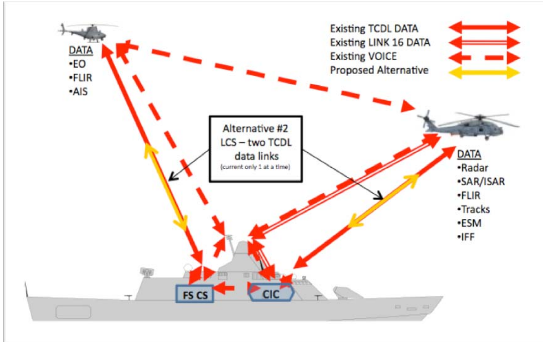
Figure 27: Alternative-2 Communications Channels
