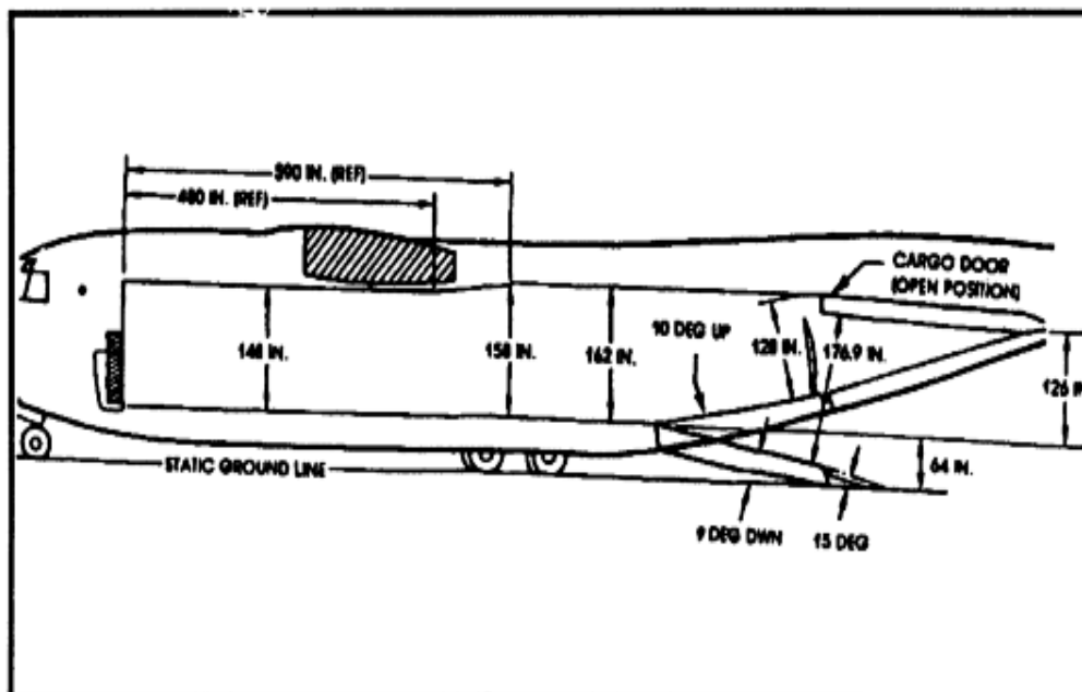
Figure F-6: C-17 Cargo Compartment Height Dimensions. 453
