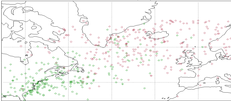
Figure 23. Atlantic basin. Green diamonds denote position of when hurricane force wind extratropical cyclone wind speeds become greater than 43-knot (L) winds speed threshold. Red diamonds denote where storms winds speed become lower than 43 knots.
