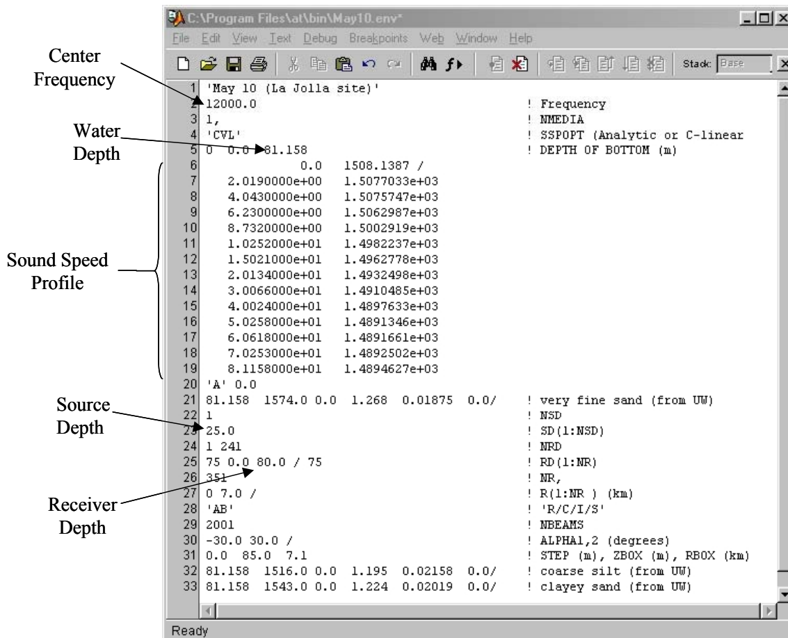
Figure 31. Input file for Bellhop , which describes the channel dimensions and physics.
