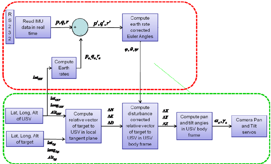
Figure 3. System architecture
