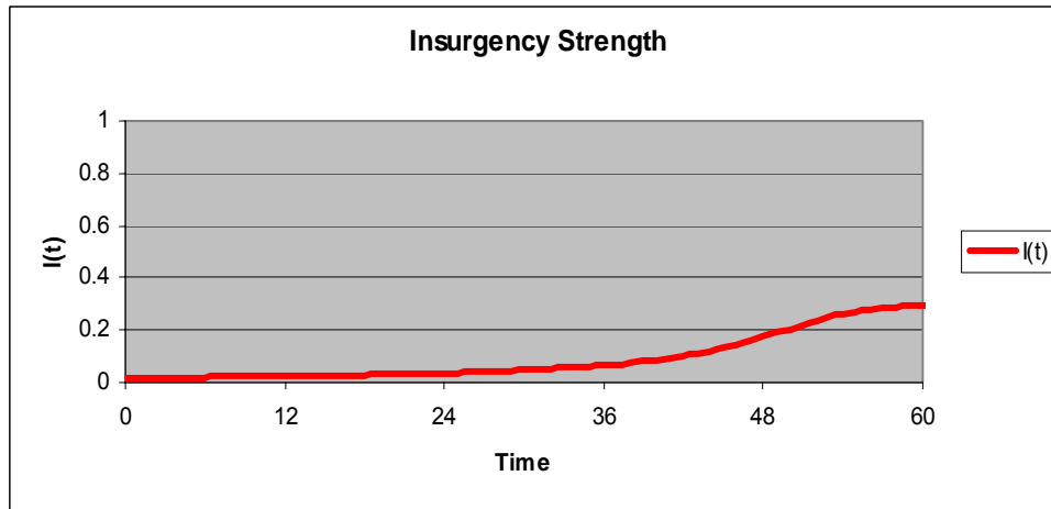
Figure 21. Advanced Model I(t) with \rho_{SC} = A_I + A_{PI} - A_G - A_{PG} for 60 months
