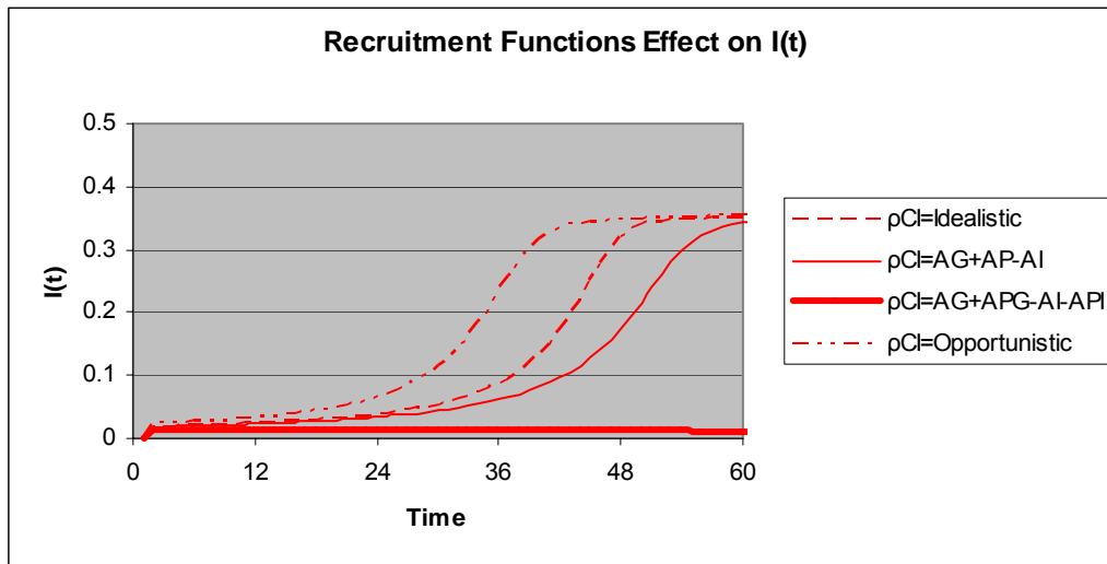
Figure 24. Recruitment Functions Effect On I(t) in Advanced Model
